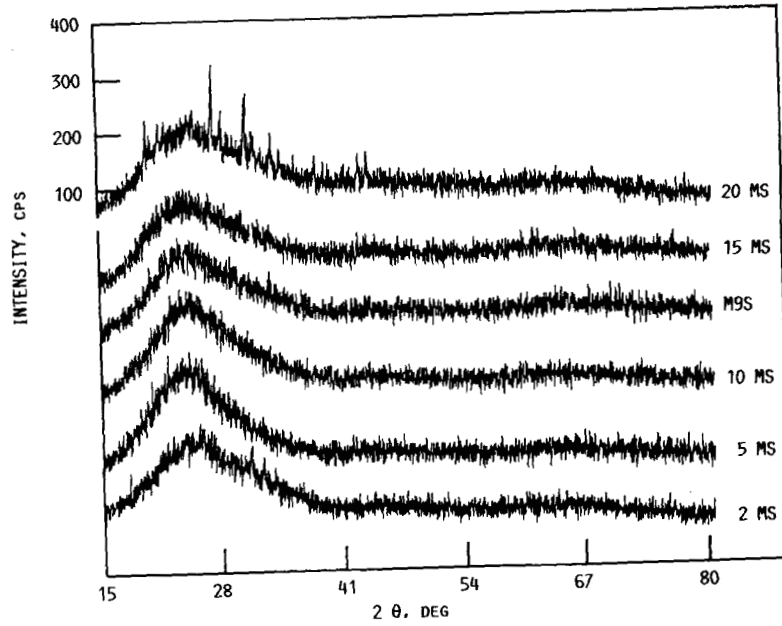
FIG. 12. - X-RAY DIFFRACTION PATTERNS OF MgO-SiO_2 GELS OF VARIOUS COMPOSITIONS DRIED AT 76^\circ C . THE PEAKS IN 20 MS SAMPLE CORRESPOND TO Mg(NO_3)_2 \cdot 6H_2O CRYSTALS.
