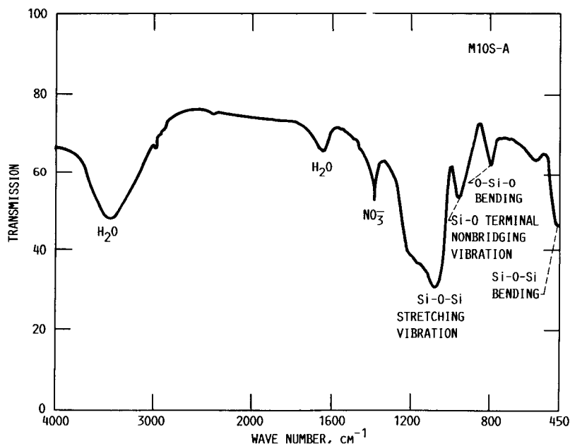
FIG. 9 - INFRARED SPECTRA OF 10MgO-90SiO_2 (MOL%) GEL DRIED AT 72\text{ }^\circ\text{C} FOR MORE THAN 6 DAYS; MOLE RATIO OF WATER:TEOS = 5.6.
