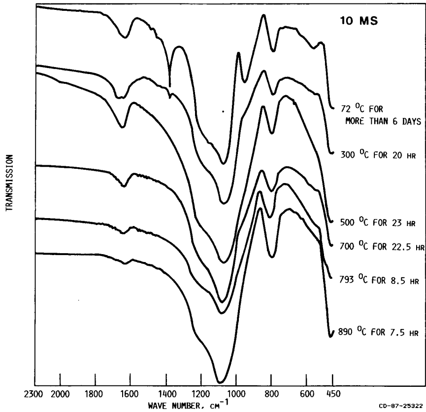
FIG. 10. - INFRARED SPECTRA OF 10MgO-90SiO 2 (MOL %) GEL AFTER FIRING AT VARIOUS TEMPERATURES. THE HEAT TREATMENTS ARE CUMULATIVE AT SUBSEQUENT TEMPERATURES.
