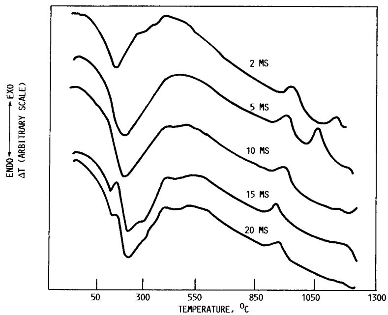
FIG. 8. - DTA CURVES OF MgO-SiO_2 GELS OF VARIOUS COMPOSITIONS DRIED AT 76\text{ }^\circ\text{C} FOR 50 HR; SCAN RATE OF 10\text{ }^\circ\text{C}/\text{MIN} IN FLOWING AIR.
