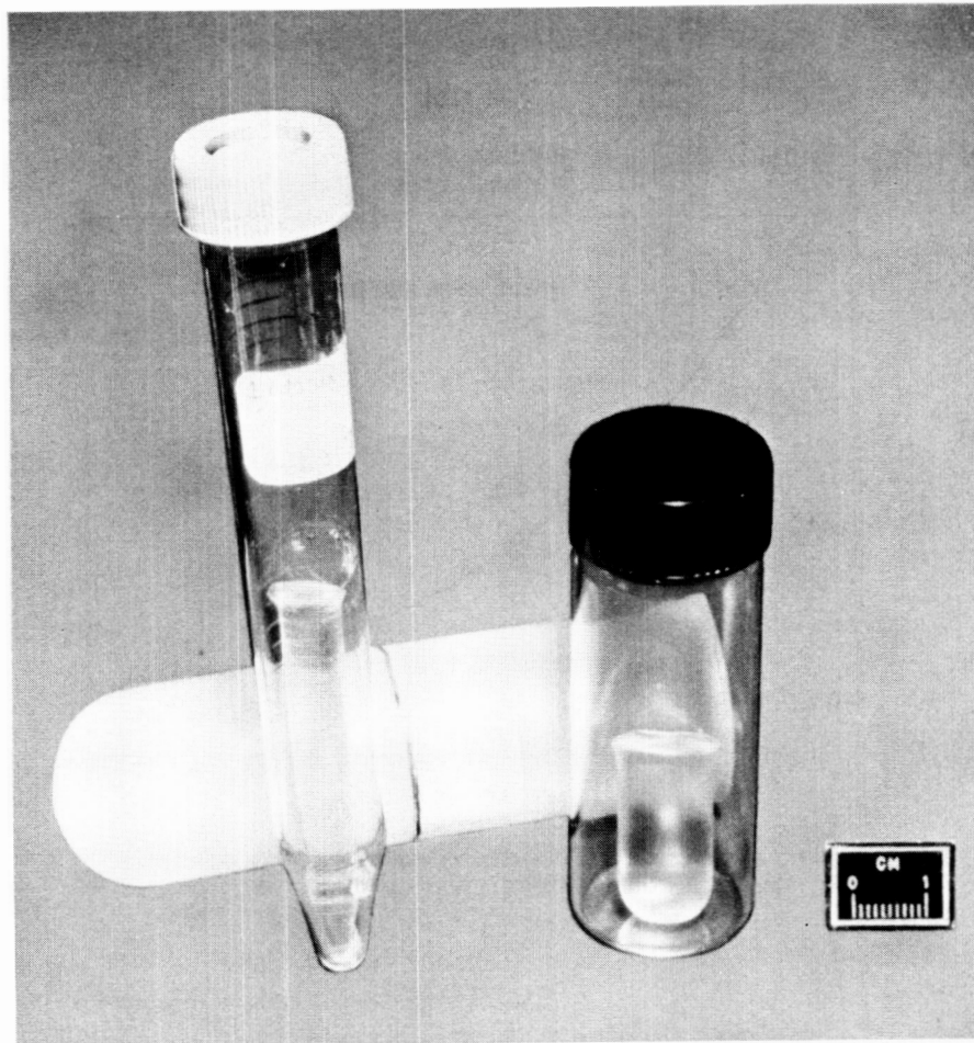
FIG. 4. - MONOLITHIC CYLINDRICAL SAMPLES OF 10MgO-90SiO 2 (MOL %) COMPOSITION PREPARED USING GLYCEROL AS THE DRYING CONTROL CHEMICAL ADDITIVE (DCCA).
