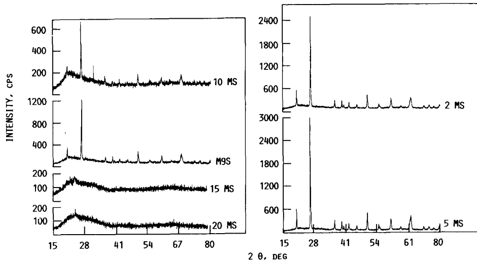
FIG. 15. - POWDER X-RAY DIFFRACTION SCANS OF MgO-SiO 2 GELS OF VARIOUS COMPOSITIONS FIRED AT 1000 °C FOR 2 HR; SHARP DIFFRACTION PEAKS IN 2 MS, 5 MS, 10 MS, AND 1 MS SAMPLES CORRESPOND TO α-QUARTZ CRYSTALS.
