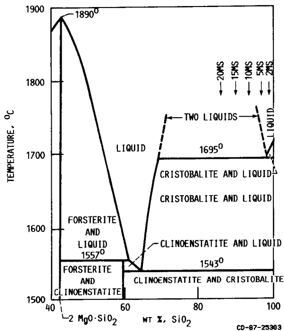
FIG. 1. - PARTIAL PHASE DIAGRAM OF MgO-SiO_2 SYSTEM SHOWING POSITIONS OF THE VARIOUS COMPOSITIONS STUDIED.
