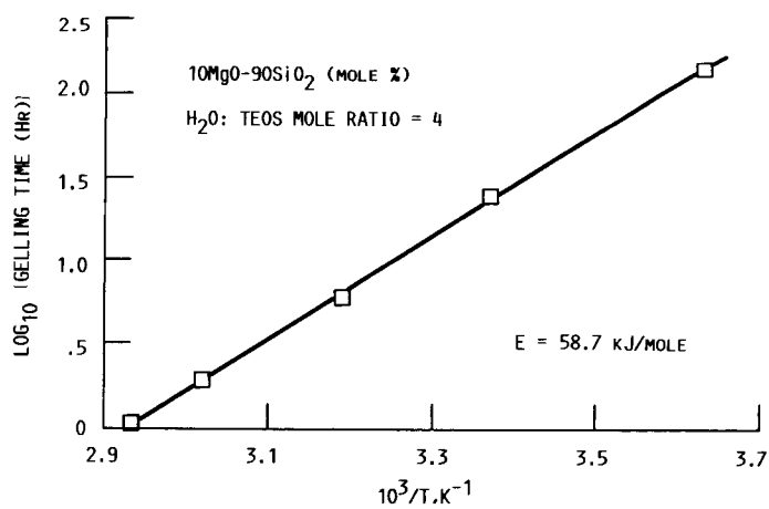
FIG. 17. - ARRHENIUS PLOT SHOWING TEMPERATURE DEPENDENCE OF GELLING TIME OF 10MgO-90SiO 2 (MOL %) COMPOSITION; WATER:TEOS MOLE RATIO = 7.5.
