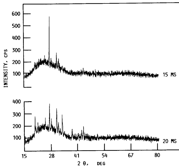
FIG. 3. - POWDER X-RAY DIFFRACTOGRAMS OF 15 MS AND 20 MS GELS DRIED AT ROOM TEMPERATURE. THE PEAKS CORRESPOND TO Mg(NO_3)_2 \cdot 6H_2O CRYSTALS.
