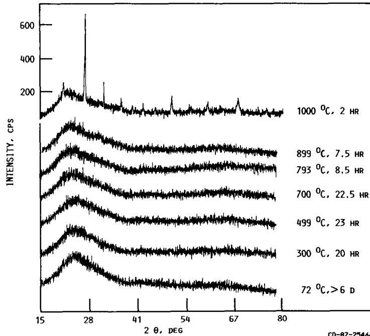
FIG. 14. - X-RAY DIFFRACTOGRAMS OF 10 MgO-90SiO 2 (MOL%) COMPOSITION GEL FIRED AT DIFFERENT TEMPERATURES FOR VARIOUS LENGTHS OF TIME; PEAKS IN THE 1000 °C FIRED SAMPLE CORRESPOND TO α-QUARTZ CRYSTALS.
