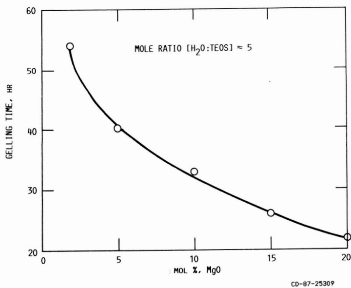
FIG. 5. - EFFECT OF MAGNESIUM OXIDE CONTENT ON TIME OF GEL FORMATION AT ROOM TEMPERATURE FOR THE MgO-SiO 2 SYSTEM; WATER:TEOS MOLE RATIO ~5.
