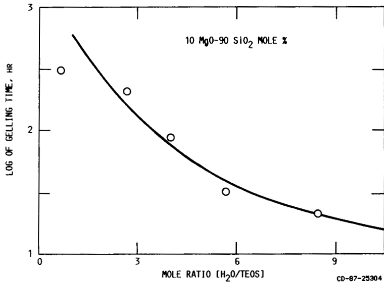
FIG. 6 - INFLUENCE OF WATER:TEOS MOLE RATIO ON TIME OF GELATION OF 10MgO-90SiO 2 (MOL %) COMPOSITION AT ROOM TEMPERATURE.
