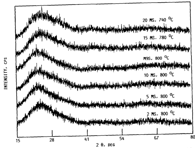
FIG. 13. - X-RAY DIFFRACTION SPECTRA OF MgO-SiO_2 GELS OF VARIOUS COMPOSITIONS HEATED TO DIFFERENT TEMPERATURES IN FLOWING AIR AT 3^\circ C/MIN AND FURNACE COOLED.
