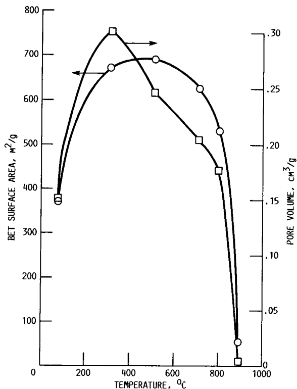
FIG. 16. - VARIATION OF BET SURFACE AREA AND PORE VOLUME WITH FIRING TEMPERATURE OF 10MgO-90SiO 2 (MOL %) GEL COMPOSITION; WATER: TEOS MOLE RATIO = 5.66. THE THERMAL TREATMENTS ARE CUMULATIVE AT SUBSEQUENT TEMPERATURES (SEE TABLE VI FOR DETAILS).
