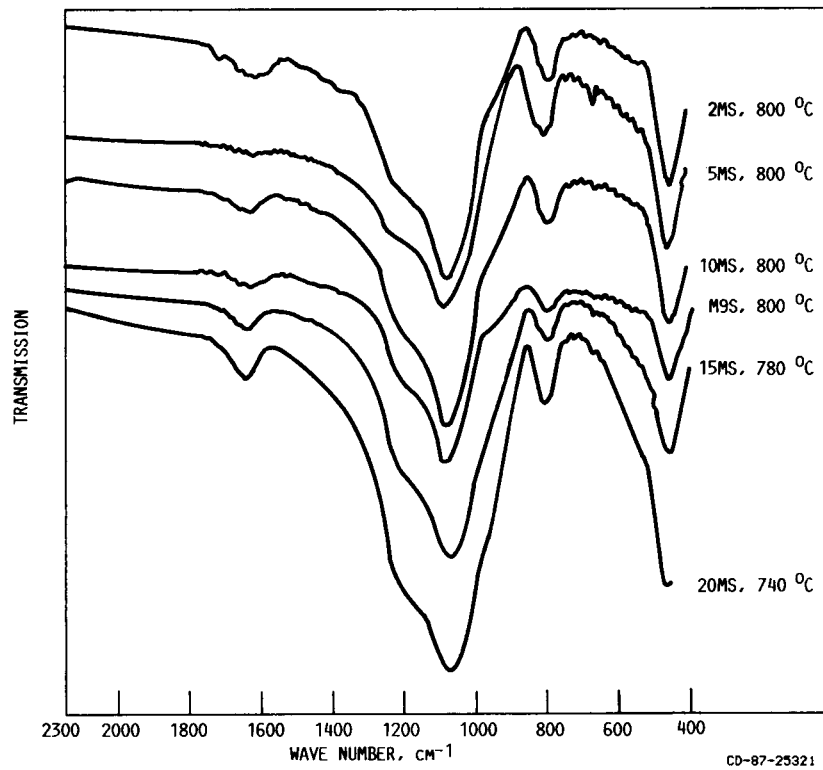
FIG. 11. - INFRARED SPECTRA OF MgO-SiO 2 GELS OF DIFFERENT COMPOSITIONS AFTER BEING FIRING TO VARIOUS TEMPERATURES AT 3 °C/MIN IN FLOWING AIR AND FURNACE COOLED.
