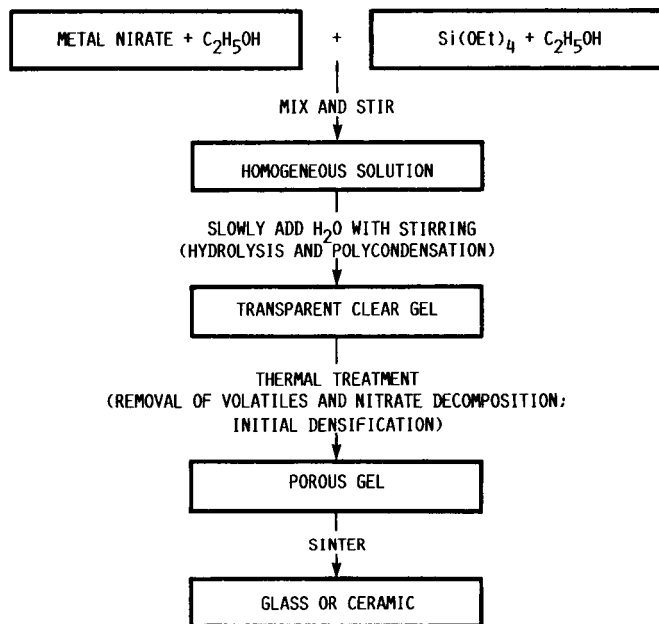
FIG. 2 - FLOW DIAGRAM OF THE SOL-GEL PROCESS FOR GLASS SYNTHESIS.
