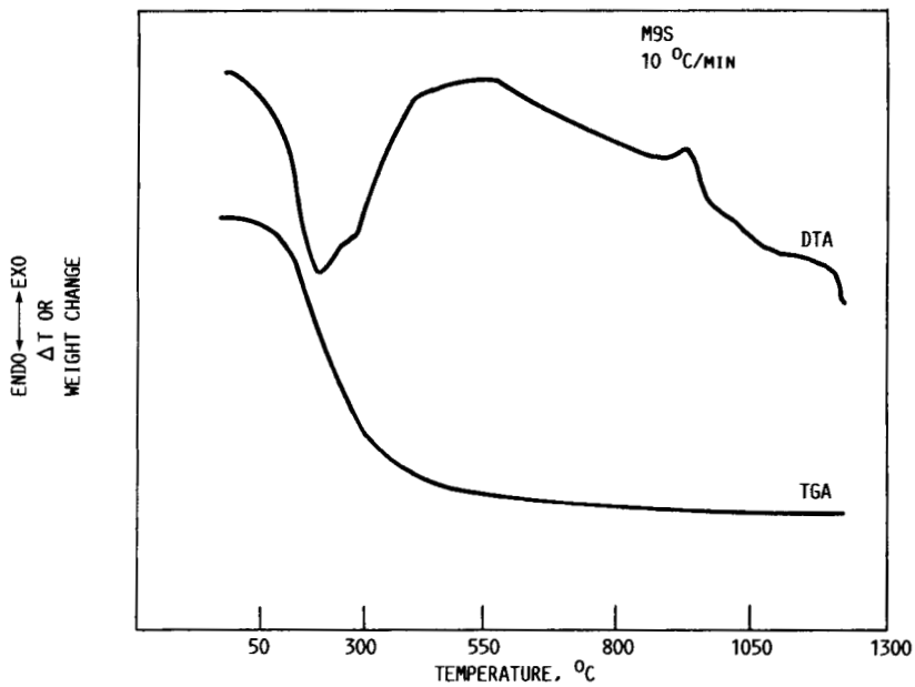
FIG. 7. - DTA AND TGA CURVES SIMULTANEOUSLY RECORDED ON THE SAME GEL SAMPLE OF COMPOSITION 10MgO-90SiO 2 (MOL %) DRIED AT 76 °C FOR 50 HR; HEATING RATE 10 °C/MIN IN FLOWING AIR.
