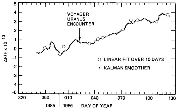
Fig. 5. Frequency offset, Australia-UTC (NBS)
