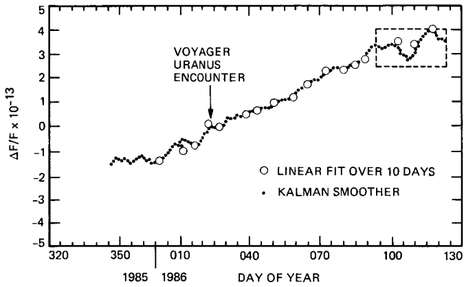
Fig. 4. Frequency offset, California-UTC (NBS)
