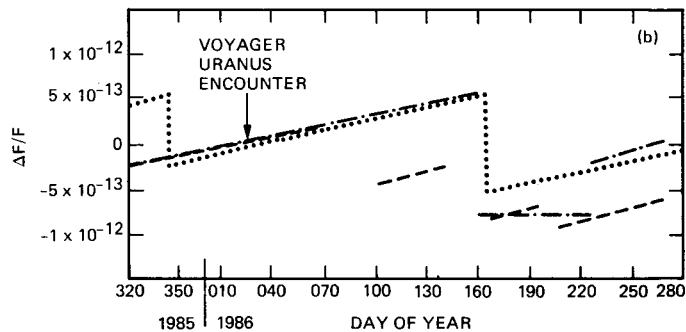
Fig. 2. Time and frequency offset with respect to UTC (NBS)
