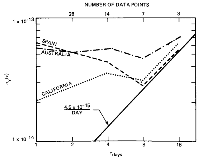
Fig. 7. Allan variance with respect to UTC (NBS)
