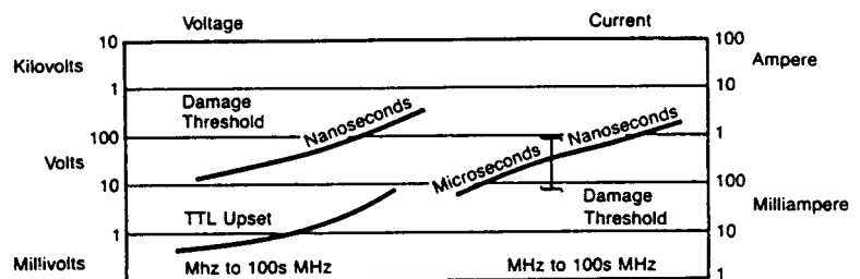
Figure 4.3-3 Trade—Digital Circuits
