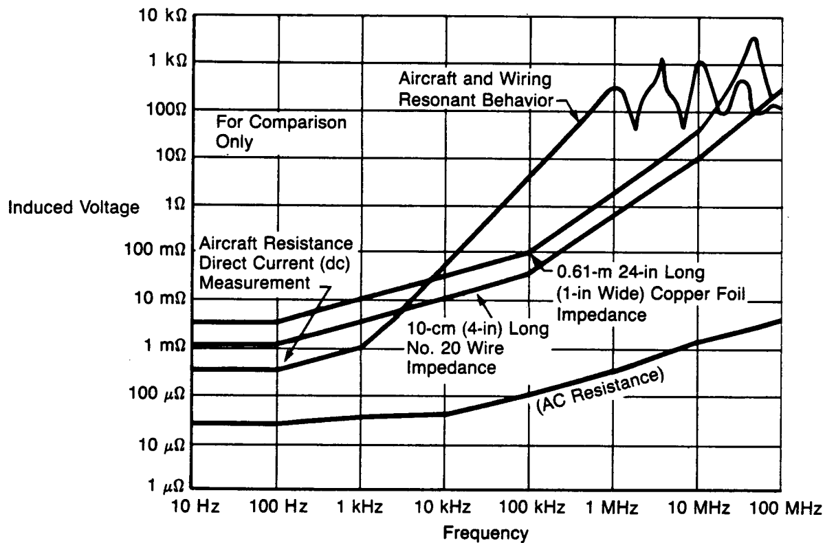
Figure 3.5-17 Aircraft and Strap Resonance
