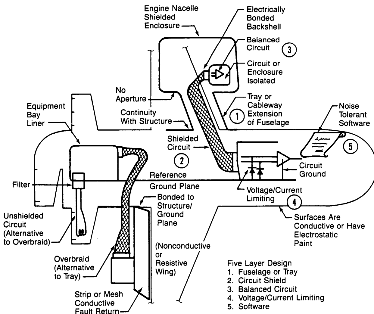
Figure 4.2-1 Layered Design
