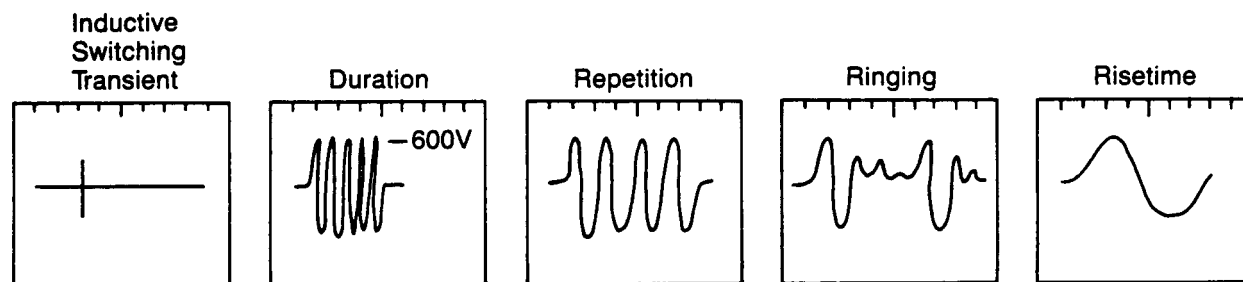
Figure 4.1-13 Transient Ringing
