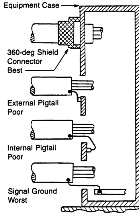
Figure 3.4-6 Shield Ties
