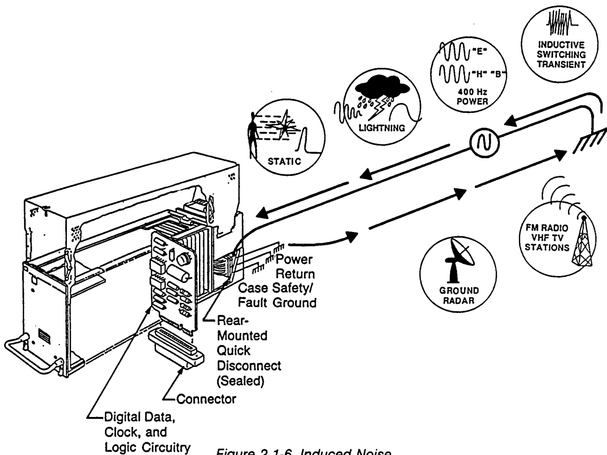
Figure 2.1-6 Induced Noise
