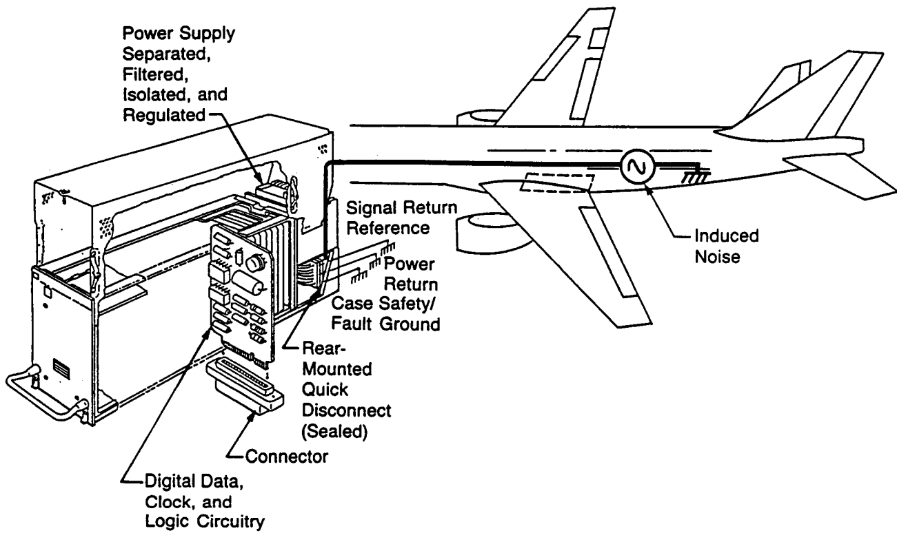
Figure 2.1-5 Structure Return
