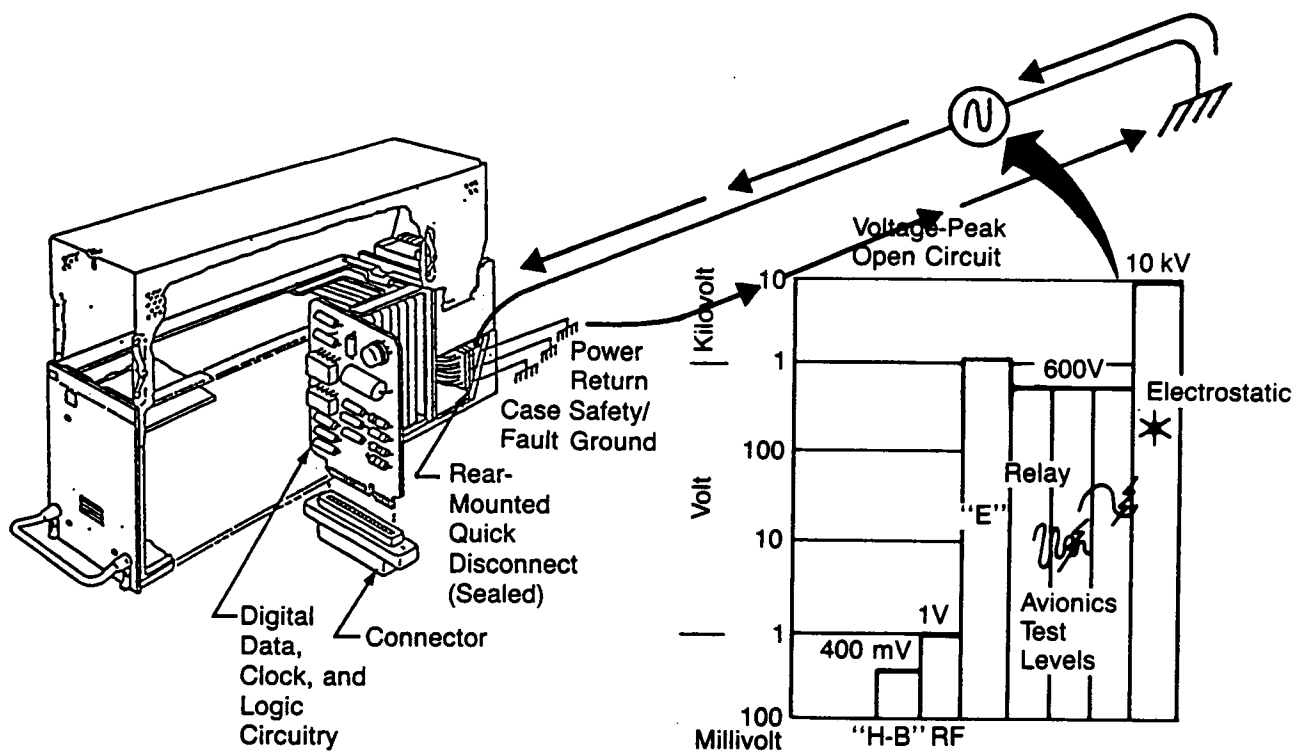
Figure 2.1-7 Noise Voltages
