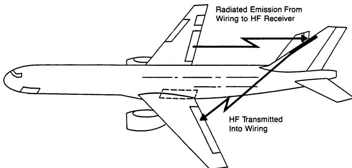
Figure 2.1-20 Radiated Emission
