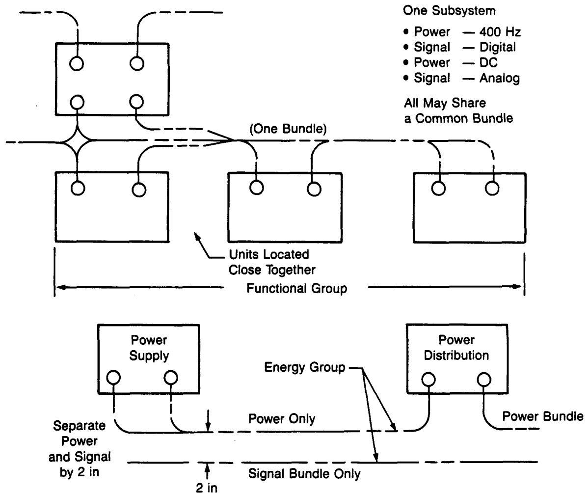
Figure 3.4-2 Wiring Categories
