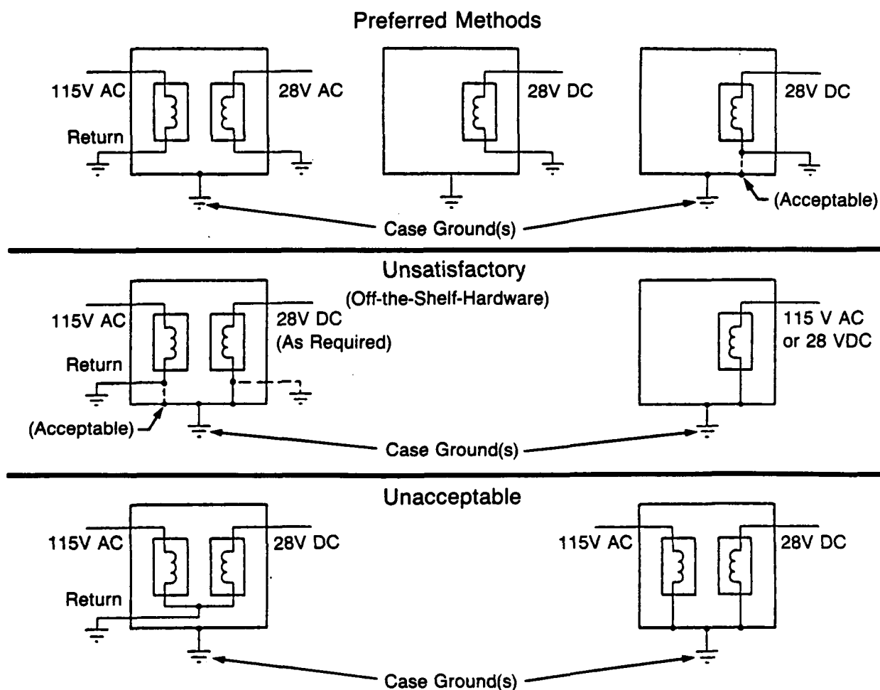
Figure 3.5-11 Power Returns
