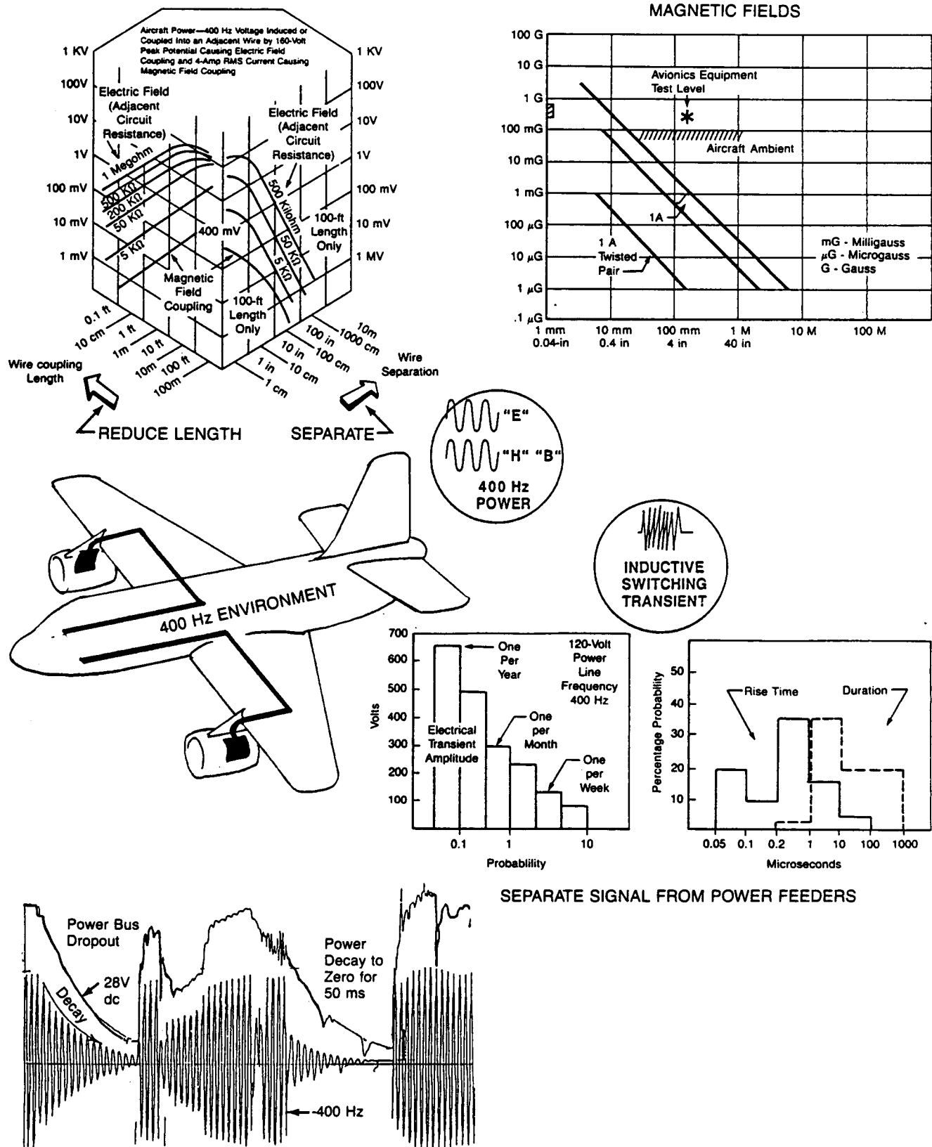
Figure 4.3-2 Trade—Wire Length/Separation
