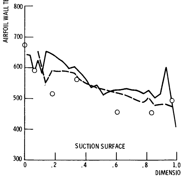
(a) Reynolds number = 1 250 000.
