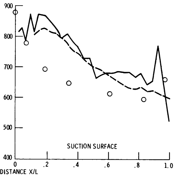
(b) Reynolds number = 1 900 000.
