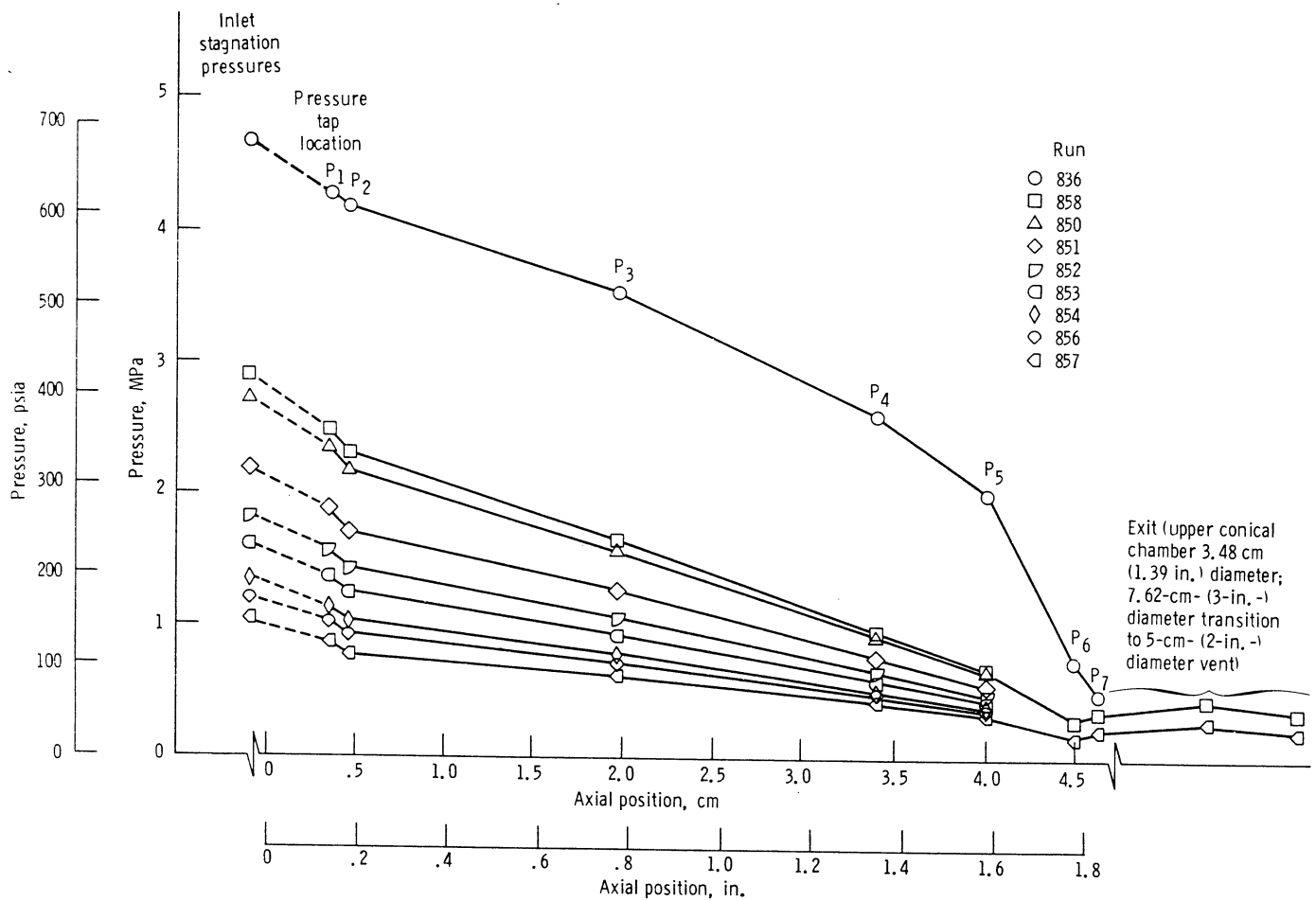
Figure 20.—Axial pressure distribution for liquid hydrogen flow through straight cylindrical seal in concentric position—third set of data.
