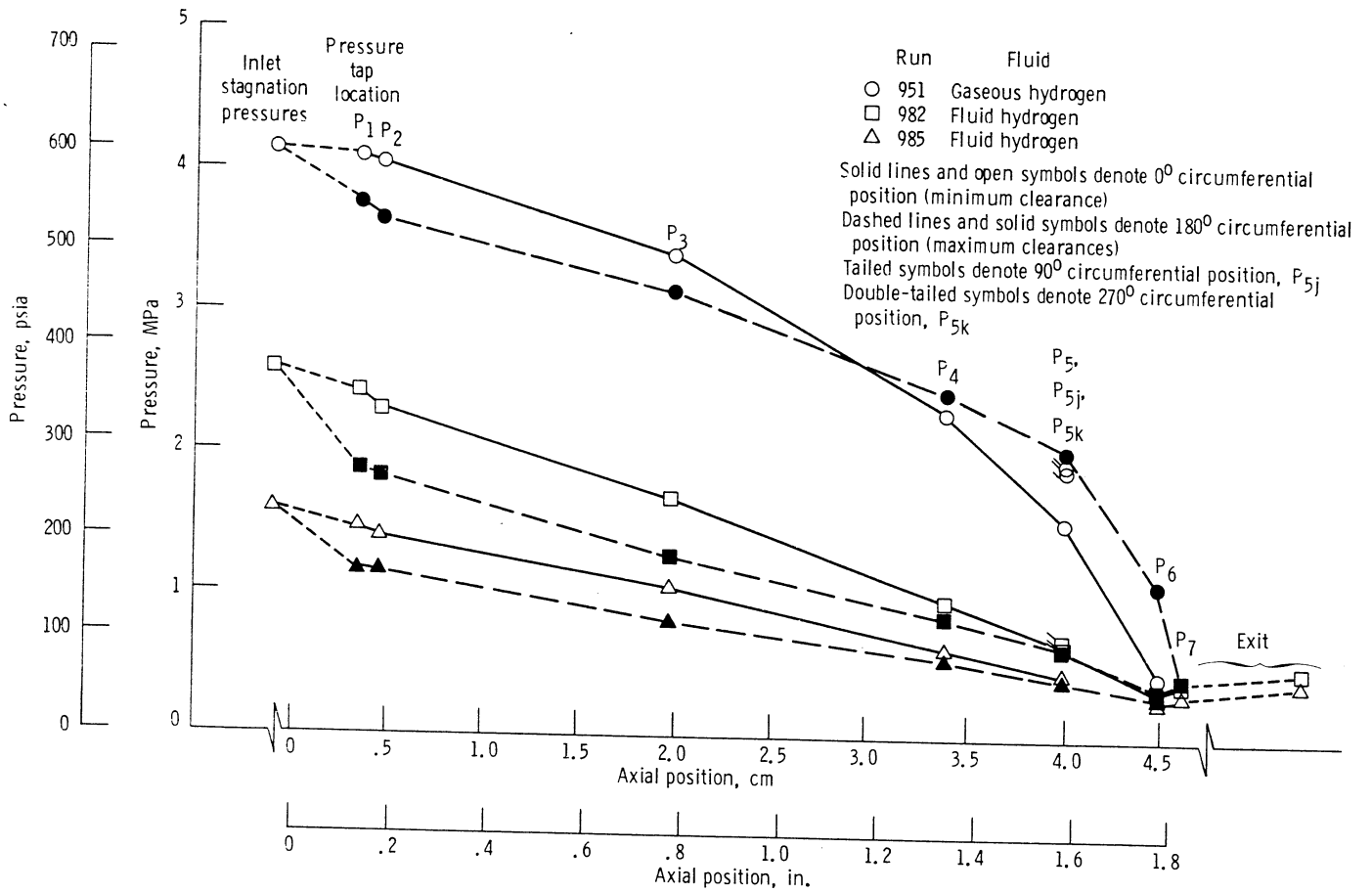
Figure 28.—Axial pressure distribution for gaseous and fluid hydrogen flow through straight cylindrical seal in fully eccentric position.
