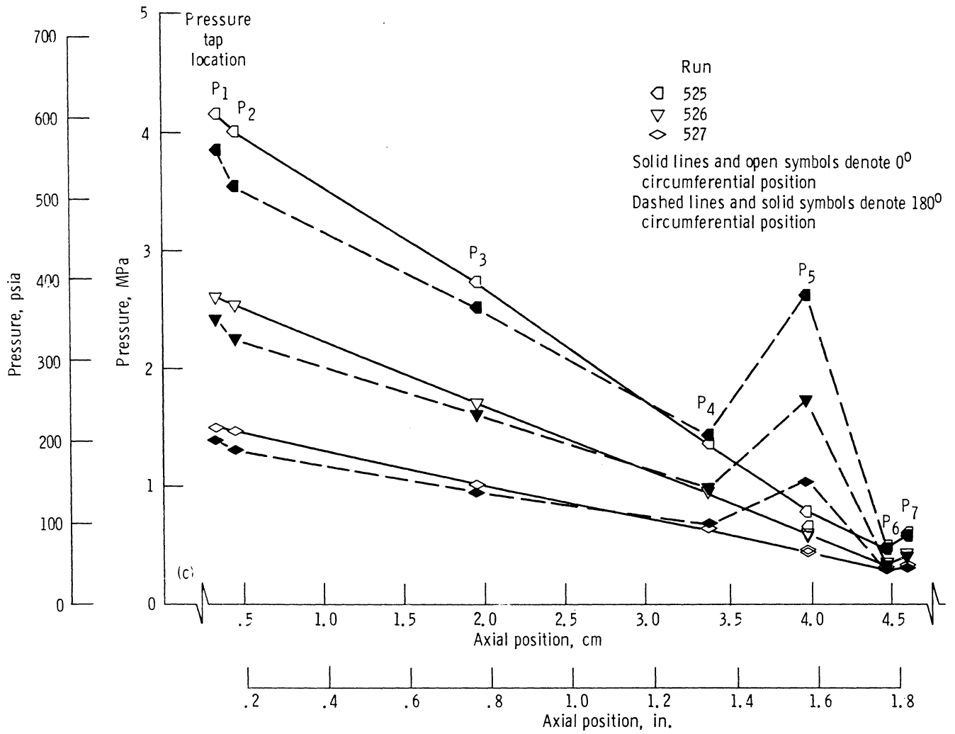
(c) Fluid nitrogen; runs 525 to 527.
