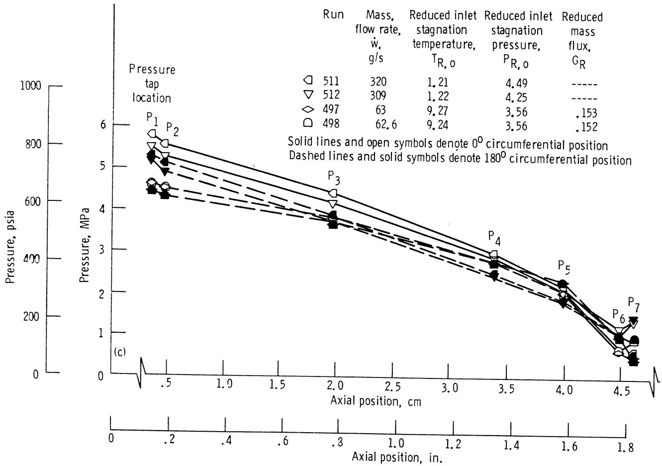
(c) Fluid hydrogen; runs 497, 498, 511, and 512.
