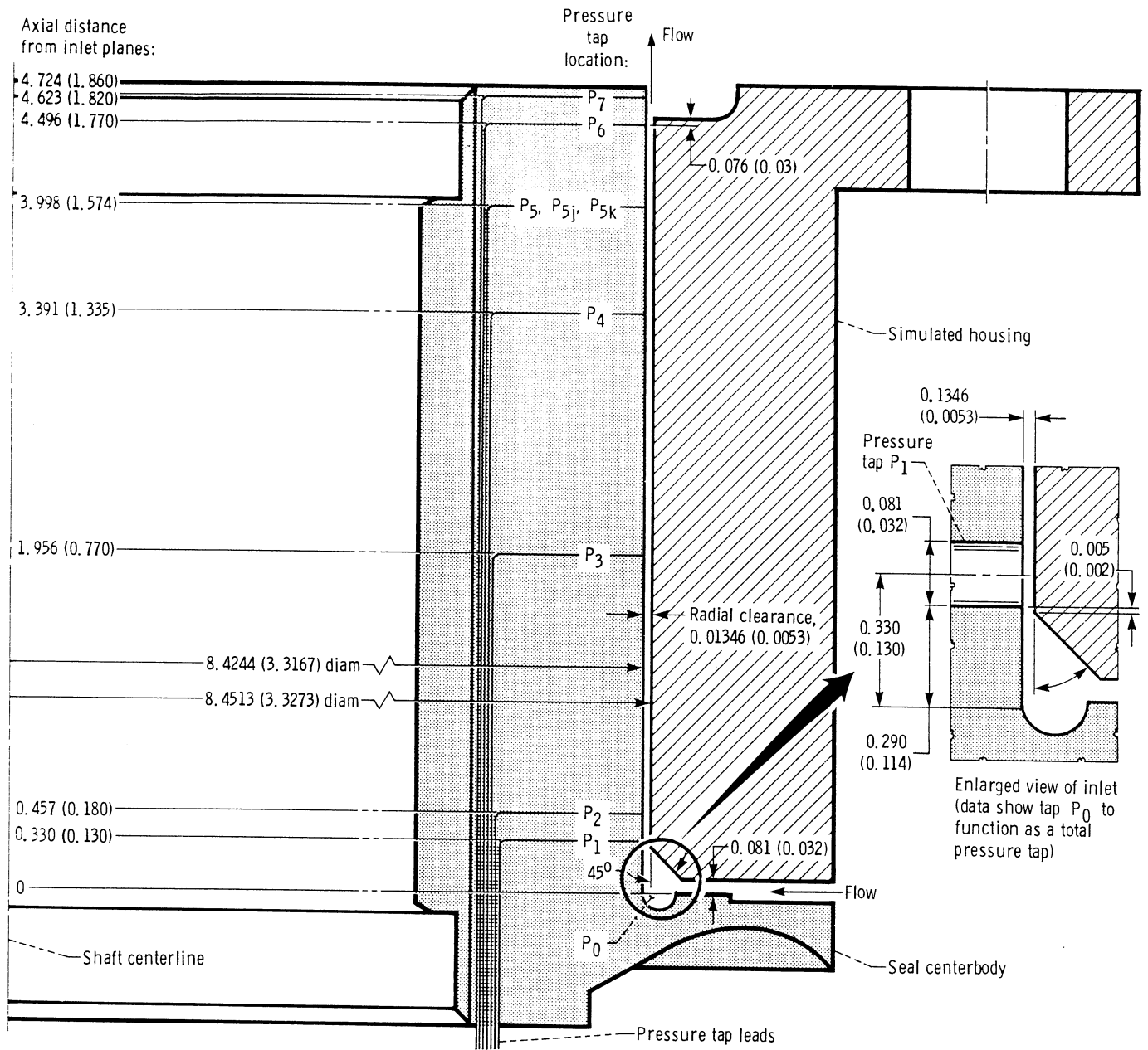
Figure 6.—Overview of pressure taps and geometry for straight cylindrical seal. (Linear dimensions are in centimeters (inches).)
