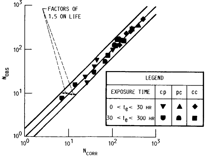
(C) EXPOSURE TIME MODIFIED STRAINRANGE PARTITIONING METHOD.
