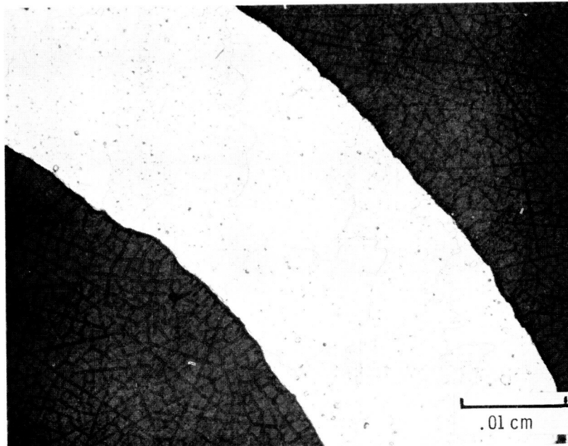
FIGURE 6. - CROSS SECTION OF Pt/Y 2 O 3 TUBE BEFORE AND AFTER TESTING FOR 2000 HR AT 1300 °C IN CO 2 .
