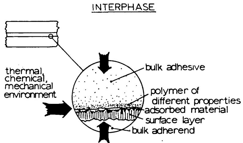
Figure III-4 Schematic representation of the components of the three dimensional interphase between fiber and matrix. (37)
