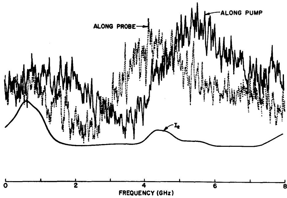
Fig. 15. Typical result of flow-velocity measurements. The obvious shift between the peaks of these Rayleigh-Brillouin-gain spectra corresponds to a relative velocity of 350 m/sec. [Following Herring et al., 1983b.]
