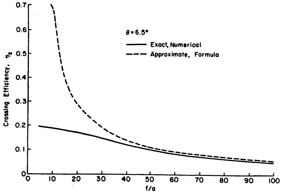
Fig. 3. Crossing efficiency of the two-photon process as a function of f/a ( \theta = 6.5^\circ ).
