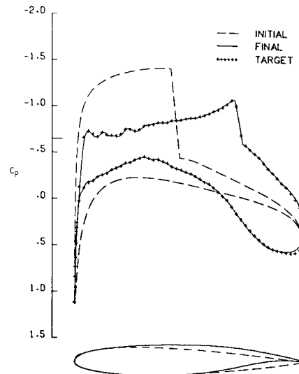
Fig. 9 Airfoil design code pressure distributions C_p .
