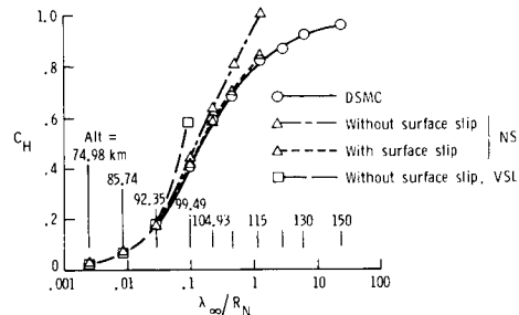
Fig. 14 Heat transfer coefficient versus Knudsen number.
