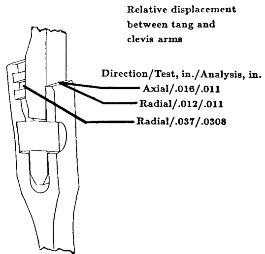
Fig. 16 Deformed geometry (exaggerated deflections).
