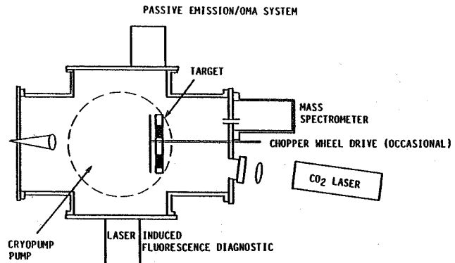
Fig. 8. Schematic of new O-atom facility
