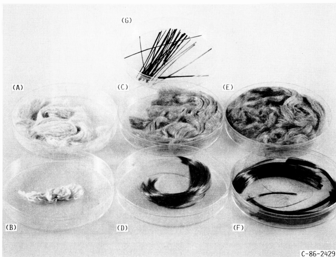
FIGURE 2. - GRAPHITE FIBERS BEFORE AND AFTER FLUORINATION AT 1 ATM BY FLUORINE GAS AT 450 °C FOR 21 HR. (A) P-55, (B) T-300, (C) P-75, (D) BROMINATED P-75, (E) P-100, (F) BROMINATED P-100, (G) TYPICAL PRISTINE GRAPHITE FIBER.
