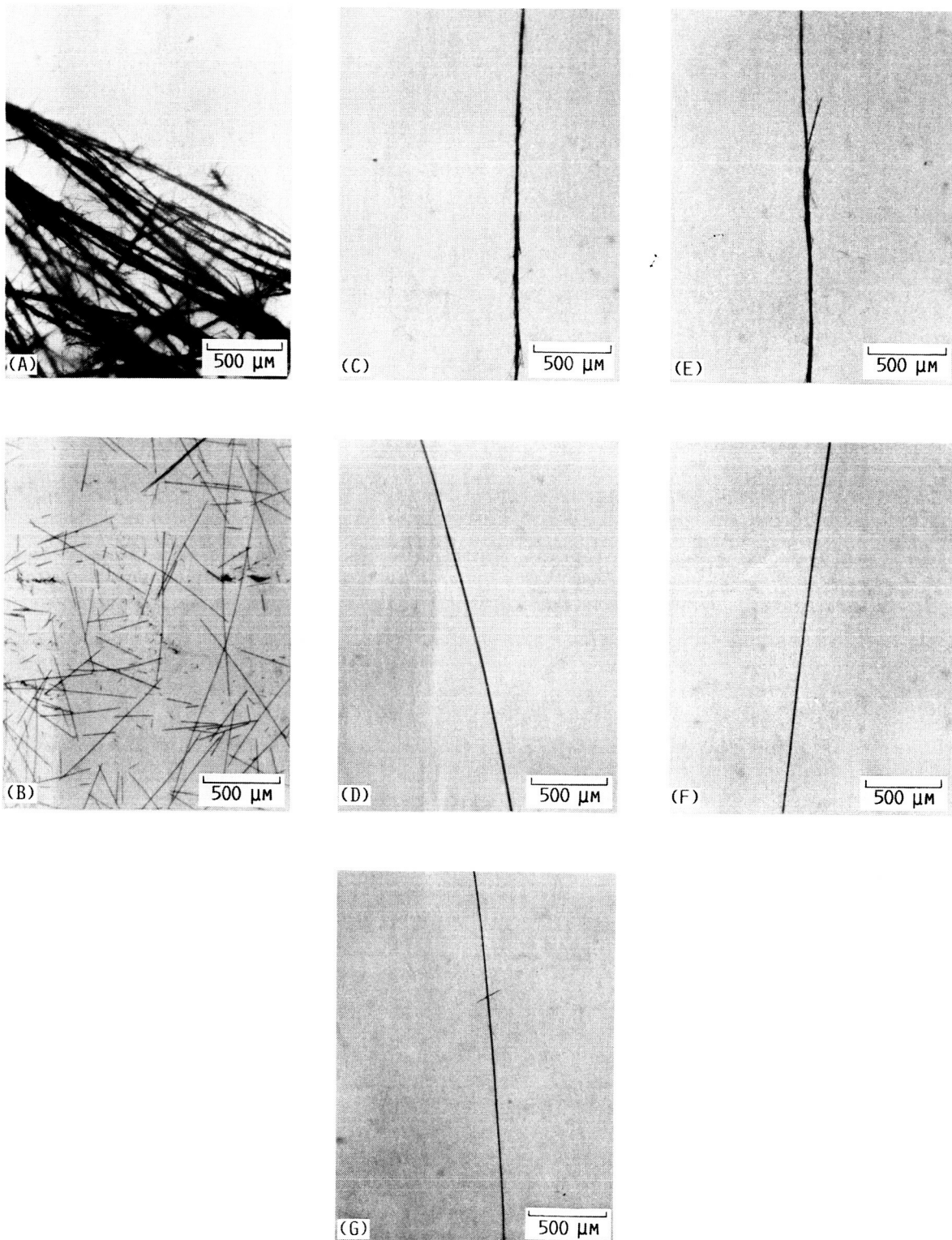
FIGURE 3. - MICROGRAPH OF GRAPHITE FIBERS AFTER FLUORINATION AT 1 ATM BY FLUORINE GAS AT 450 °C FOR 21 HR. (A) P-55, (B) T-300, (C) P-75, (D) BROMINATED P-75, (E) P-100, (F) BROMINATED P-100, (G) FLUORINE INTERCALATED P-75.
