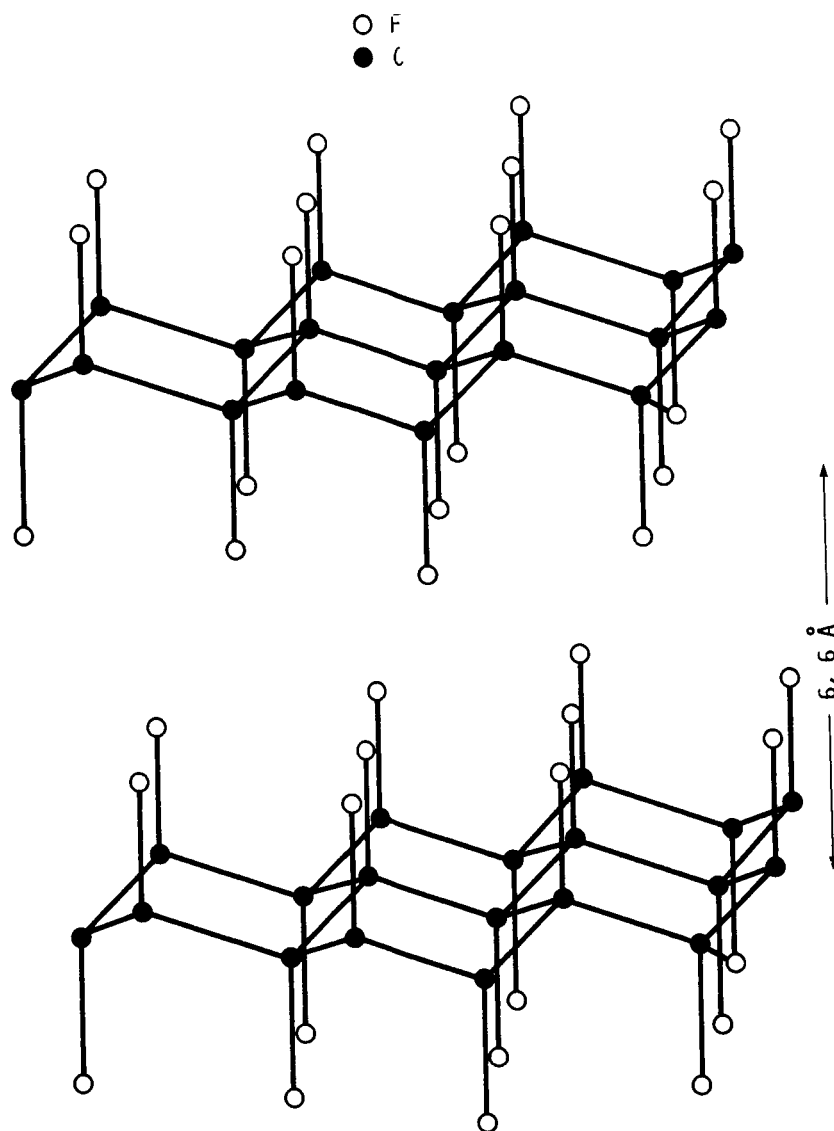
FIGURE 1. - MOLECULAR STRUCTURE OF GRAPHITE FLUORIDE (CF)_n .
