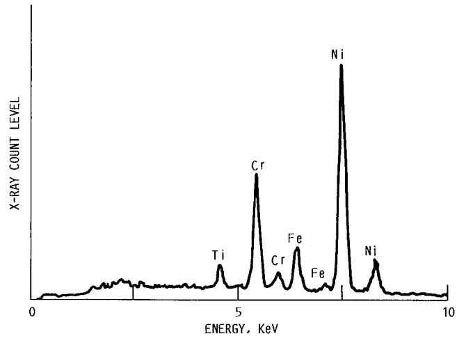
FIGURE 10. - EDAX SPECTRUM OF FOIL SURFACE AFTER SLIDING AGAINST UNMODIFIED COATING (PS218) WITH NO LUBRICANT ADDITIVES.
