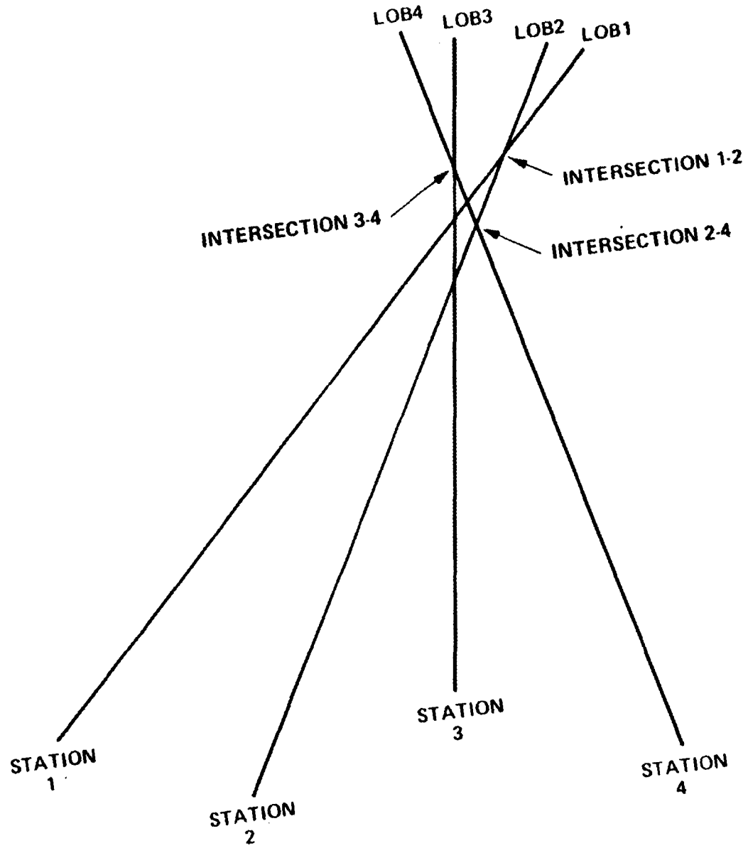
Figure 3-4. Set of LOBs Showing Intersections After LOB5 has been Removed
