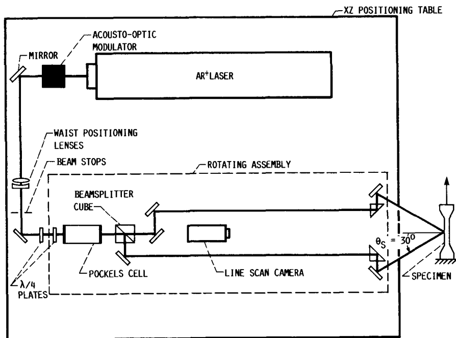
FIGURE 9. - SCHEMATIC OF THE PHASE II OPTICAL DESIGN.
