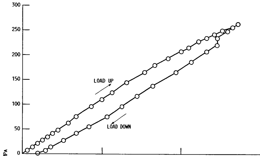
FIGURE 6A. - HYSTERESIS MEASURED BY THE OPTICAL GAUGE.
