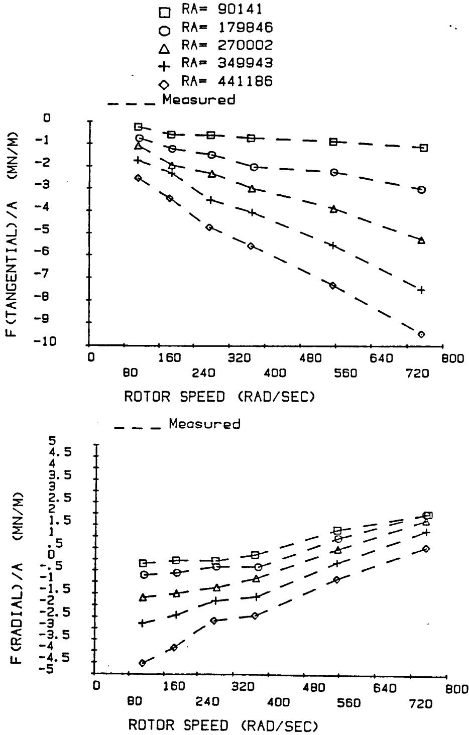
Figure 47. F_r/A and F_\theta/A for helically-grooved-stator seal 8, \alpha = 70^\circ .
