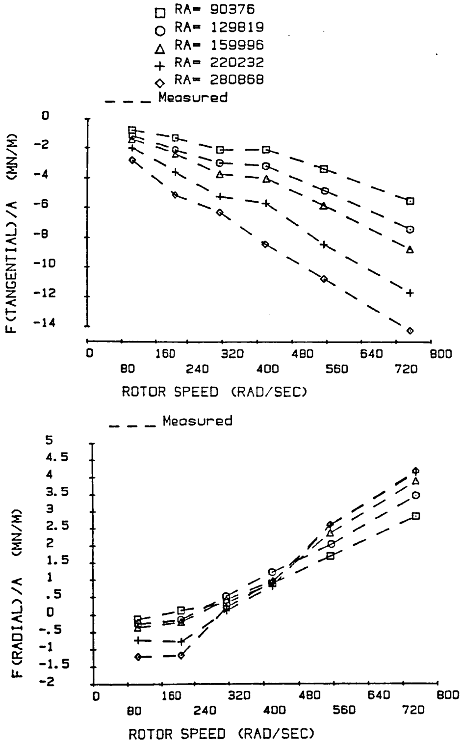
Figure 41. F_r/A and F_\theta/A for helically-grooved-stator seal 2, \alpha = 15^\circ .
