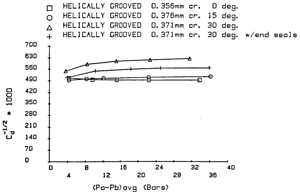
Figure 39. C_d^{-1/2} versus \Delta P for helically-grooved-stator seals.
