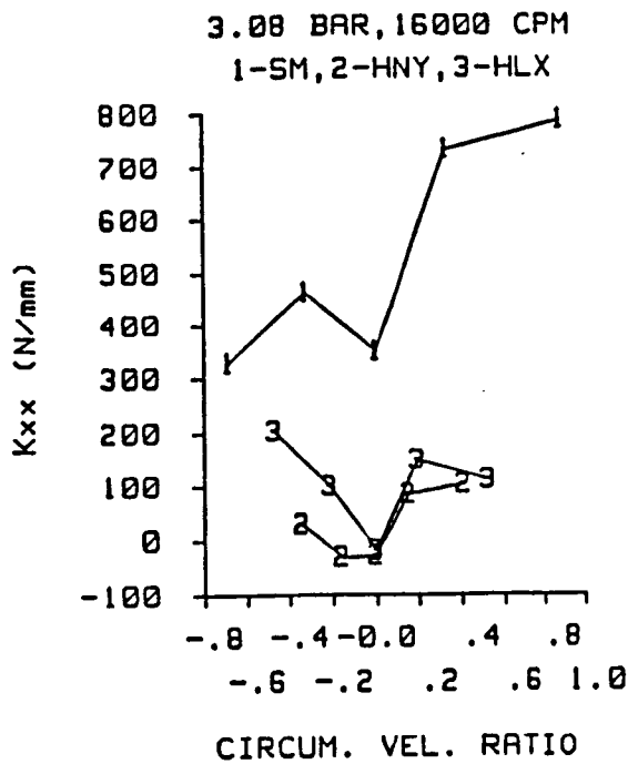
Figure 55(a). K_{xx} and K_{xy} versus u_{\theta 0} for smooth (1), honeycomb (2), and helix (3) stators at 16,000 CPM.
