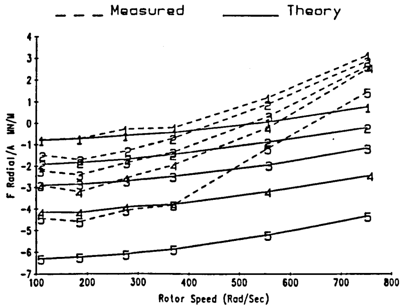
Figure 24. Measured and theoretical 2 results for F_r/A and F_\theta/A ; hole-pattern stator 2.
