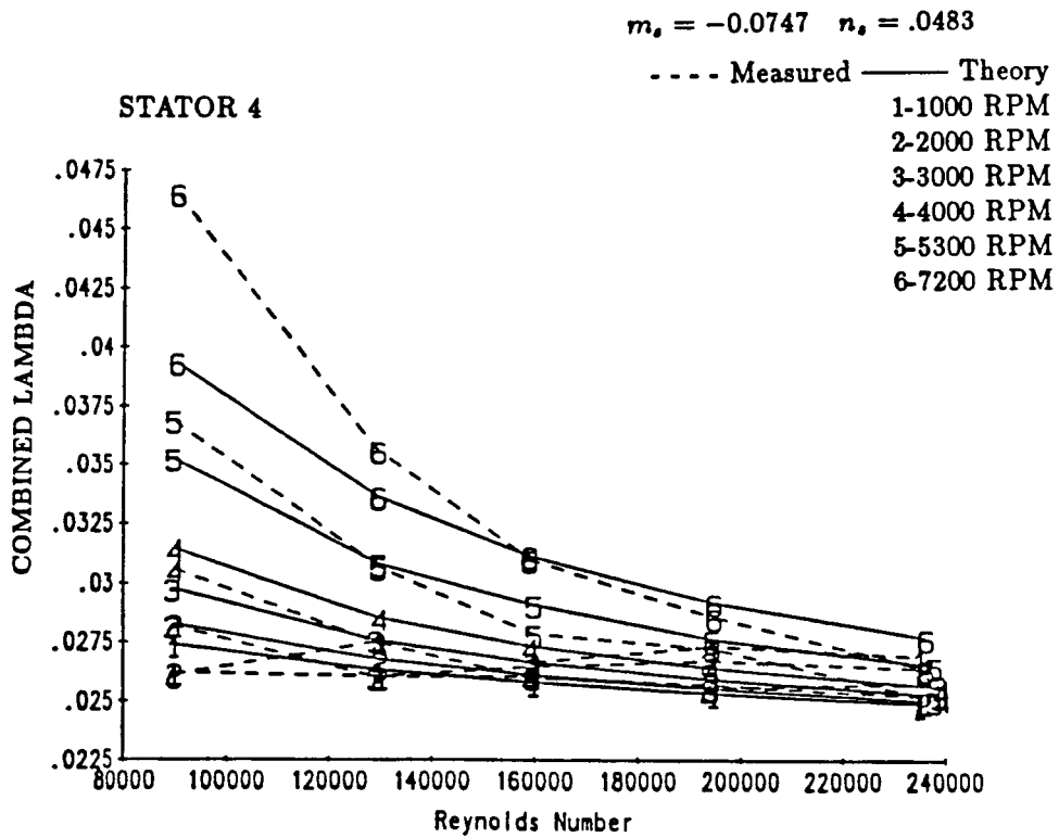
Figure 17. Combined lambda data for damper seals with hole-pattern-stators 3 and 4.
