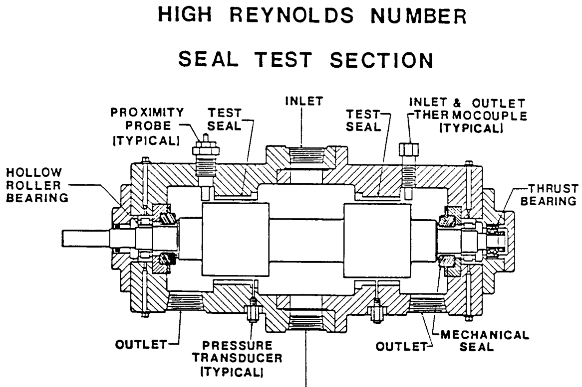
Figure 2. High-Reynolds-Number Seal Test Section.
