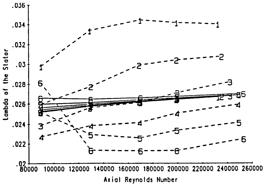
Figure 21. Stator lambda data for hole-pattern-stators 5 and 6.
