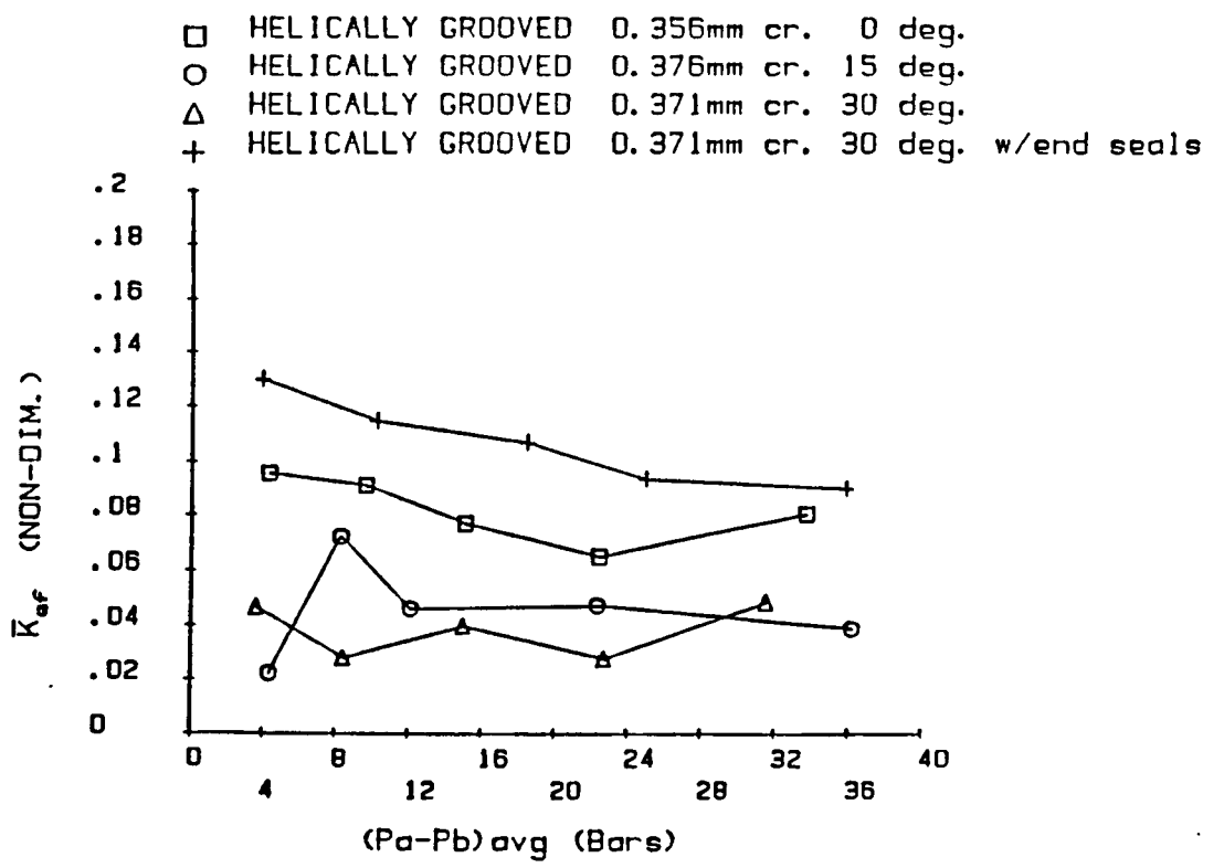
Figure 48. \bar{K}_{ef} versus \Delta P for the helically-grooved stator seals.
