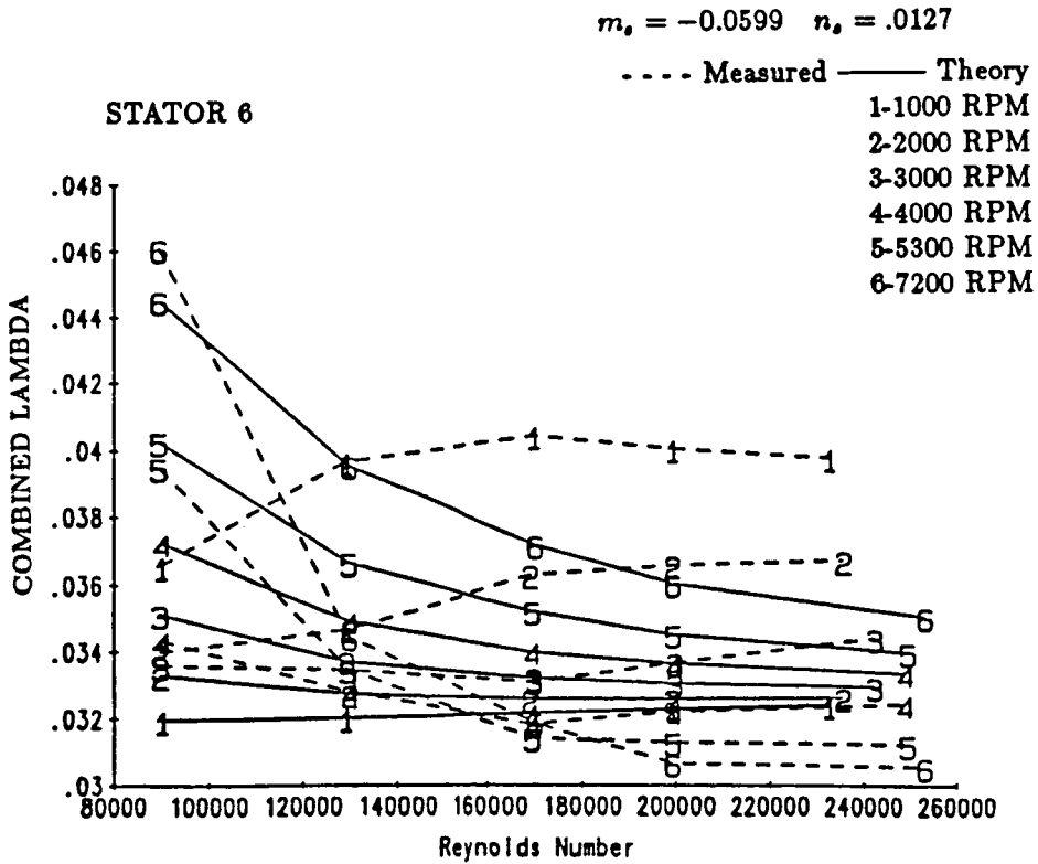
Figure 18. Combined lambda data for damper seals with hole-pattern-stators 5 and 6.
