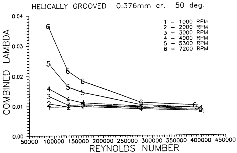
Figure 36. Combined-lambda, \lambda_c , data for helically-grooved-stators
