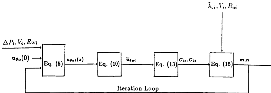
Figure 4. Flowchart for the solution of the empirical coefficients for equal rotor and stator surface roughnesses. The subscript i denotes the i th data point.
