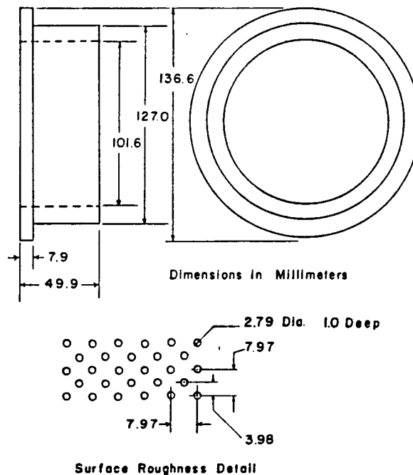
Figure 1. Hole-pattern stator.
