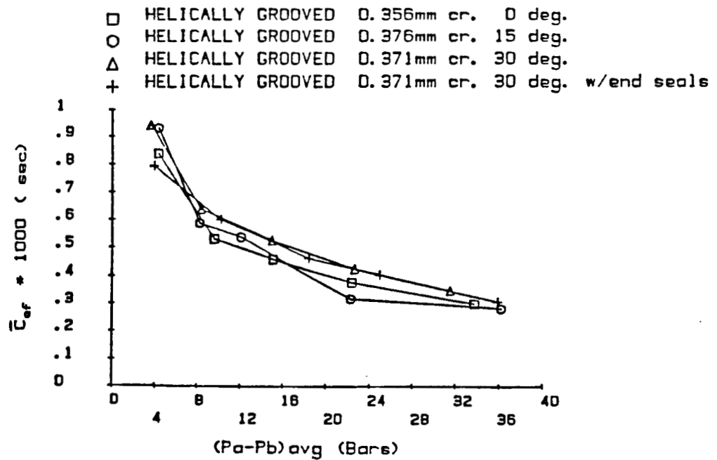
Figure 49. \bar{C}_{ef} versus \Delta P for the helically-grooved stator seals.
