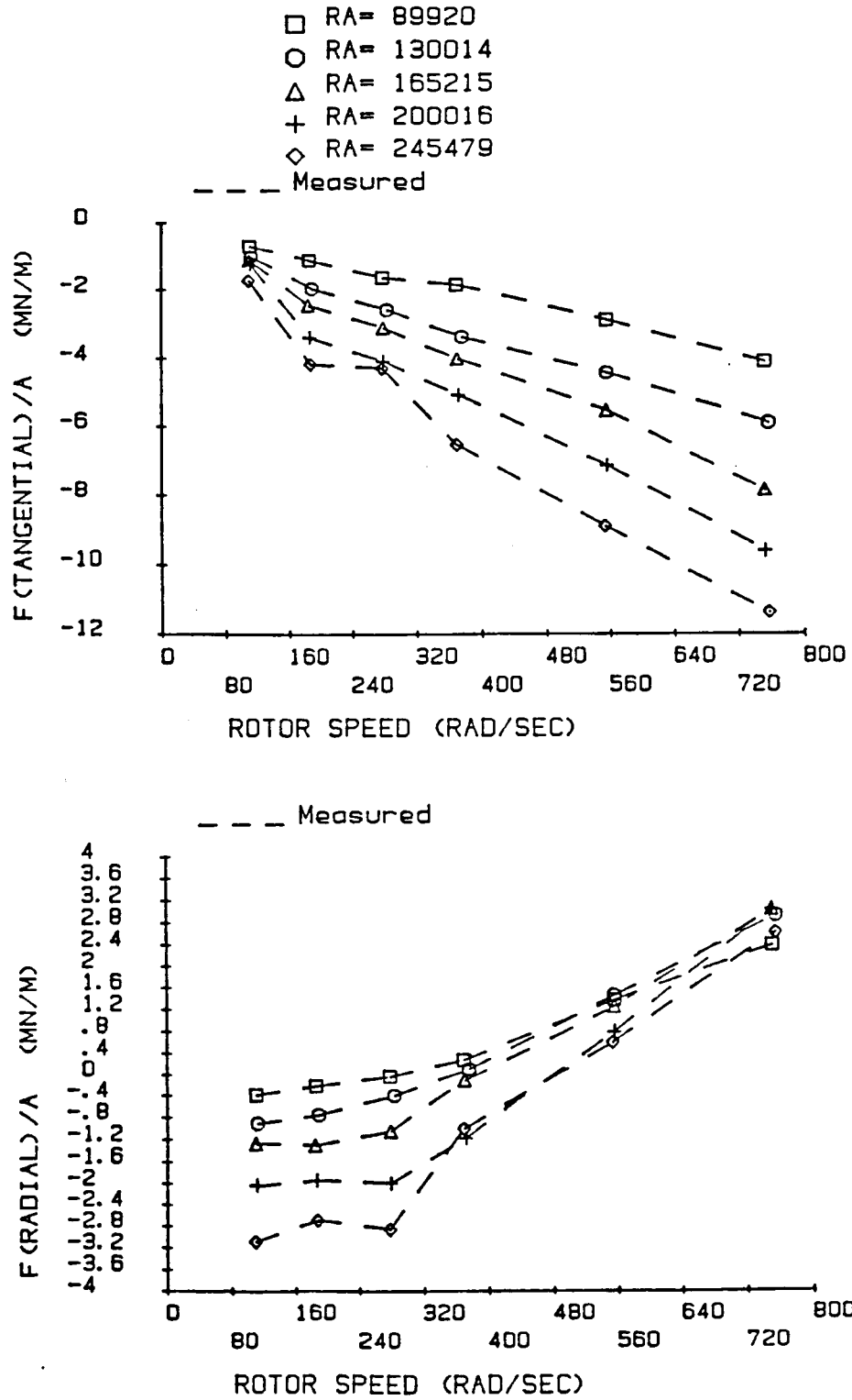
Figure 40. F_r/A and F_\theta/A for helically-grooved-stator seal 1, \alpha = 0^\circ .
