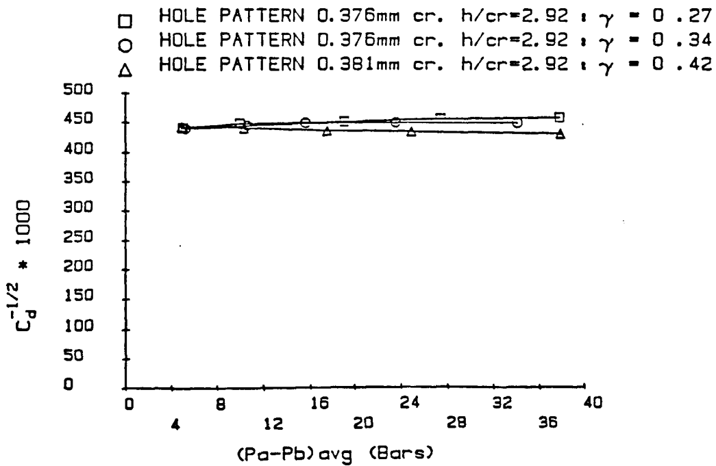
Figure 22. C_d^{-1/2} for hole-pattern-stator seals.
