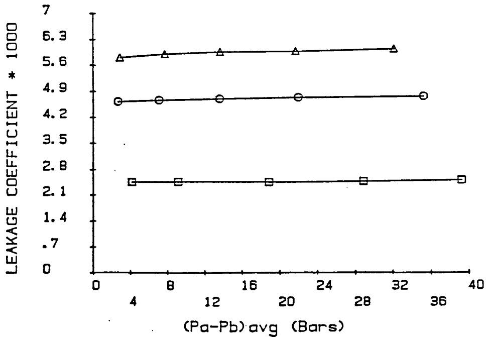
Figure 8. C_d^{-1/2} and C_L for smooth seals; C_r = 0.254, 0.381, \text{ and } 0.508\text{mm} .
