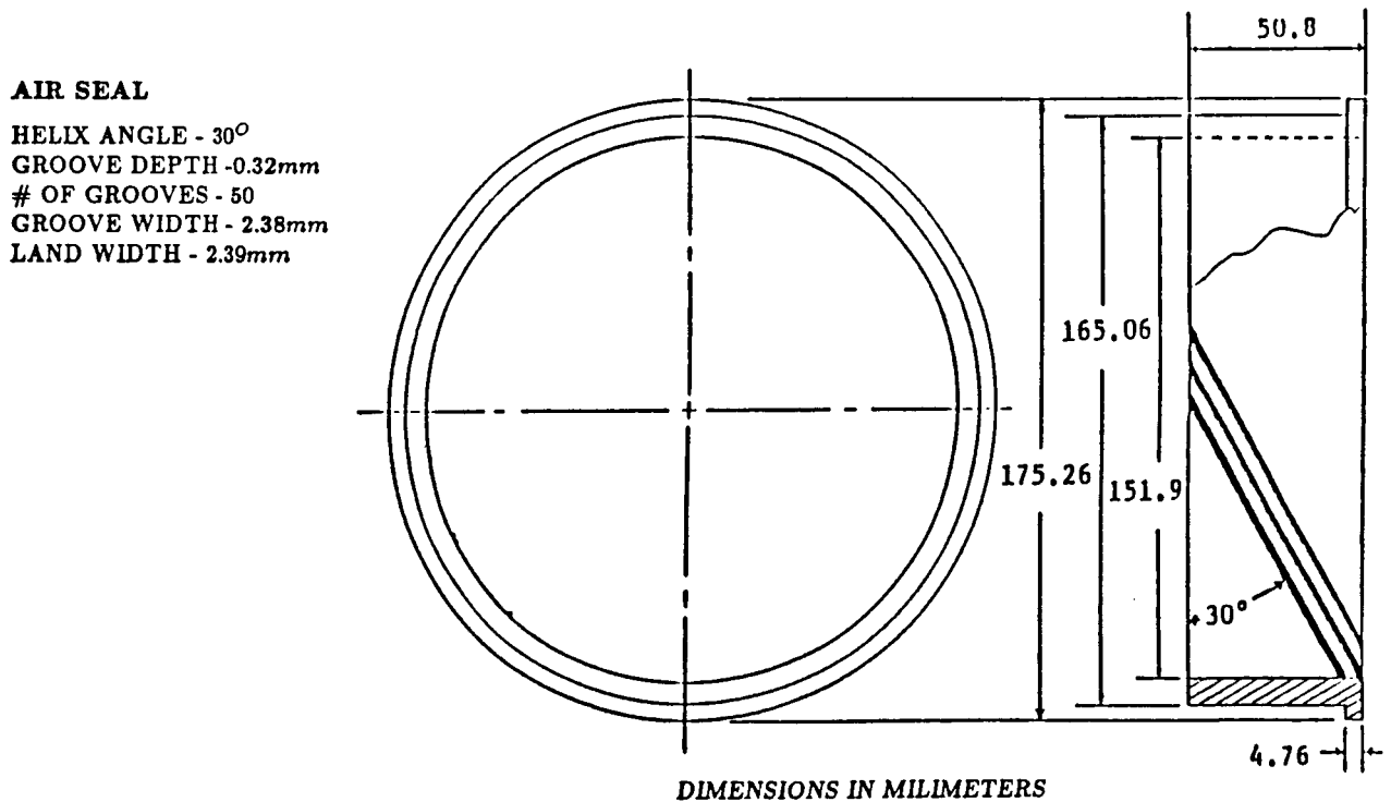
Figure 50. Helically Grooved Air Seal
