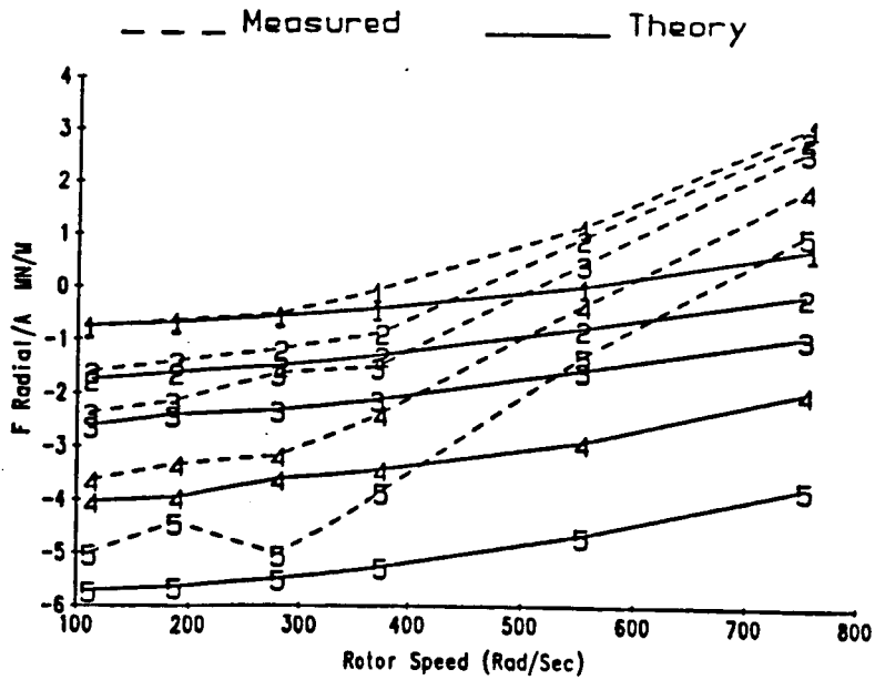
Figure 25. Measured and theoretical 2 results for F_r/A and F_\theta/A ; hole-pattern stator 3.
