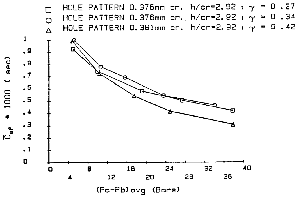
Figure 32. \bar{C}_{ef} for hole-pattern stators 1 through 6.
