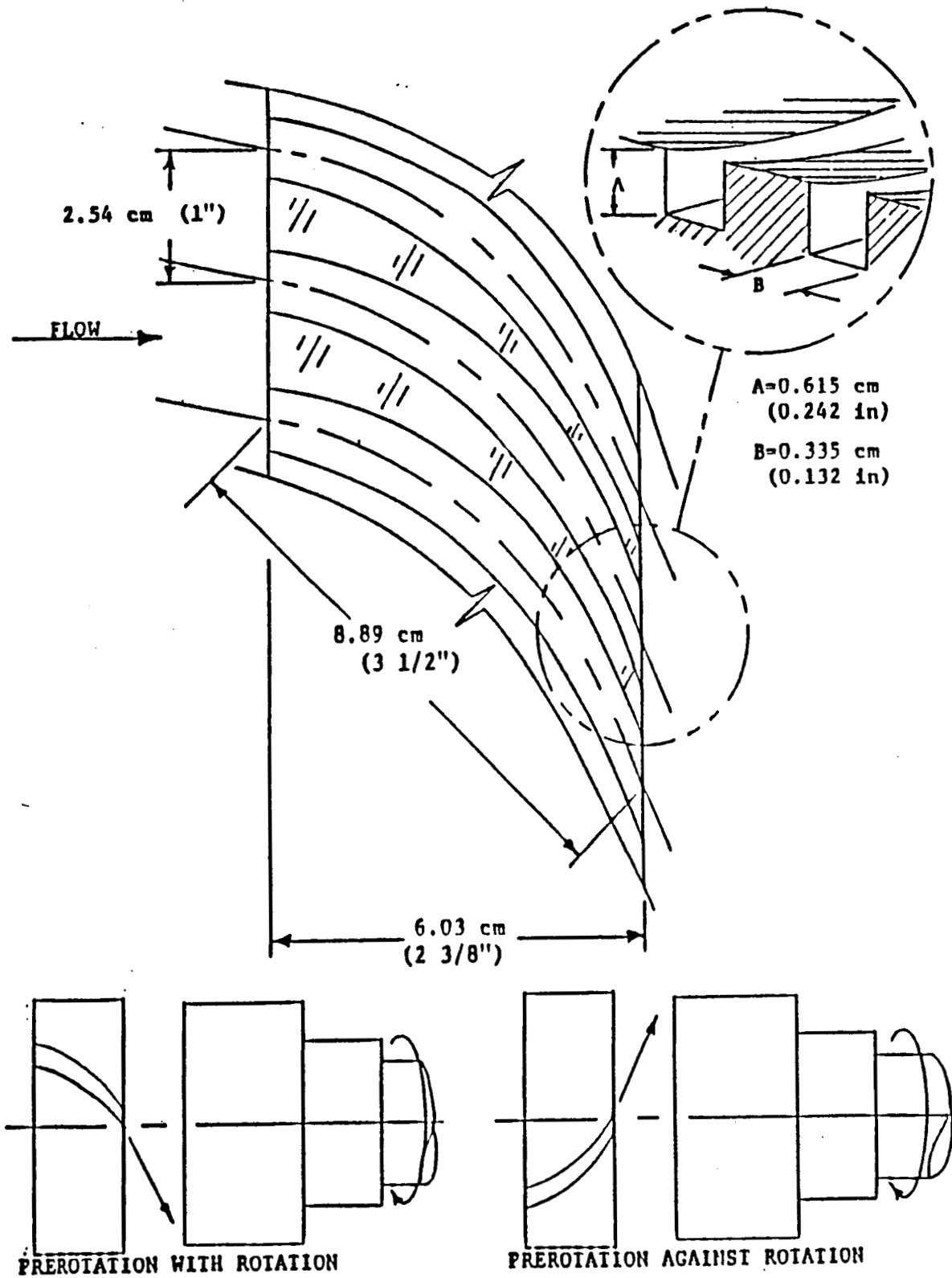
Figure 53. Inlet guide vane detail.
