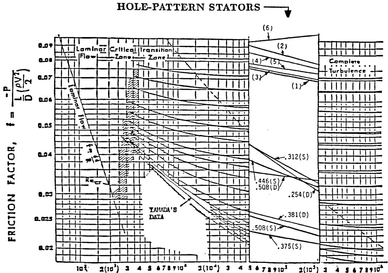
Figure 57. Measured friction-factor data plotted on a Moody diagram.
