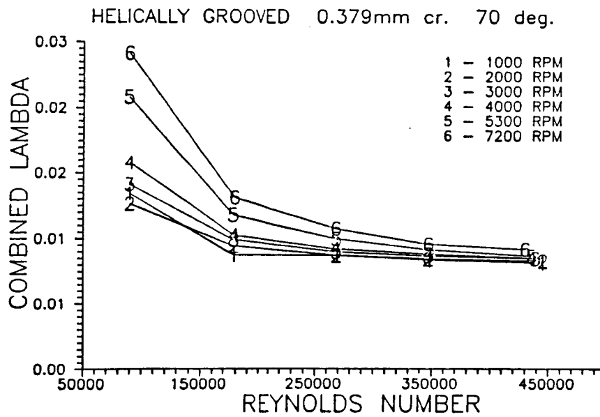
Figure 37. Combined-lambda, \lambda_c , data for helically-grooved-stators 7 and 8 versus R_a and \omega .
