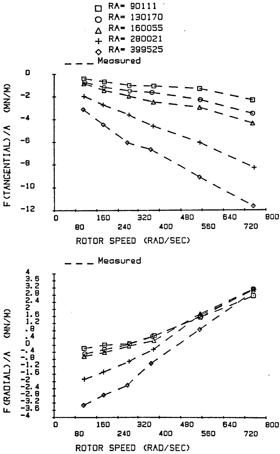
Figure 45. F_r/A and F_\theta/A for helically-grooved-stator seal 6, \alpha = 50^\circ .
