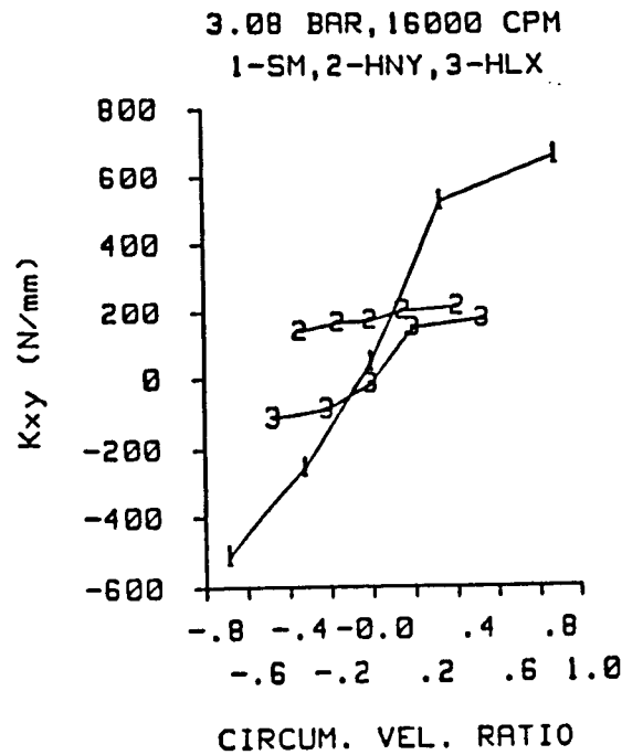
Figure 55(a). K_{xx} and K_{xy} versus u_{\theta 0} for smooth (1), honeycomb (2), and helix (3) stators at 16,000 CPM.
