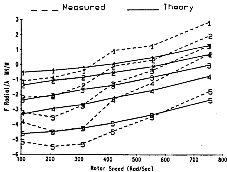
Figure 28. Measured and theoretical 2 results for F_r/A and F_\theta/A ; hole-pattern stator 6.
