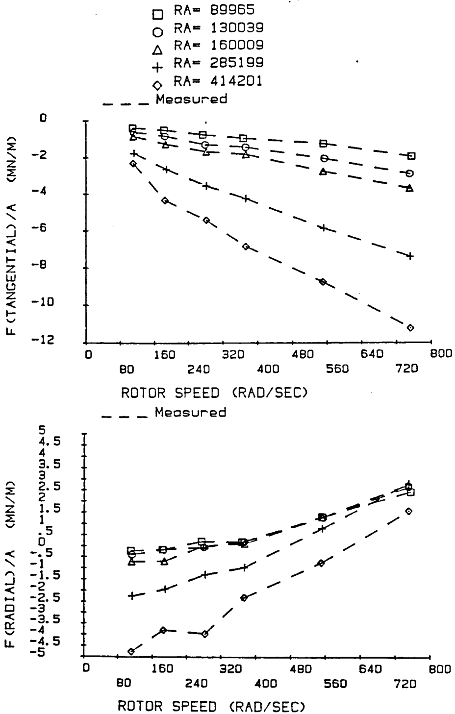
Figure 46. F_r/A and F_\theta/A for helically-grooved-stator seal 7, \alpha = 60^\circ .
