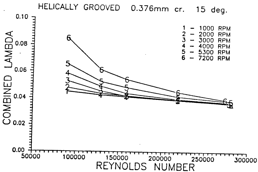
Figure 34. Combined-lambda, \lambda_c , data for helically-grooved-stators 1 and 2 versus R_a and \omega .
