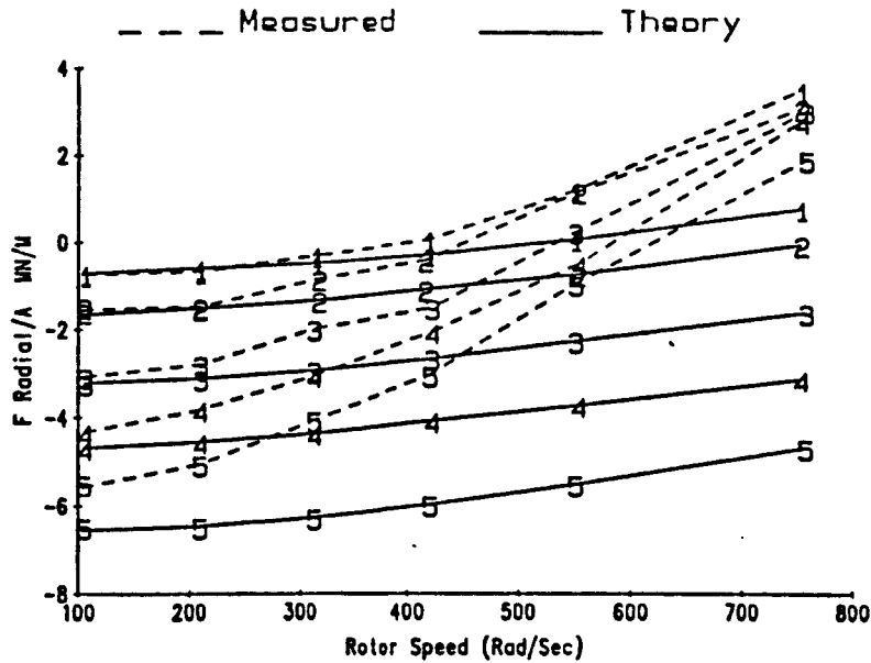
Figure 27. Measured and theoretical 2 results for F_r/A and F_\theta/A ; hole-pattern stator 5
