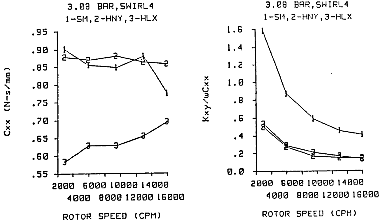
Figure 56(b). Test results for C_{xx} and K_{xy}/\omega C_{xx} versus running speed for smooth (1), honeycomb (2), and helix (3) stators versus running speed for maximum inlet-flow prerotation in the direction of shaft rotation.
