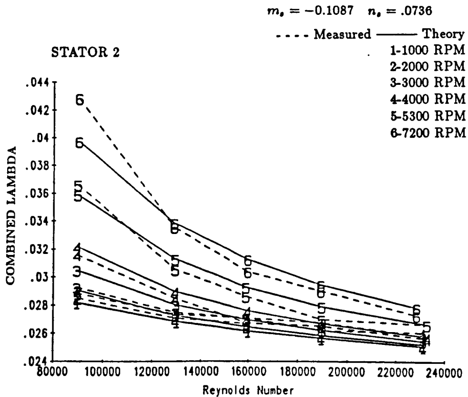
Figure 16. Combined lambda data for damper seals with hole-pattern-stators 1 and 2.
