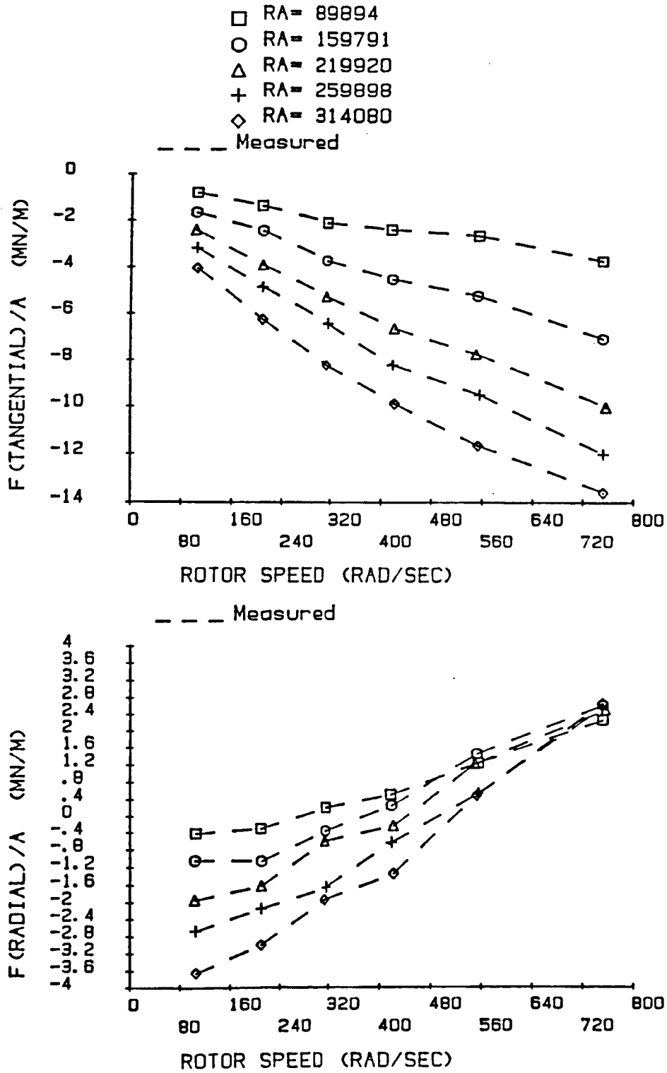
Figure 43. F_r/A and F_t/A for helically-grooved-stator seal 4, \alpha = 30^\circ with end lands.
