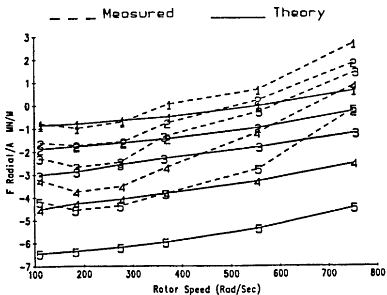
Figure 26. Measured and theoretical 2 results for F_r/A and F_{\theta}/A ; hole-pattern stator 4.
