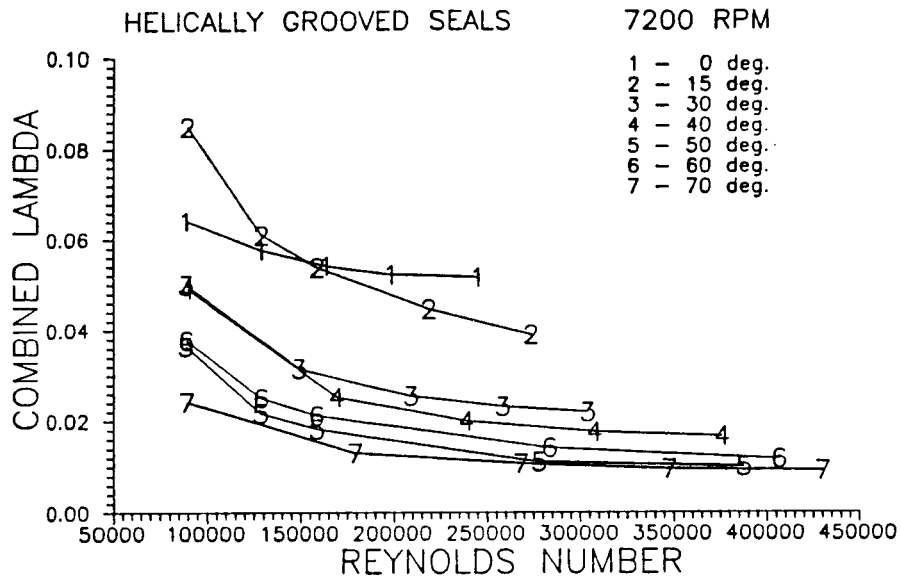
Figure 38. Combined-lambda data for helix-angles 0° through 70° at 7200 rpm, versus R_a .
