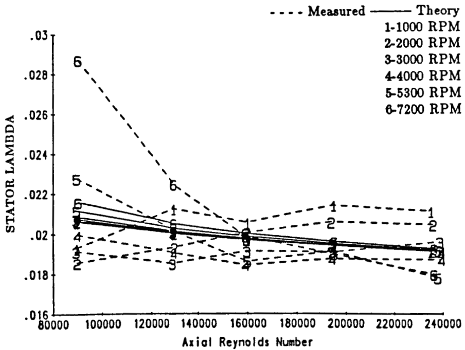
Figure 20. Stator lambda data for hole-pattern-stators 3 and 4.
