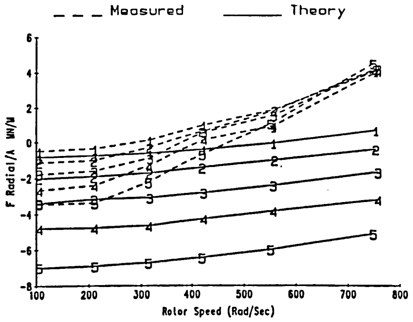
Figure 23. Measured and theoretical 2 results for F_r/A and F_\theta/A ; hole-pattern stator 1.
