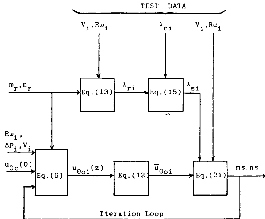
Figure 5. Flowchart for the solution of stator empirical turbulence coefficients m_s, n_s from test data and known rotor coefficients. The subscript i denotes the i th data point
