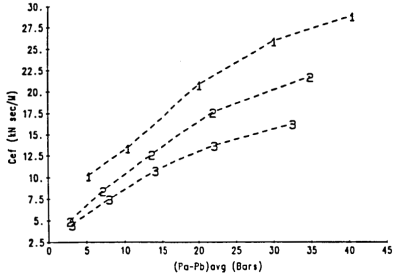
Figure 13. C_{ef} versus \Delta P for smooth seals at three different clearances.
