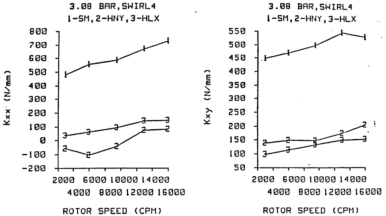
Figure 56(a). Test results for K_{xx} and K_{xy} versus running speed for smooth (1), honeycomb (2), and helix (3) stators versus running speed for maximum inlet-flow prerotation in the direction of shaft rotation.
