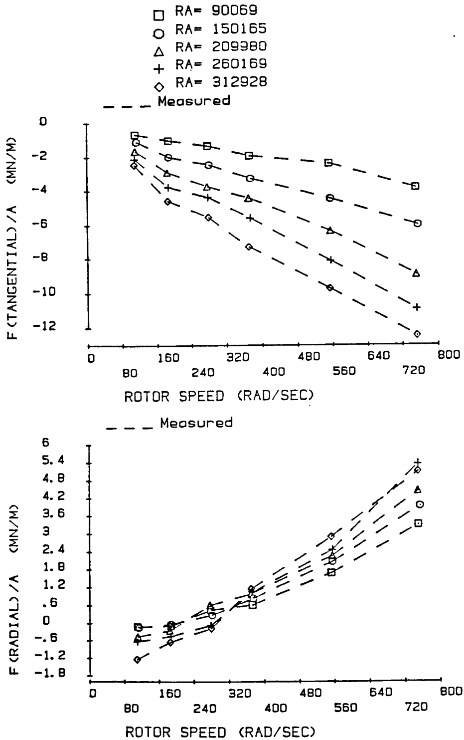
Figure 42. F_r/A and F_\theta/A for helically-grooved-stator seal 3, \alpha = 30^\circ .
