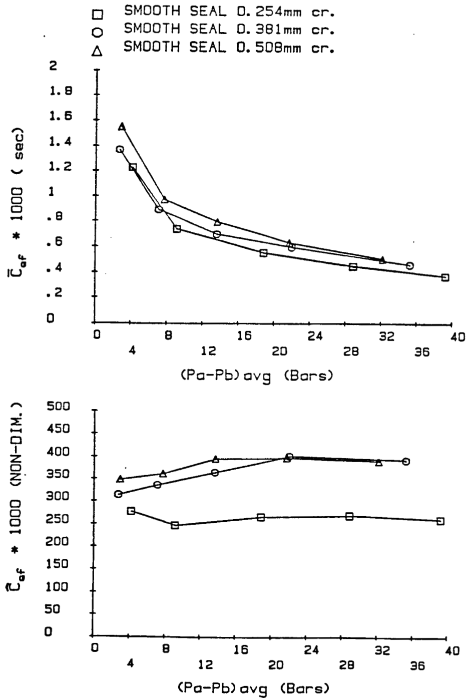
Figure 14. \bar{C}_{ef} and \hat{C}_{ef} versus \Delta P for smooth seals at three different clearances.
