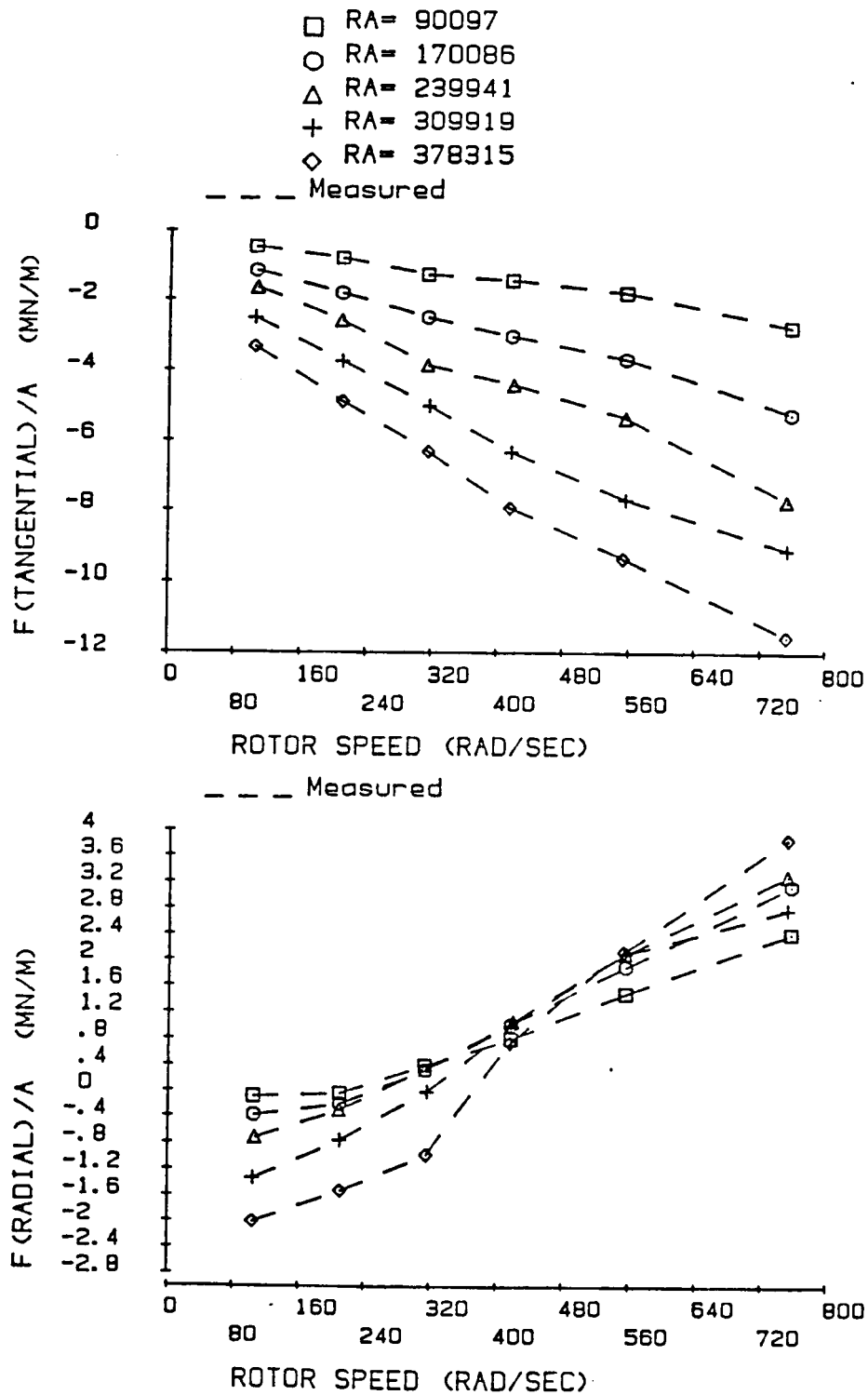
Figure 44. F_r/A and F_\theta/A for helically-grooved-stator seal 5, \alpha = 40^\circ .
