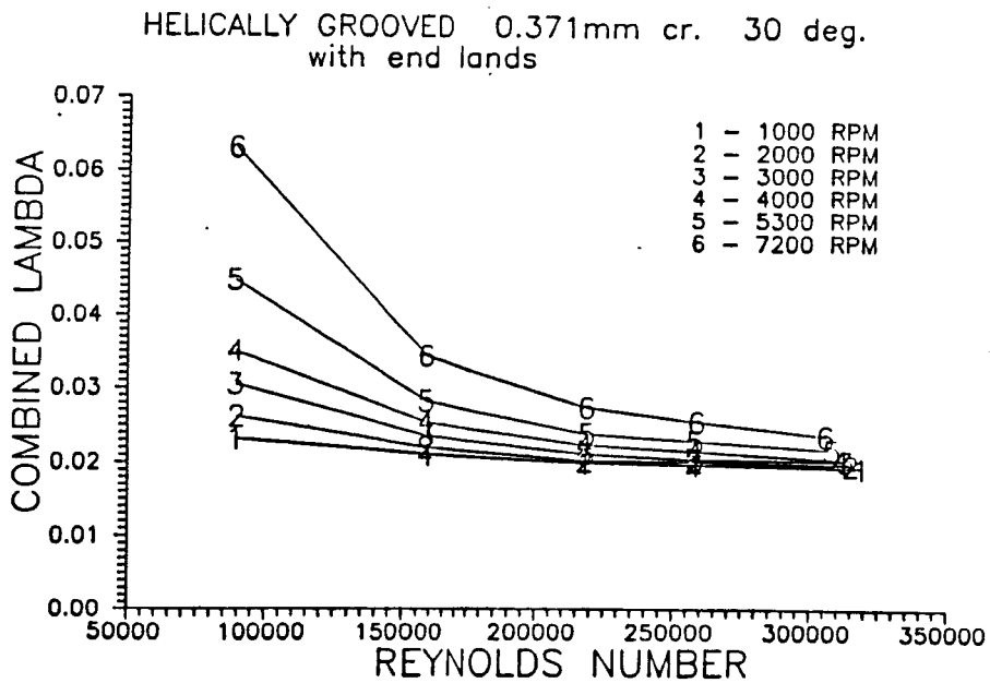
Figure 35. Combined-lambda, \lambda_c , data for helically-grooved-stators 3 and 4 versus R_a and \omega .
