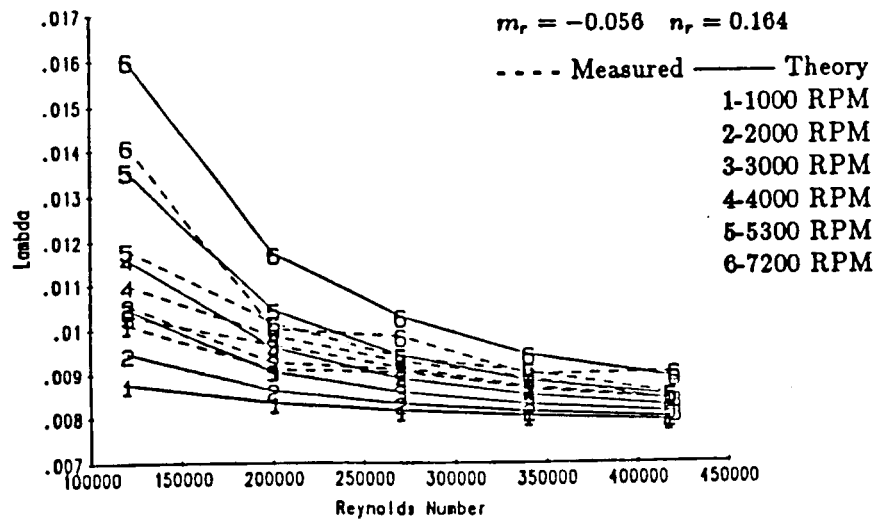
Figure 7. Measured and theoretical values for \lambda versus Reynolds number and running speed for seals with a smooth stator and a smooth eccentric rotor; C_r = 0.254, 0.381, 0.508mm .
