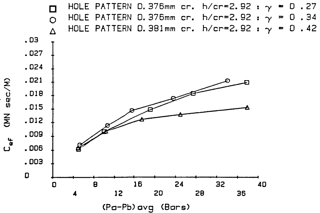
Figure 31. C_{ef} for hole-pattern stators 1 through 6.
