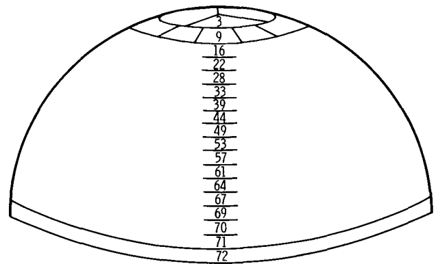
Figure 1. Igloo grid system for near-equal-area grids. Number of grids in each 5° latitude region for one hemisphere is shown.
