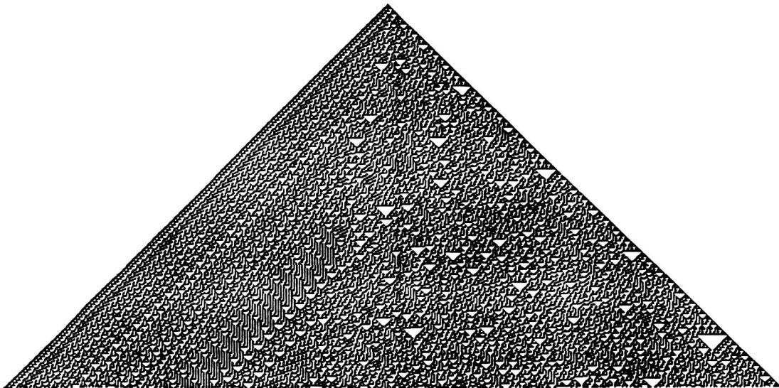
Figure 3: Pattern generated by a one-dimensional cellular automaton with two possible values at each site, and rule a'_i = (a_{i-1} + a_i + a_{i+1} + a_i a_{i+1}) , starting from a single nonzero site. Despite the simplicity of its specification, many aspects of the pattern seem random. For example, the center column of site values passes all standard statistical tests of randomness. This cellular automaton illustrates the rather general phenomenon that simple processes can lead to complexity that is so great that many aspects of it seem random.
