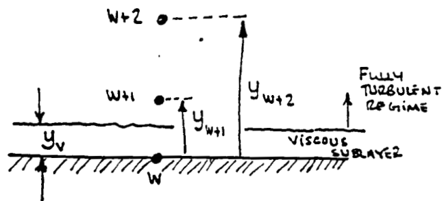
Figure 4. Near-wall region for low-Reynolds-number k-\epsilon calculations or wall functions.
