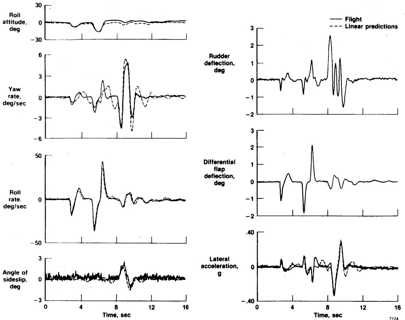
Fig. 11 Response of the X-29A to a differential flap and rudder input compared with linear simulation results.
