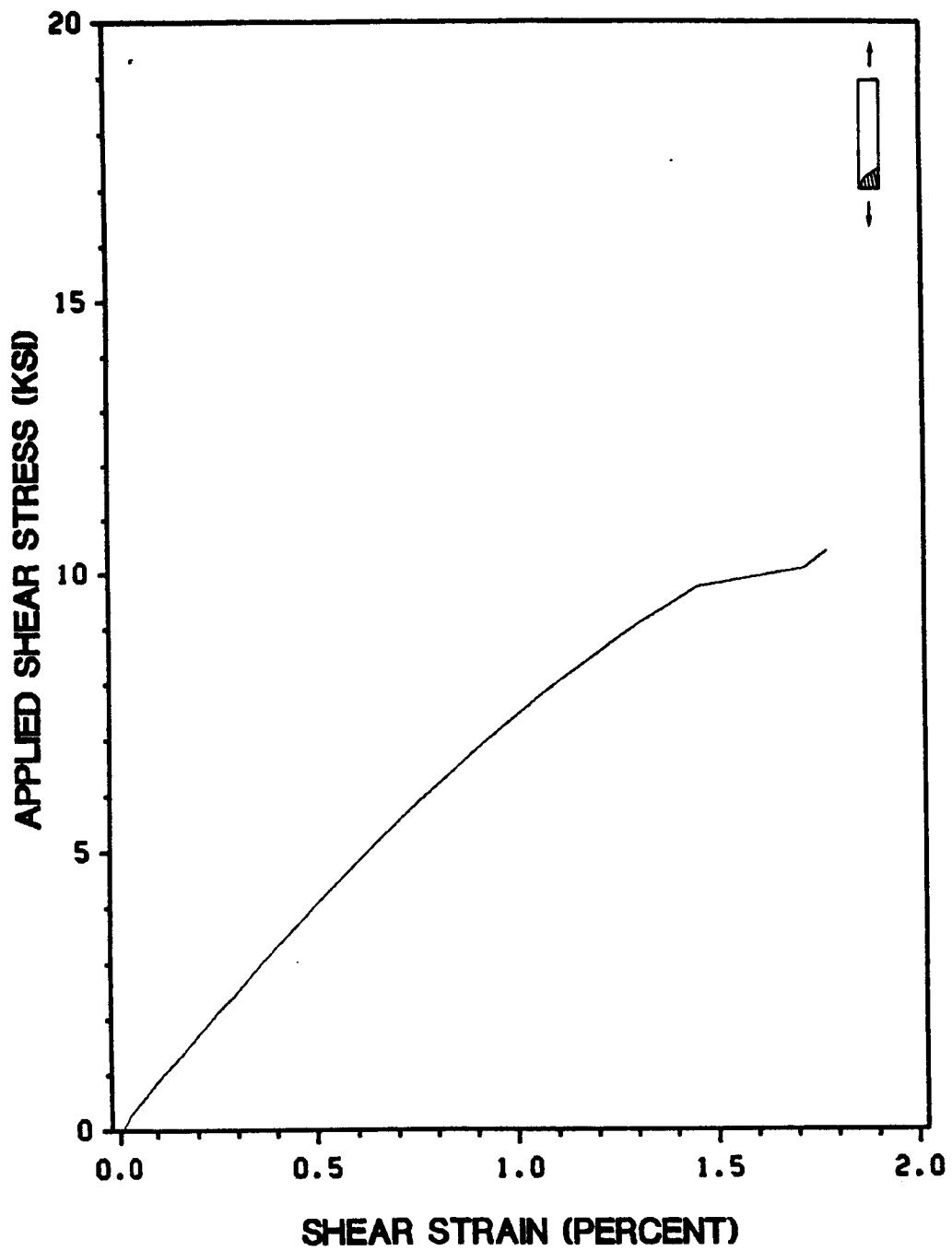
Figure 66. Shear Stress vs. Shear Strain for a Typical 10° Off-Axis Tensile Test: AS4/3501-6 Graphite-Epoxy, Shear Coupling Effects Not Included
