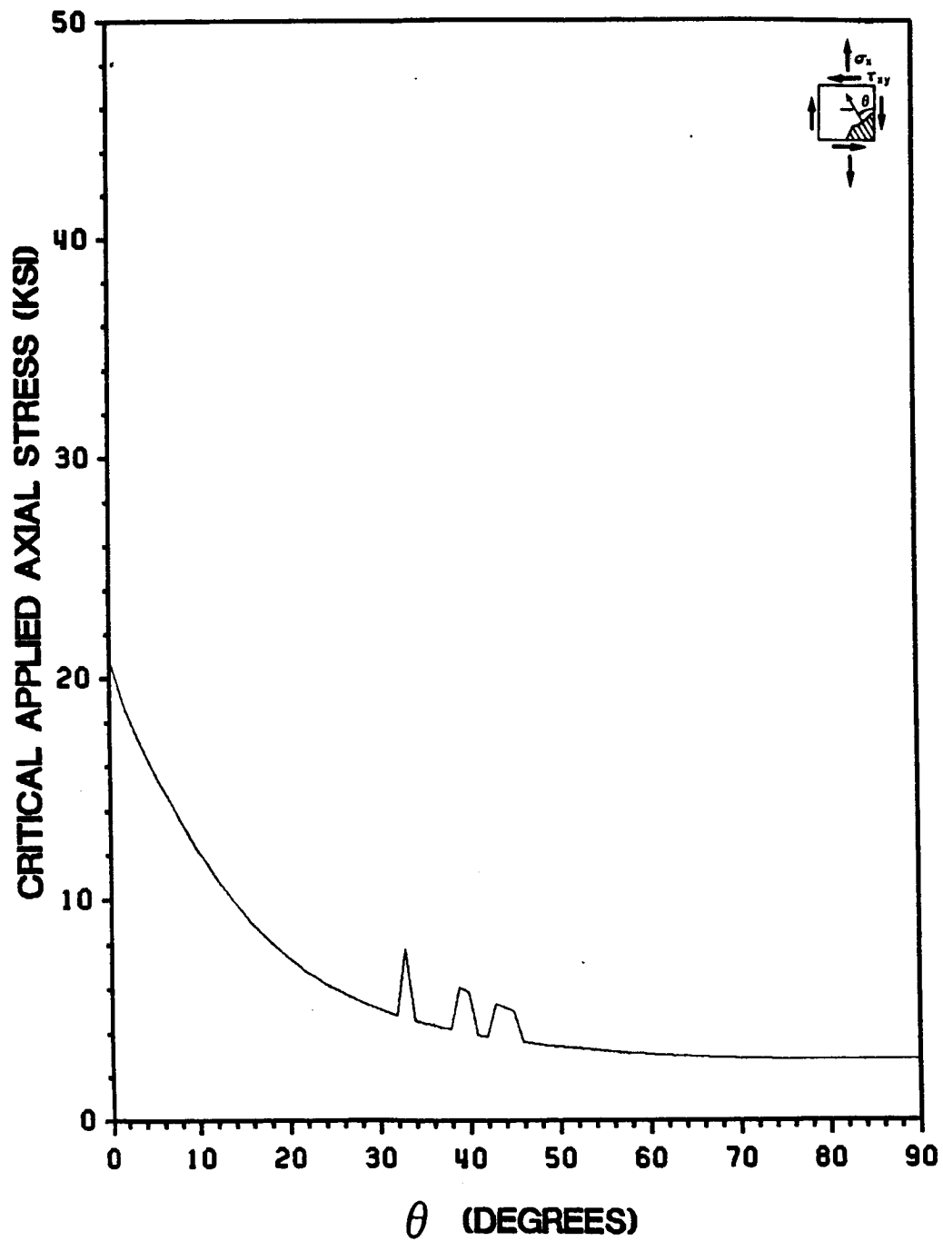
Figure 57. Predicted Critical Axial Stresses vs. Fiber Angle for Tensile Coupons with Horizontal Center Notches: Shear Coupling Effects Included, AS4/3501-6 Graphite-Epoxy
