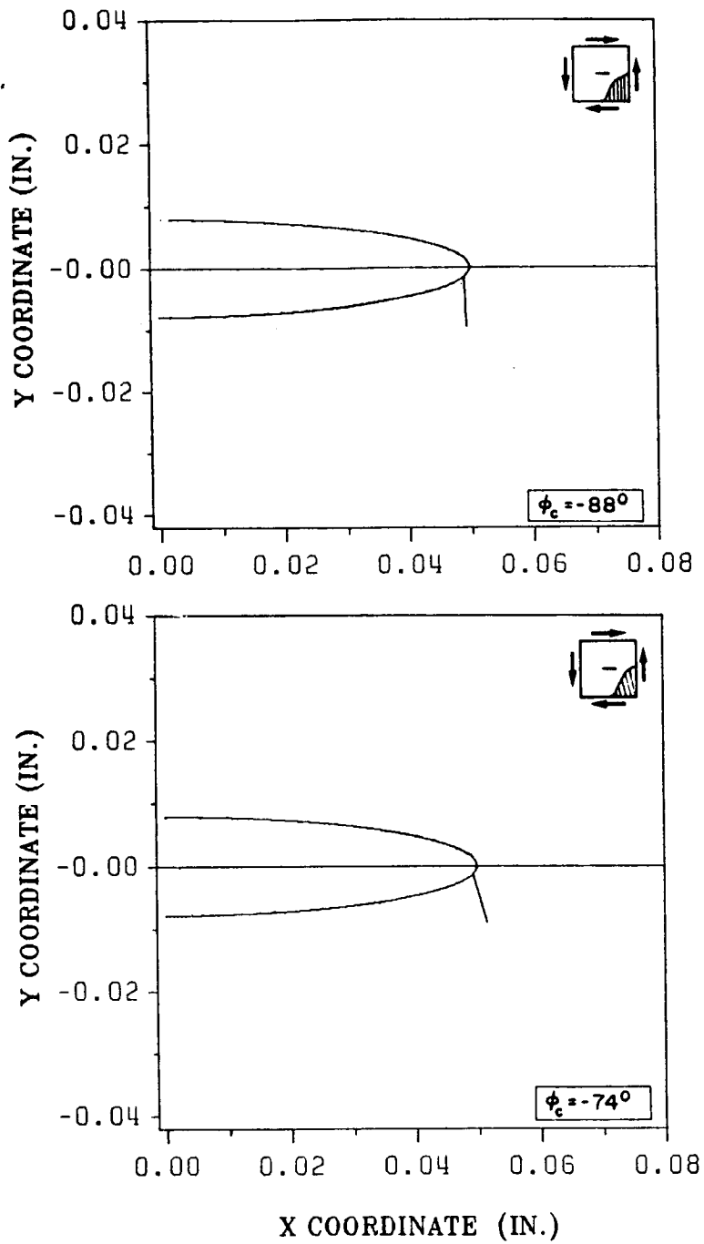
Figure 62. Predicted Locations of Crack Initiation for 0^\circ and 15^\circ Iosipescu Shear Specimens
