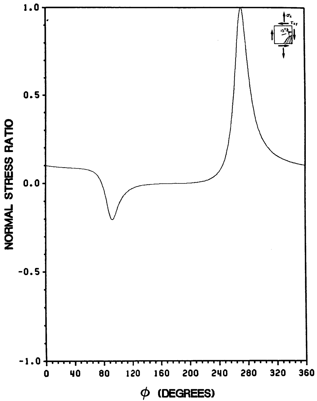
Figure 8. Normal Stress Ratio vs. \phi : 15^\circ Off-Axis Tensile Coupon, AS4/3501-6 Graphite-Epoxy, Aspect Ratio = 8, 105^\circ Notch
