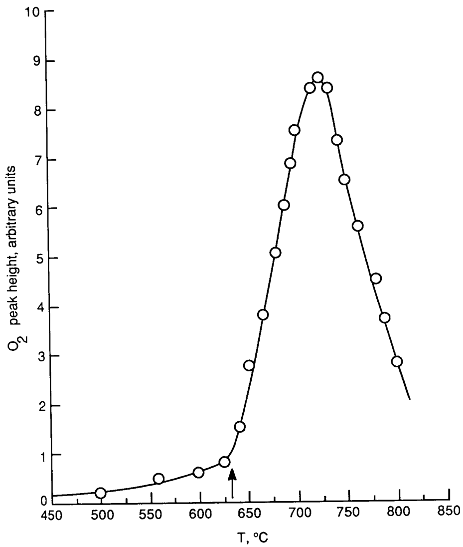
Figure 8. Vacuum desorption of oxygen from Ag membrane for dT/dt = 4\text{K}/\text{min} . Arrow indicates onset of vacuum desorption.
