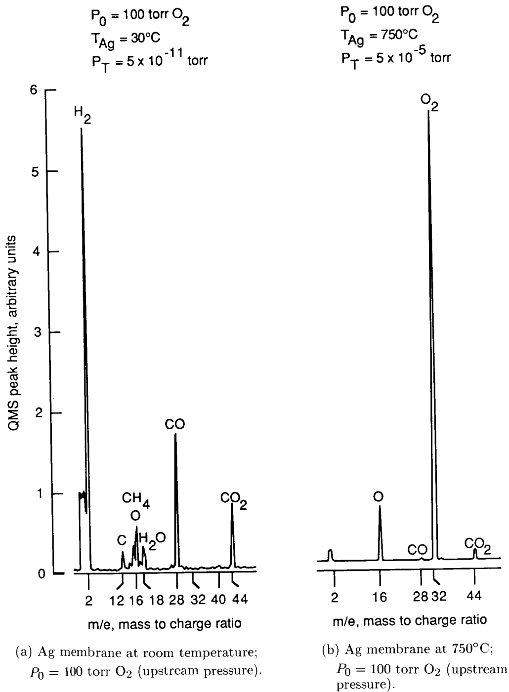
Figure 4. QMS spectra of system.
