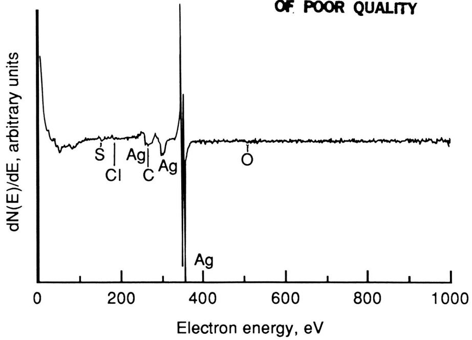
(a) AES survey of Ag membranes after polishing and chemical cleaning.
