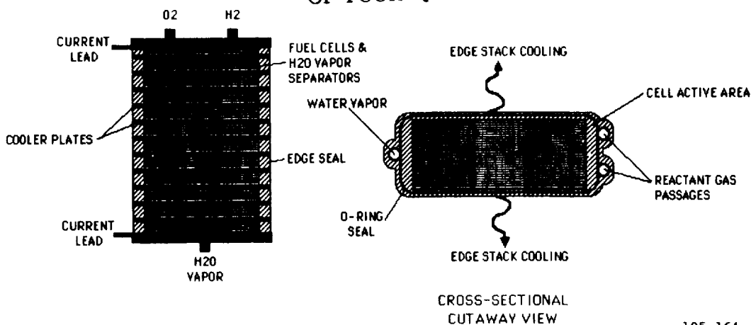
Figure 27. Alkaline Fuel Cell Stack
