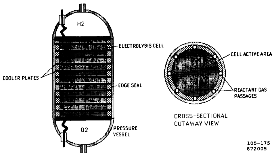
Figure 38. PEM Electrolysis Cell Stack
