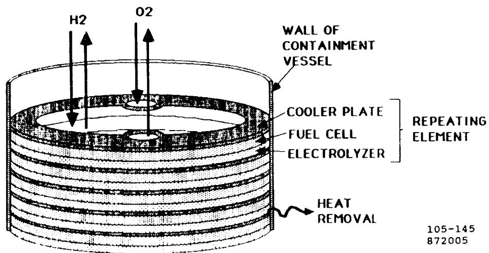
Figure 6. Cell Stack Cutaway Sketch
