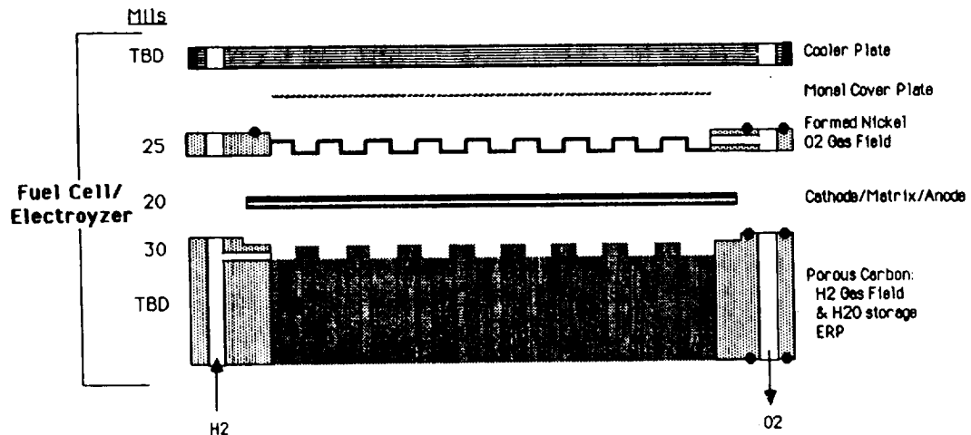
Figure 44. Cell Detail - Dual Function Alkaline Fuel Cell/Electrolyzer
