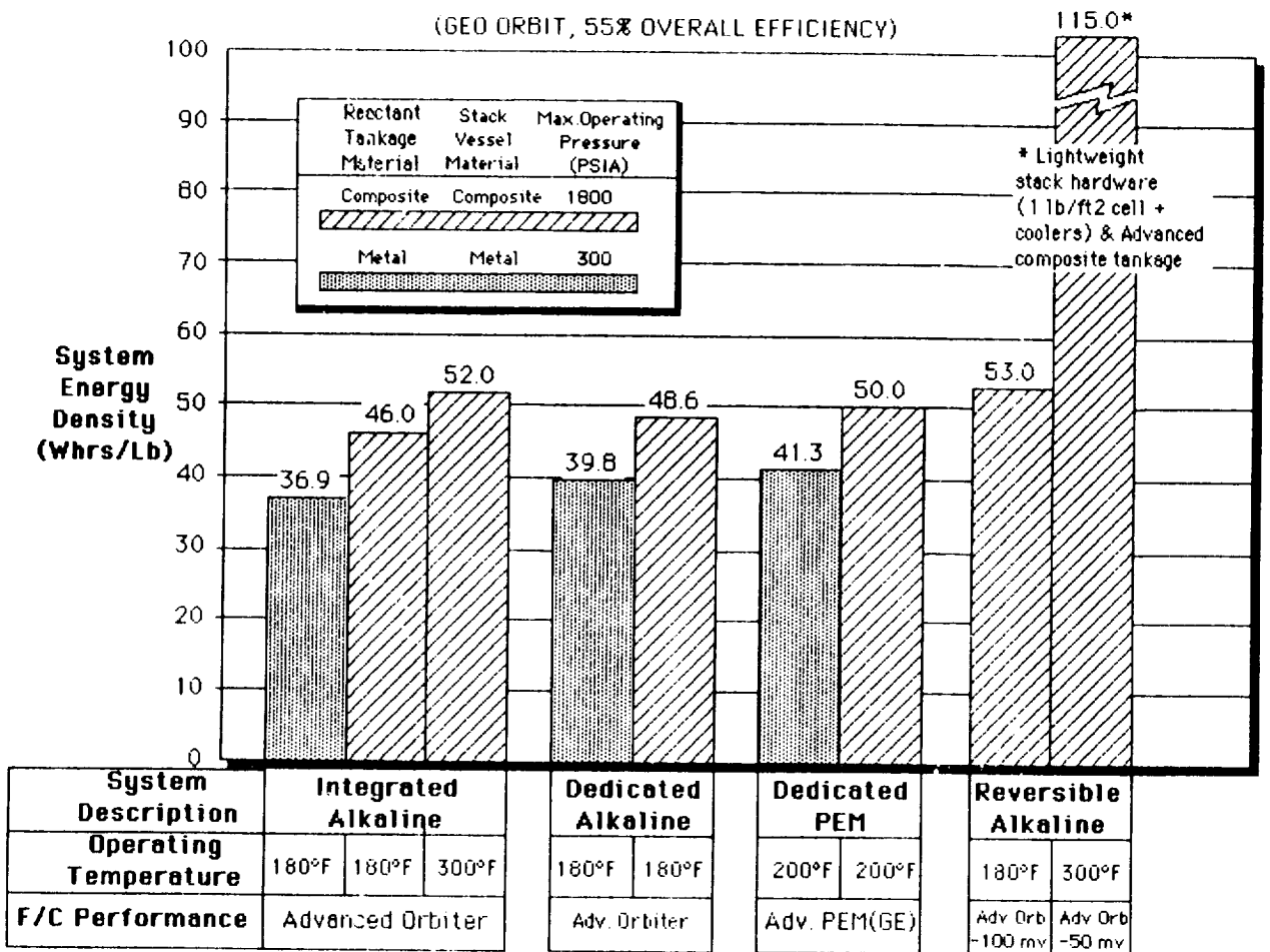
Figure S-1. Energy Density Results for Systems Studied
