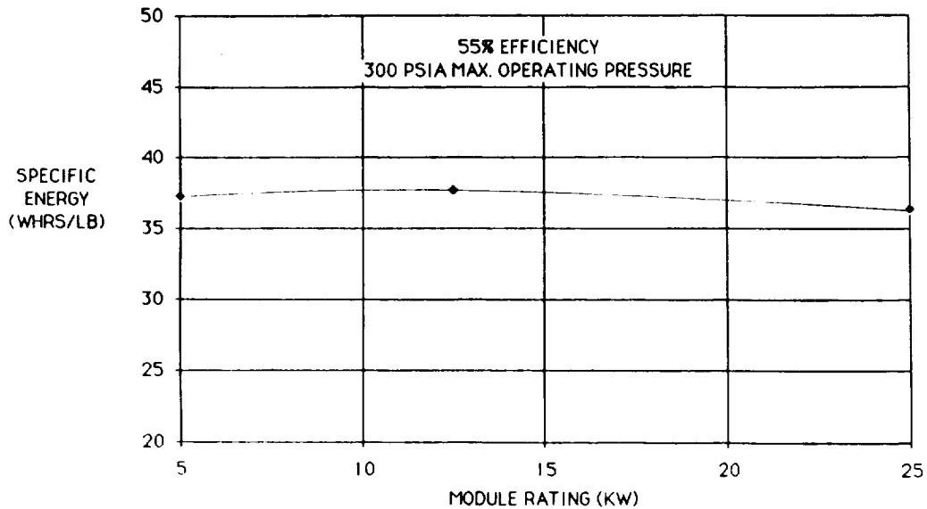
Figure 18. Effect of Module Power Rating
