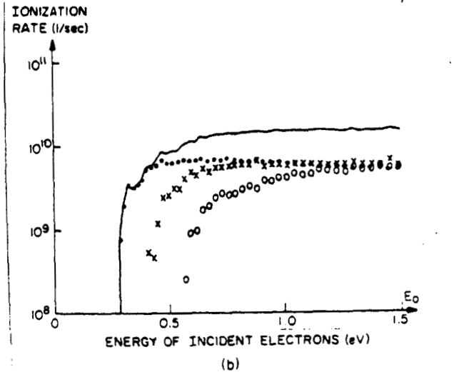
FIG. 3. (a) The impact ionization rate (1/\tau(E_0)) as a function of the incident electron energy E_0 measured from the conduction-band edge of the AlGaAs region using the analytical approximation (12) in Eq. (4). (circles = first subband, crosses = second subband, dashed line = total.) (b) 1/\tau(E_0) calculated using direct numerical integrations of multiple integrals as has been done in Fig. 4(b) of Ref. 8.
