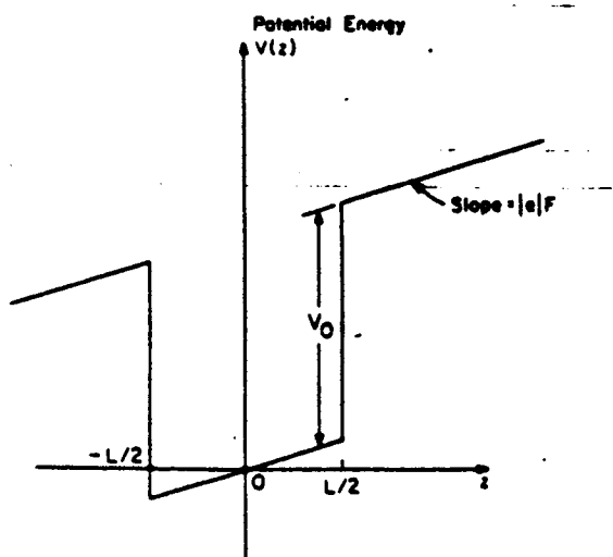
FIG. 1. Potential-energy profile V(z) for a single quantum well with depth V_0 and width L subject to an external electric field F .
