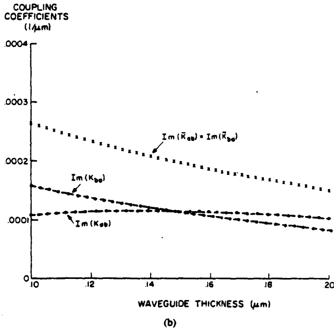
Fig. 5. (a) The real parts, and (b) the imaginary parts of the coupling coefficients K_{ab} and K_{ba} for the waveguide system in Fig. 3 are plotted versus the thickness ( \mu\text{m} ) of waveguide b . Our results (dashed lines) and the results using [3] (dotted lines) are on top of each other. The crosses are the results using [2].
