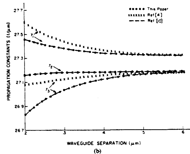
Fig. 4. (a) A comparison of the propagation constants of the three supermodes between the exact results (solid lines) and the results of this paper (dotted lines) for the three coupled waveguides in Fig. 3. (b) A comparison with other two methods: results using [10] (dashed lines), results using [4] (crosses). The results of this paper are given by dotted lines.
