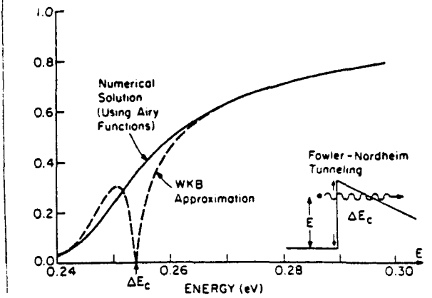
FIG. 4. The transmission coefficient for electron tunneling through a triangular barrier with a height \Delta E_c = 0.254 eV. The solid curve is using the numerical approach with Airy functions and their derivatives. The dashed curve is from the WKB method.
