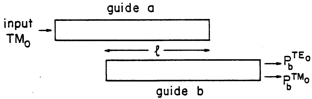
Directional Coupler 2
