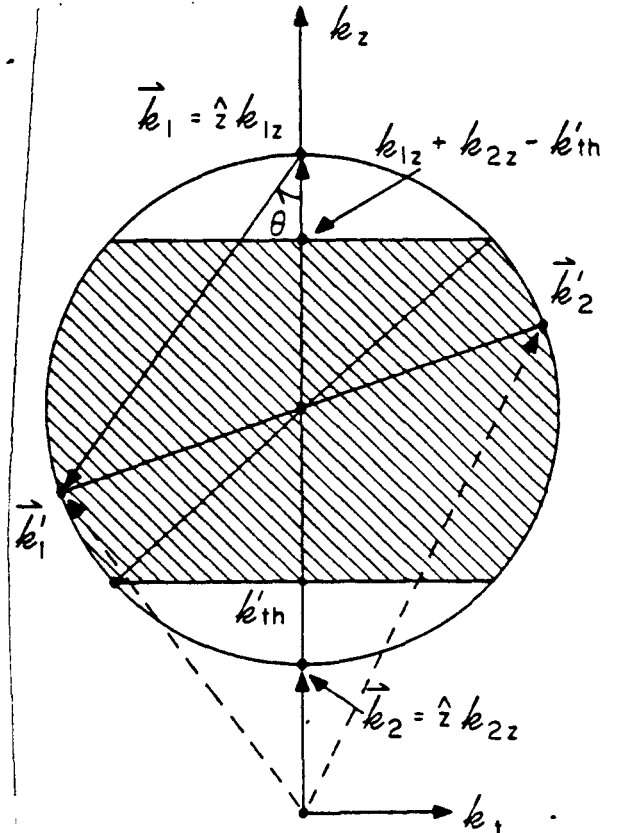
FIG. 2. A momentum space diagram illustrating the range of integrations for k'_1 . Because of both energy and momentum conservation, the four wave vectors k_1 , k_2 , k'_1 , and k'_2 lie on a spherical surface in the momentum space assuming parabolic band structures.
