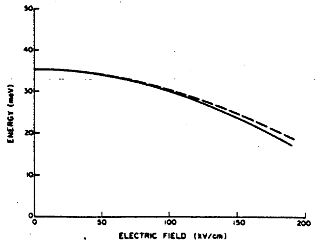
FIG. 2. Comparison of the ground-state energy of the variational calculation (Refs. 13 and 15) for infinite-well with appropriate effective-well width (dashed line) and the real part of the energy eigenvalue E_0 from exact calculation (solid line) of this paper.
