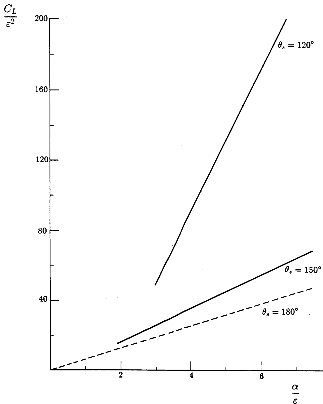
Figure 7.4 Lift vs. relative incidence for various separation angles on a circular cone.
