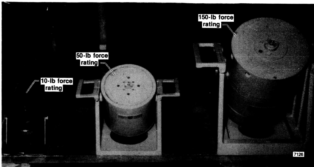
Fig. 1 Electrodynamic shakers.
