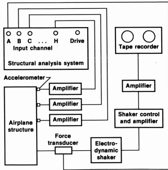
Fig. 7 Schematic of the minicomputer-based structural analysis system for random excitation and data acquisition.
