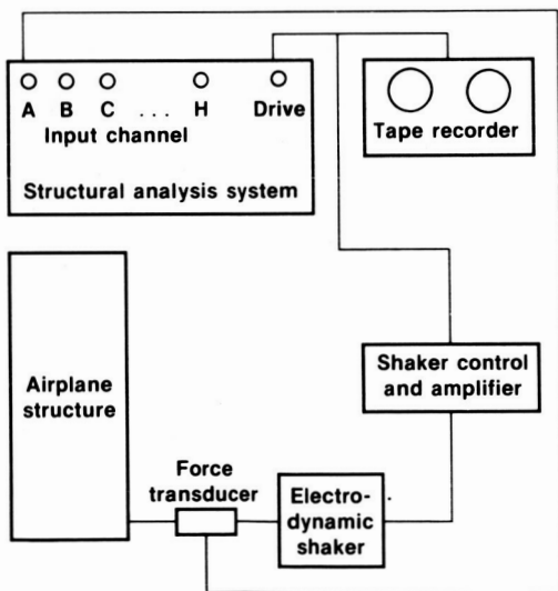
Fig. 6 Schematic of the minicomputer-based structural analysis system for forcing-function generation.
