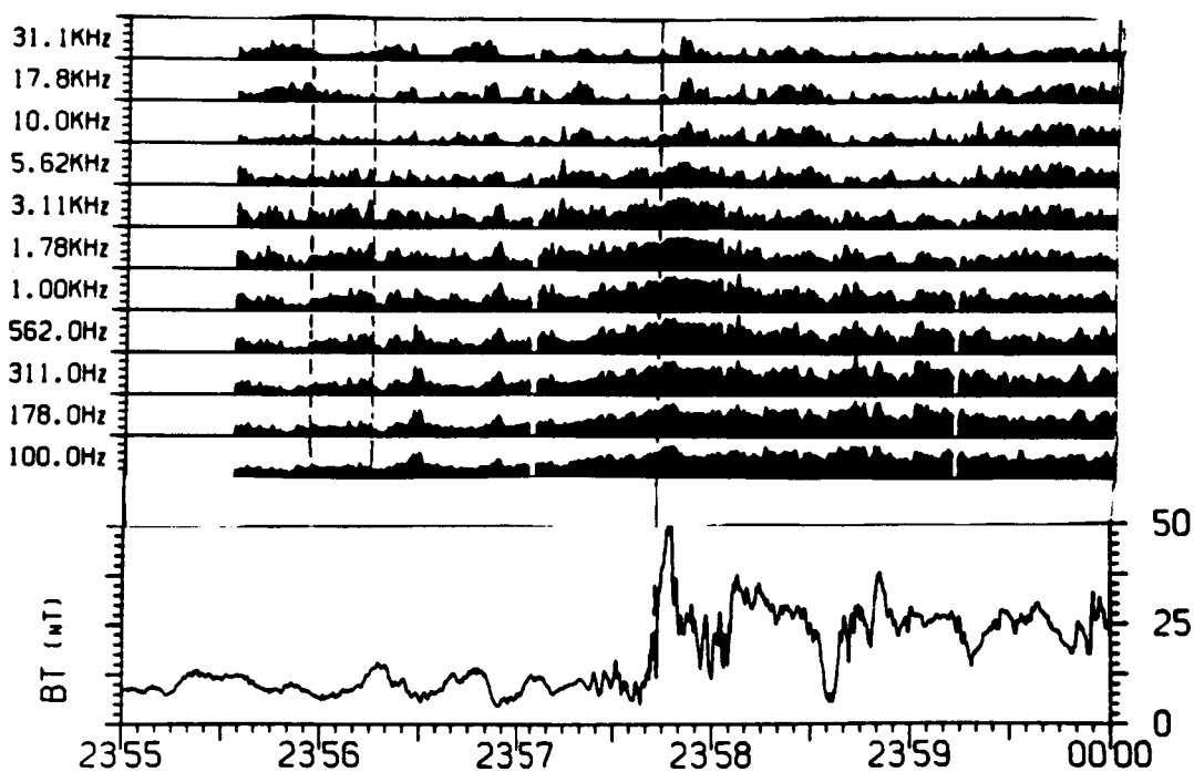
Figure 2. Quasiparallel Bow Shock: Plasma Wave Profile.
