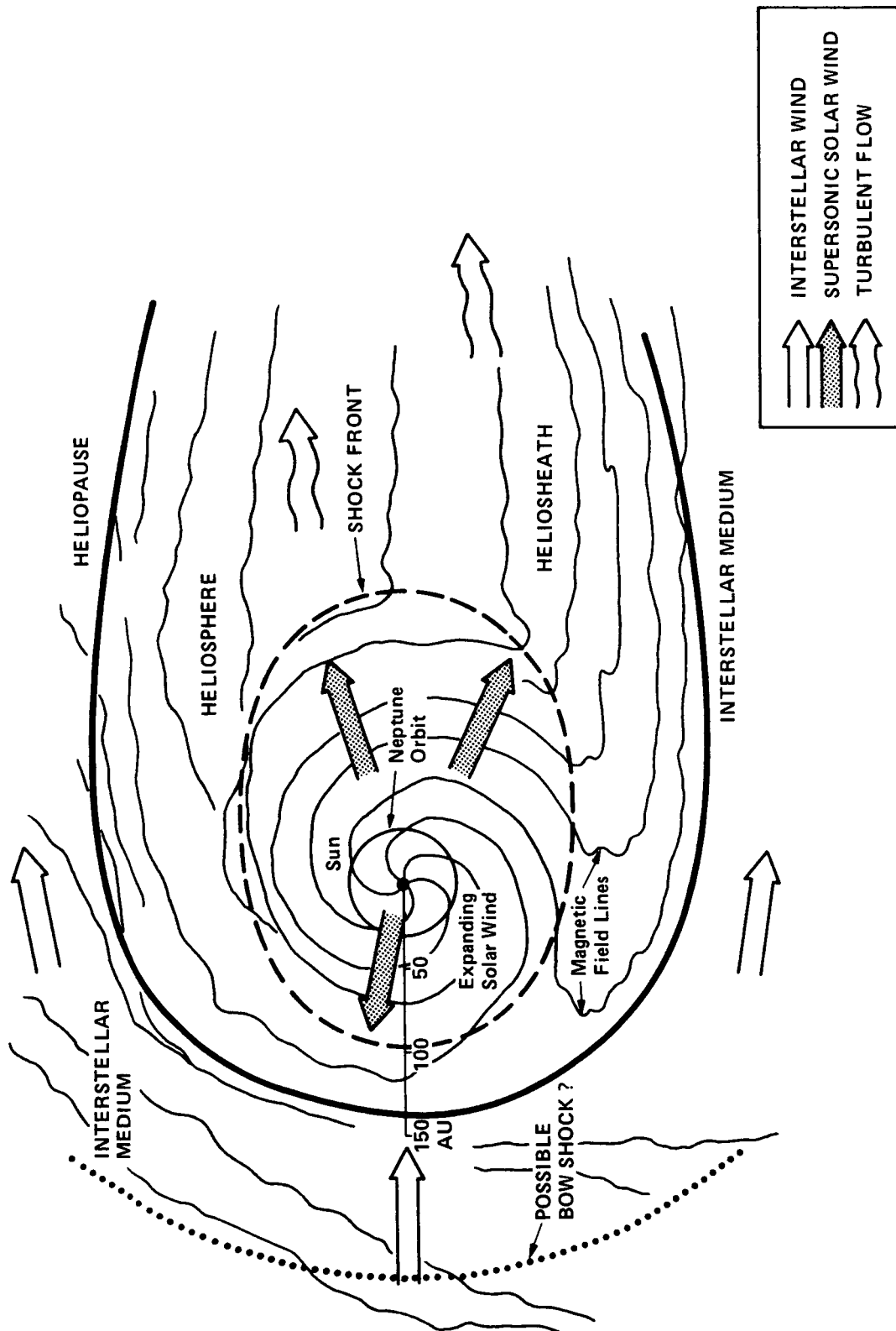
Figure 4. Probable Model for Heliosphere
