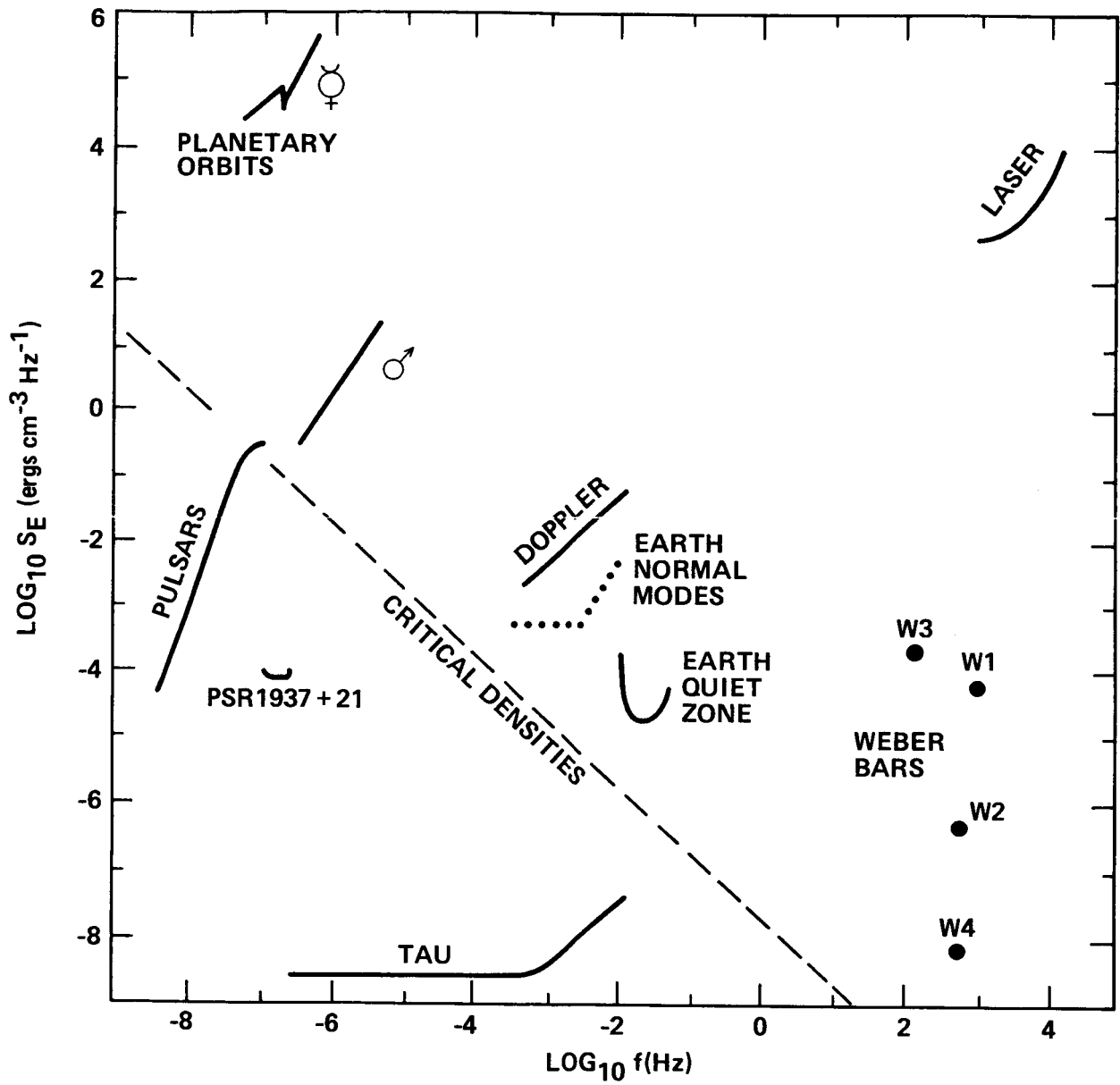
Figure 3. Gravity Wave Detection Limits
