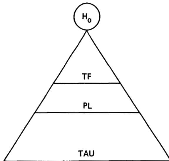
Figure 2. Comparison of Current Method of Determining the Hubble Constant With Method Available With TAU
