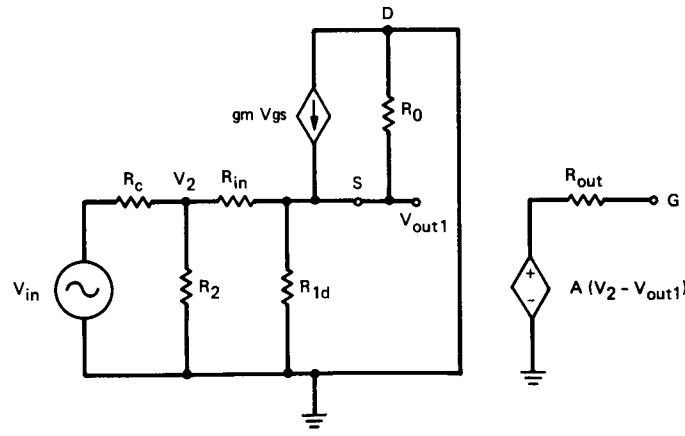
Fig. 4. Small signal model with AC source on anode of constant diode ( R_c )
