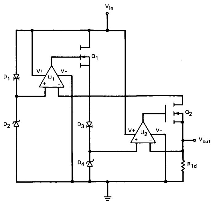
Fig. 3. Two staged FET circuit
