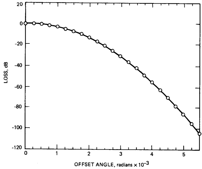
Fig. 3. Connector coupling loss as a function of the angular offset
