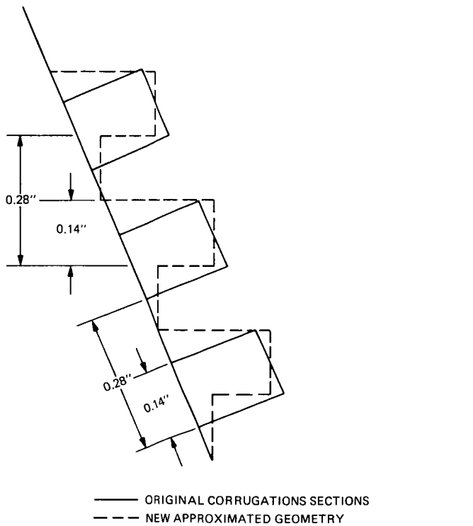
Fig. 2. Approximation of the standard JPL feedhorn corrugations by cylindrical sections
