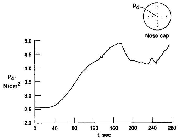
(h) Pressure measured at orifice 4.
