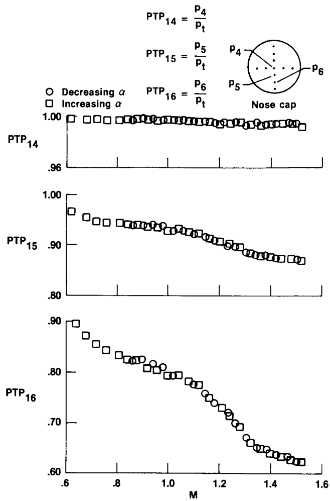
Figure 14. Stagnation pressure parameter as a function of Mach, \alpha = 0.0^\circ to 5.9^\circ .
