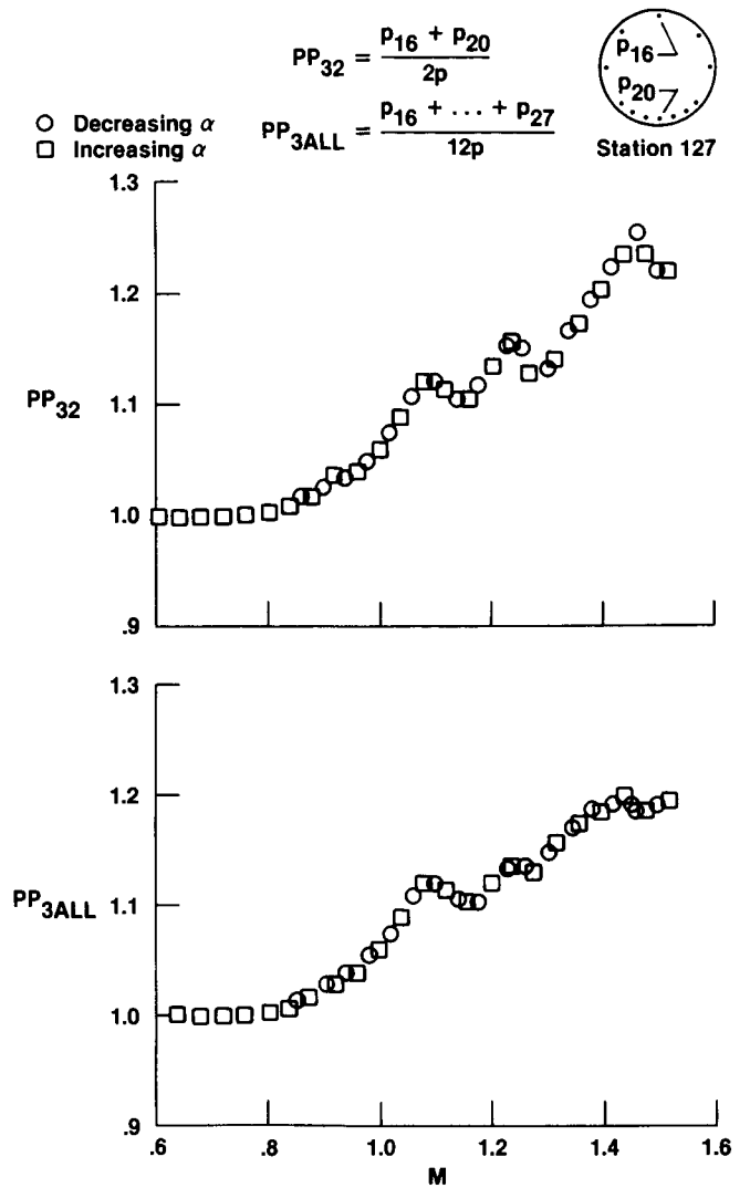
(b) Orifices at station 127.
