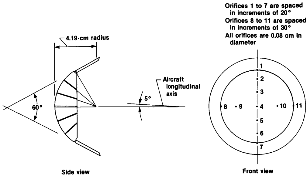
Figure 5. Sectional views of FADS nose cap.
