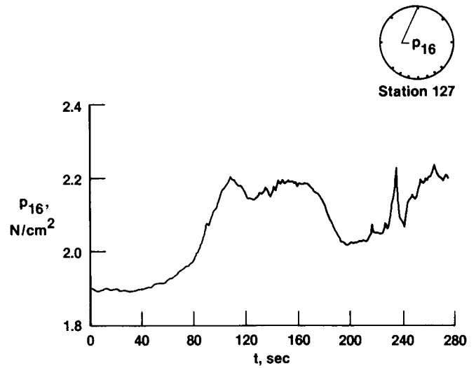
(r) Pressure measured at orifice 16.
