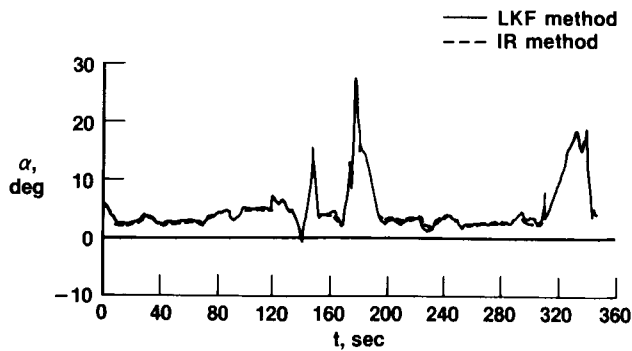
(c) Angle of attack.
