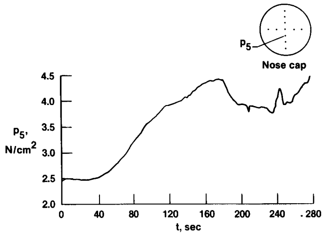
(i) Pressure measured at orifice 5.
