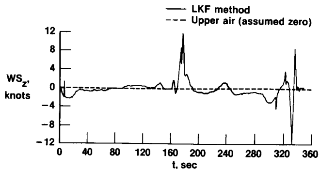
(f) Vertical windspeed.
