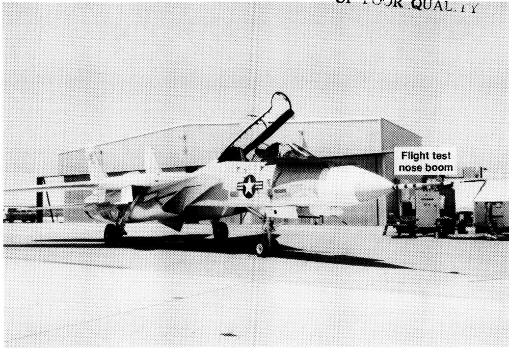
Figure 1. F-14 airplane with flight test nose boom.
