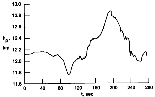
(b) Reference pressure altitude.
