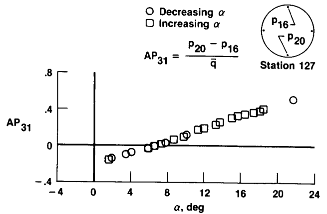
(f) M = 0.90 , orifices at station 127.
