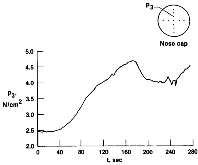
(g) Pressure measured at orifice 3.
