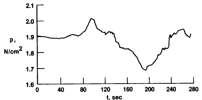
(f) Reference static pressure.
