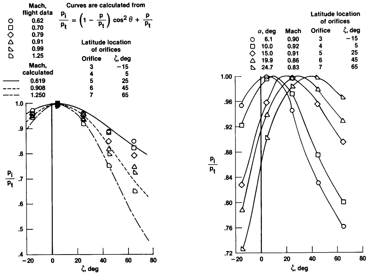
(b) Effect of angle of attack.
