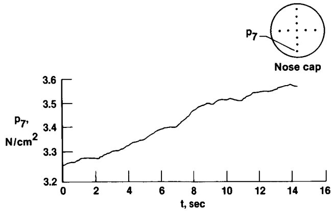
(e) Pressure measured at orifice 7.
