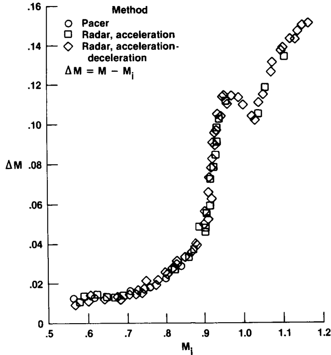
Figure 27. Typical results of Mach correction for static-pressure position error of IR reference probe as a function of indicated Mach, \alpha = 1.7^\circ to 2.7^\circ .
