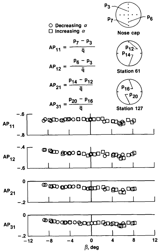
Figure 21. Effect of sideslip on angle-of-attack parameter, M = 0.90 and \alpha = 4.0^\circ .
