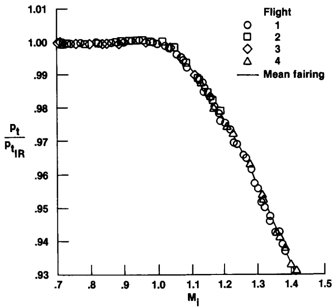
Figure 31. Ratio of stagnation pressure of nose boom to stagnation pressure of IR reference probe as a function of indicated Mach, \alpha < 10.0^\circ .
