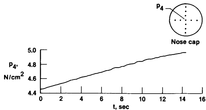
(b) Pressure measured at orifice 4.
