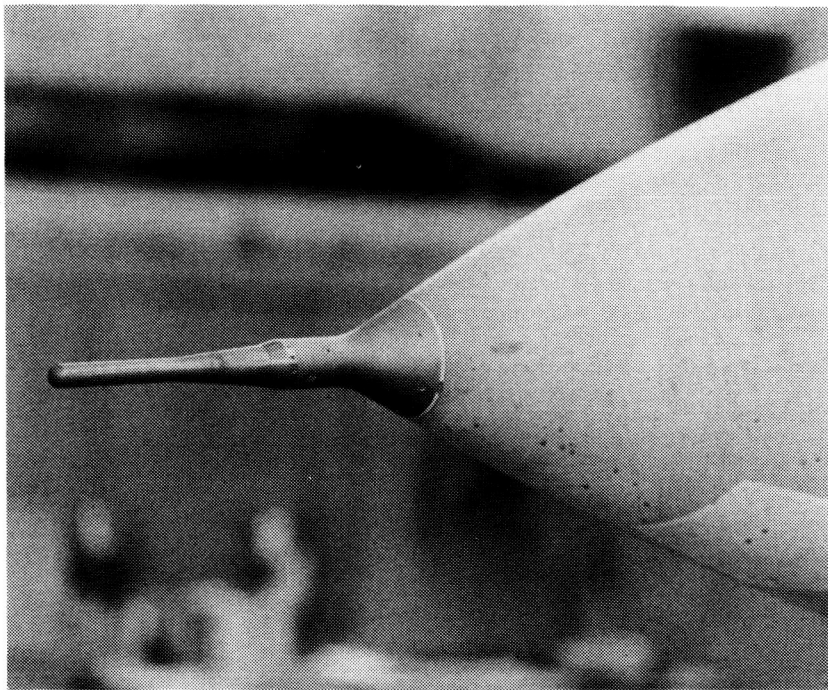
Figure 3. Hemispherical flow direction probe.
