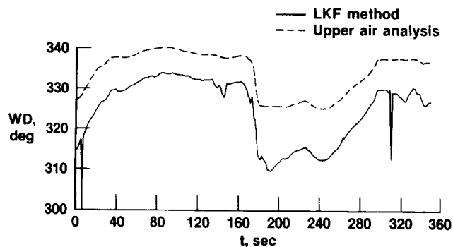
(h) Wind direction.
