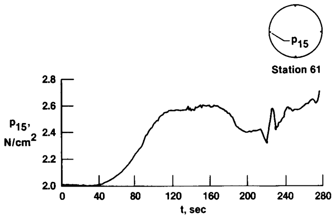
(q) Pressure measured at orifice 15.
