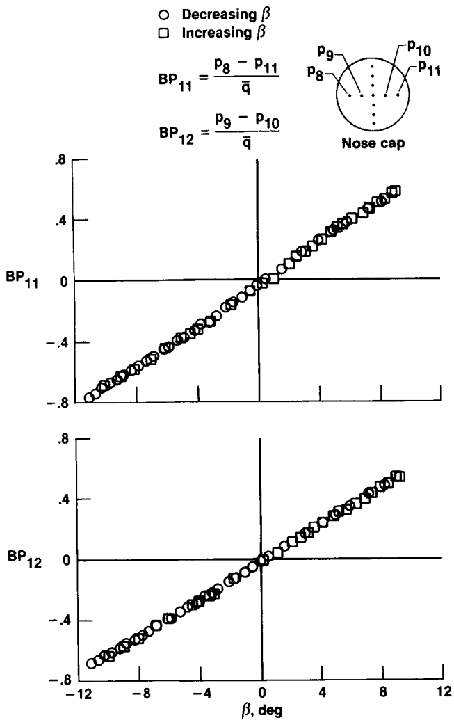
(a) M = 0.77 , \alpha = 1.9^\circ to 3.6^\circ , orifices on nose cap.
