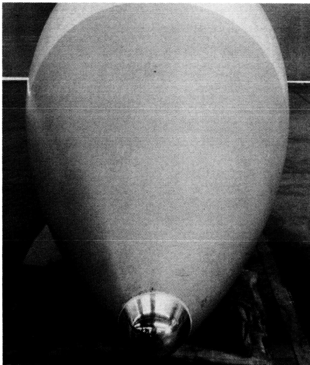
Figure 4. FADS nose cap blended with F-14 nose cone.
