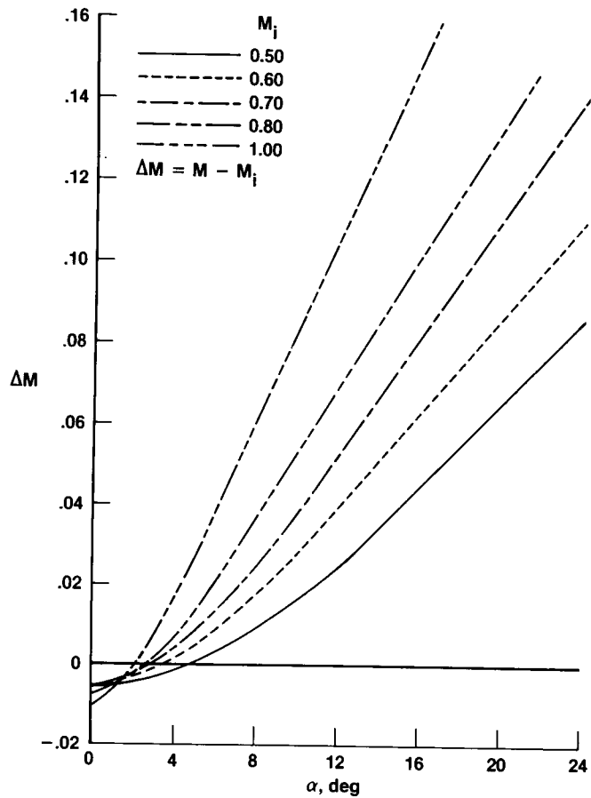
Figure 29. Mach correction for static-pressure position error of IR reference probe as a function of angle of attack at constant indicated Mach.
