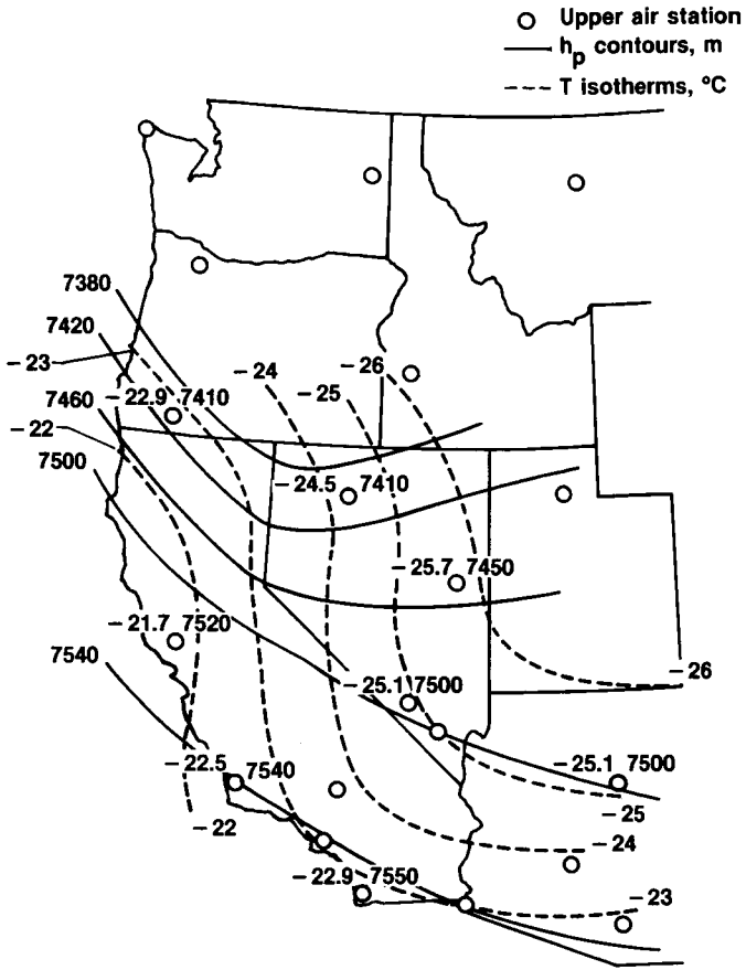
Figure 34. Synoptic meteorological analysis for 400-mbar surface, h_p = 7.19 km.
