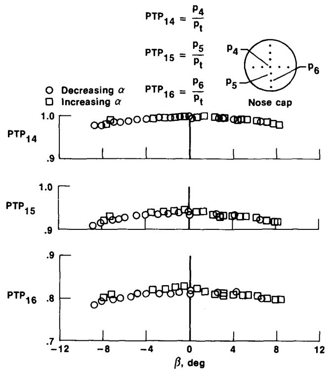
(b) M = 0.87 to 0.92 .
