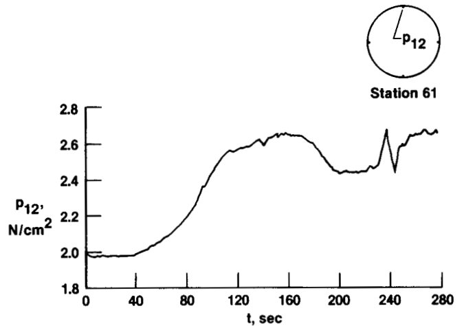
(n) Pressure measured at orifice 12.
