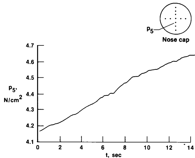
(c) Pressure measured at orifice 5.
