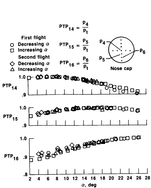
(a) M = 0.57 to 0.68 .
