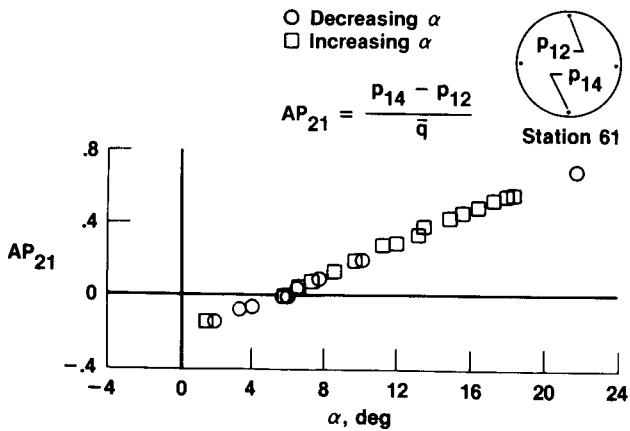
(e) M = 0.90 , orifices at station 61.
