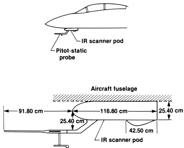
Figure 8. Standard NASA pitot-static probe (ref. 12) installed on IR pod.
