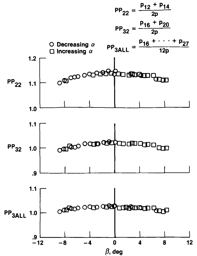
(b) M = 0.87 to 0.92 .
