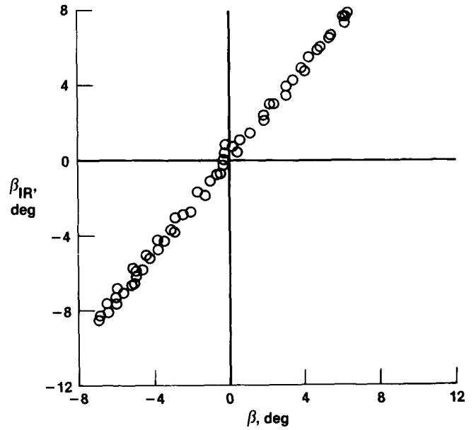
(b) Angle of sideslip, M_i = 0.86 to 0.88 .
