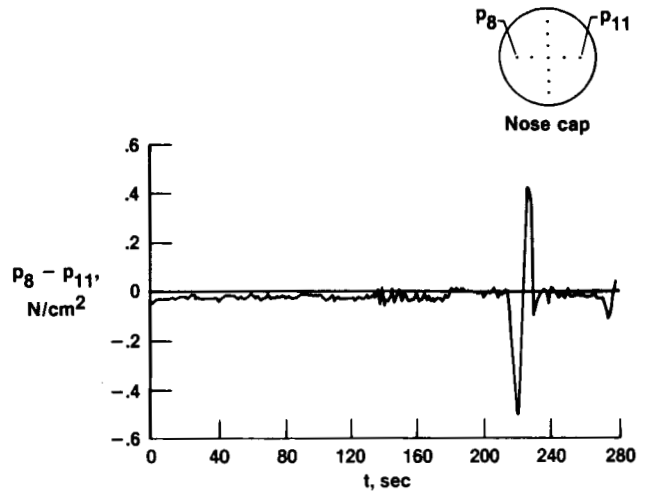
(l) Differential pressure measured between orifices 8 and 11.
