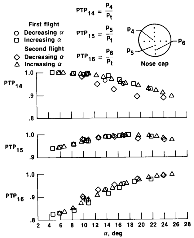
(b) M = 0.87 to 0.92 .
