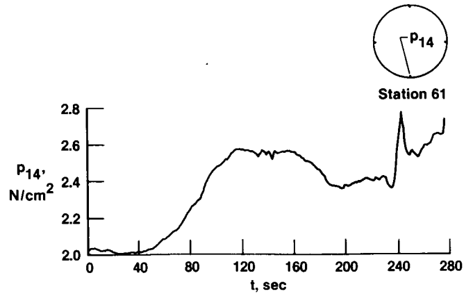
(p) Pressure measured at orifice 14.
