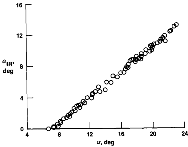
(a) Angle of attack, M_i = 0.53 to 0.63 .
