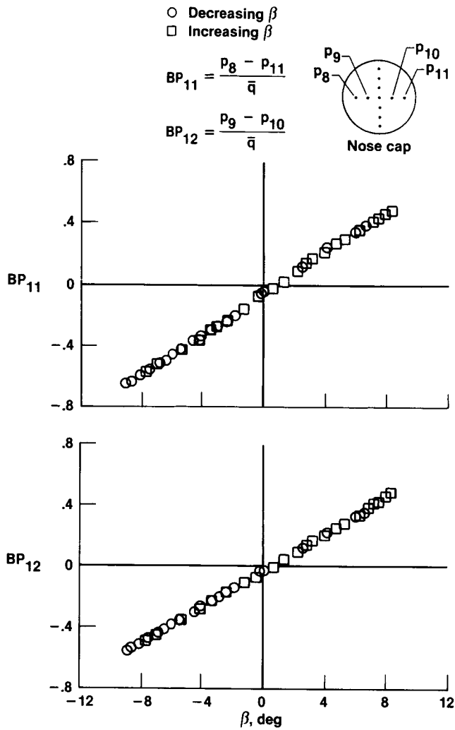
(c) M = 0.89 , \alpha = 3.3^\circ to 5.6^\circ , orifices on nose cap.
