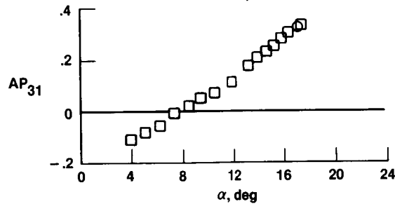
(i) M = 1.23 , orifices at station 127.
