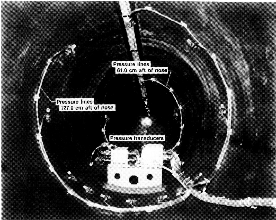
Figure 7. Pressure lines and transducers (looking forward inside nose cone).
