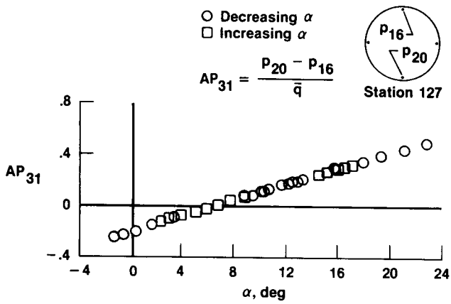
(c) M = 0.60 , orifices at station 127.
