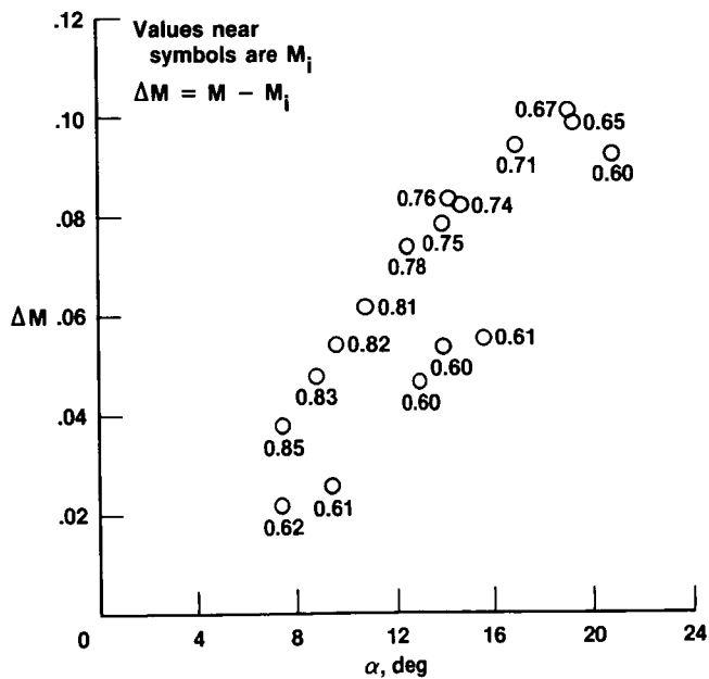
Figure 28. Mach correction for static-pressure position error of IR reference probe as a function of angle of attack for different indicated Mach numbers.
