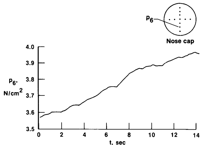
(d) Pressure measured at orifice 6.
