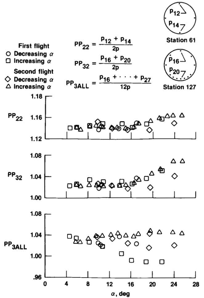
(b) Mach corrected to M = 0.90 ( M = 0.79 to 0.96 , actual range).
