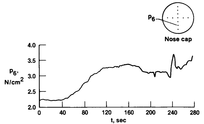
(j) Pressure measured at orifice 6.
