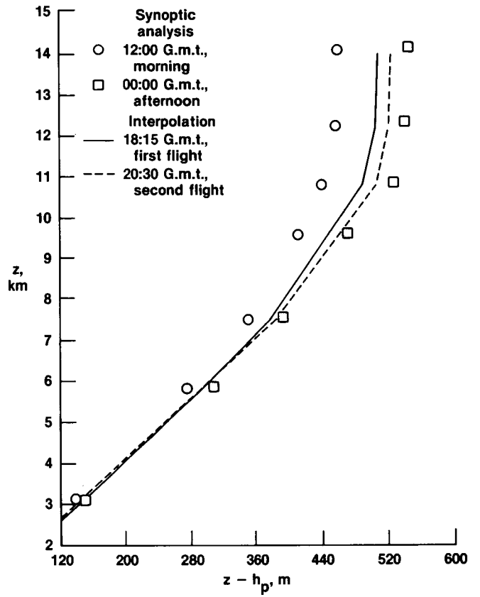
Figure 35. Geometric altitude profile of difference between geometric altitude and pressure altitude.
