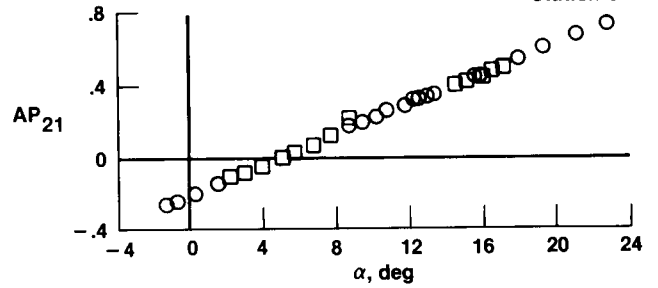
(b) M = 0.60 , orifices at station 61.
