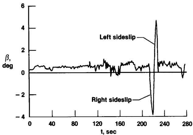
(c) Reference angle of sideslip.
