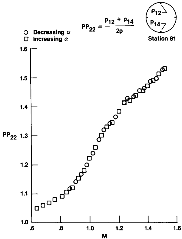
(a) Orifices at station 61.
