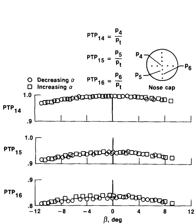
(a) M = 0.75 to 0.80 .
