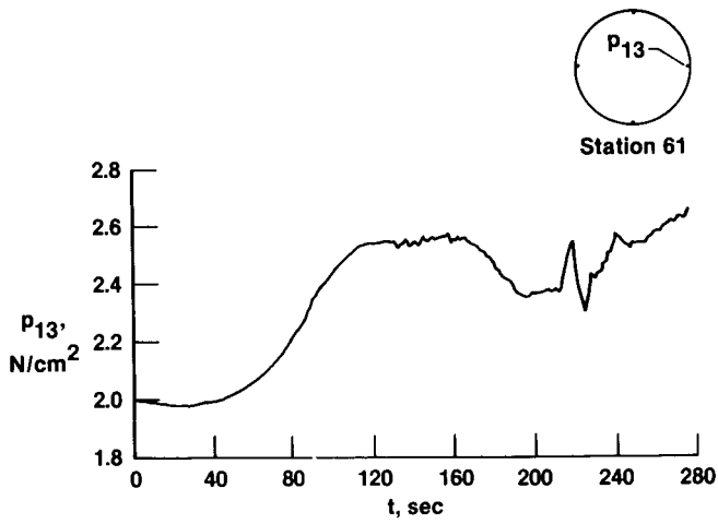
(o) Pressure measured at orifice 13.
