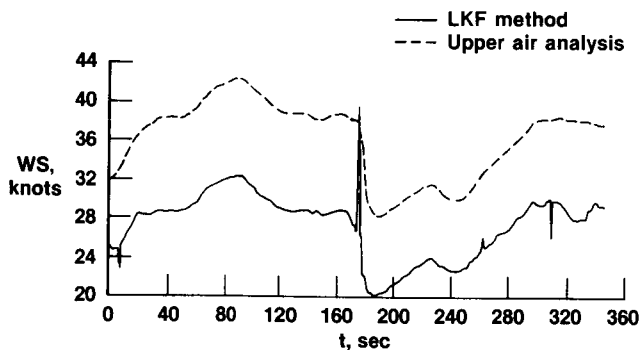
(g) Windspeed.
