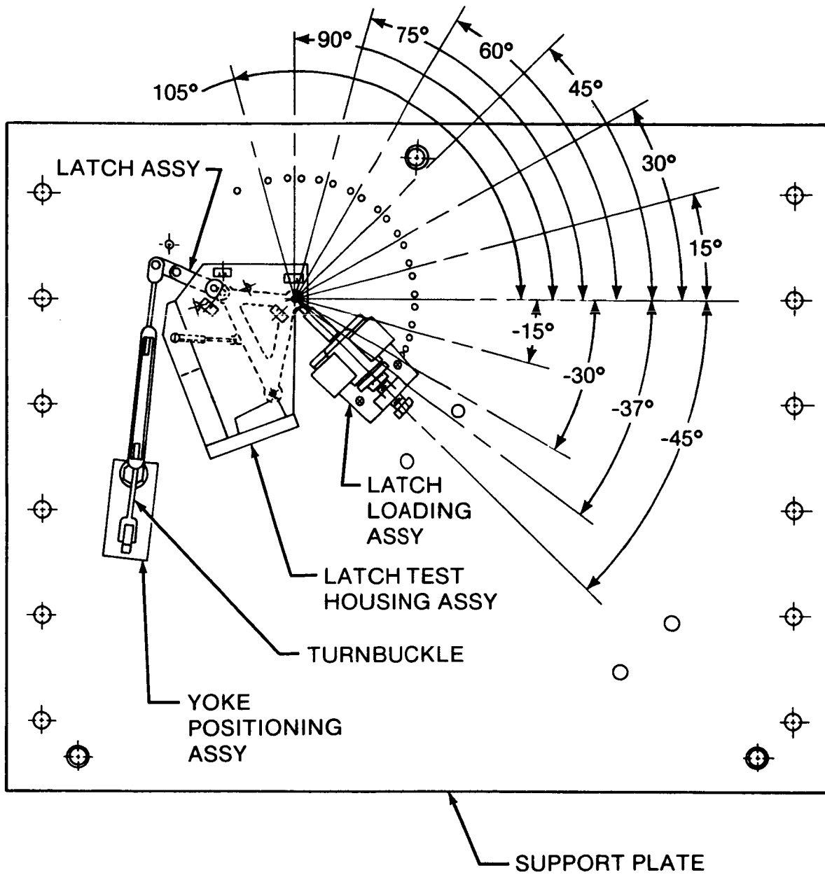
Figure 7. Yoke release position, latch loading.
