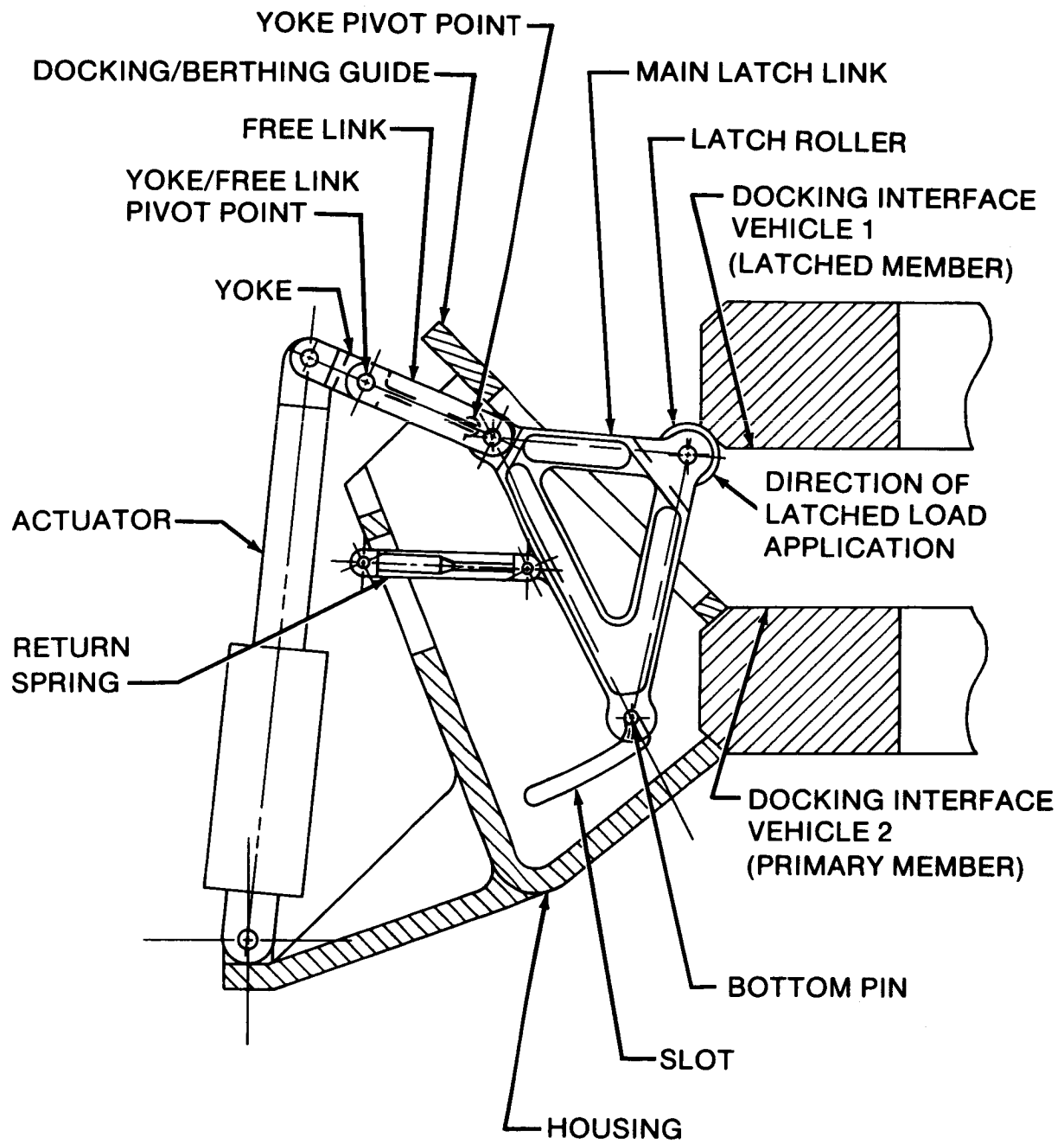
Figure 5. Latch components.
