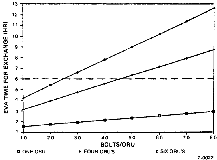
Figure 7. Results of Trade Study on ORU Exchange Times in EVA
