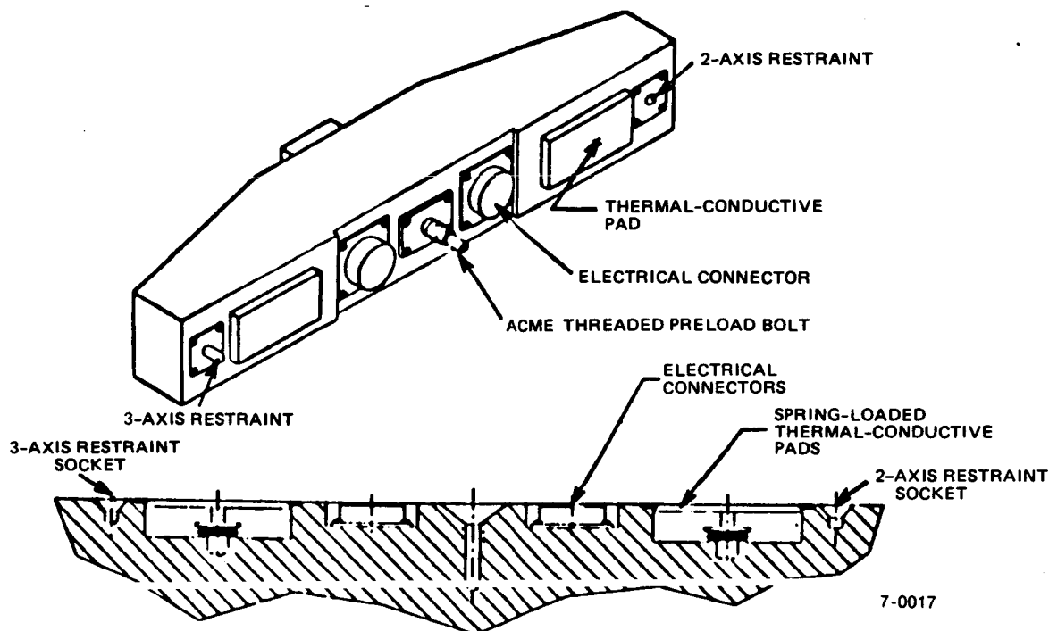
Figure 2. SIC-to-Platform Interface
