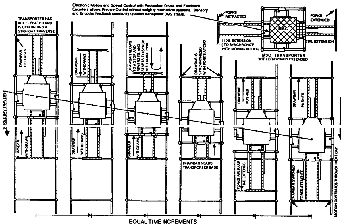
FIGURE 13- MOBILE TRANSPORTER DUAL DRAWBAR PRODUCES CONTINUOUS MOTION
