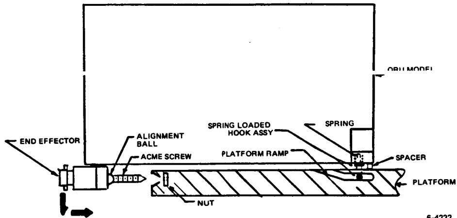
Figure 5. SIC: Edgemount Variation
