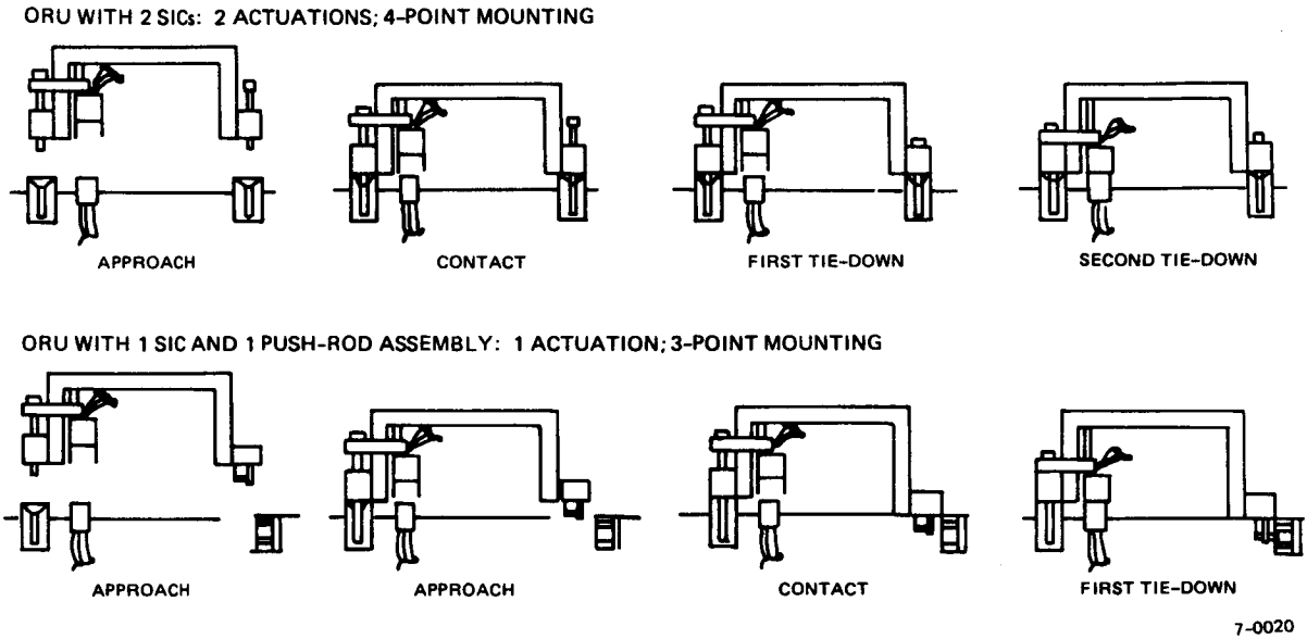
Figure 6. Attachment Procedure for Two Variations of the SIC Baseline
