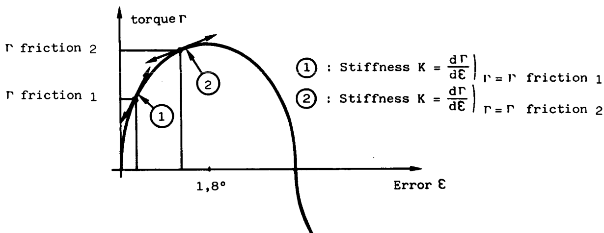
Schematic of Detent position motor torques
