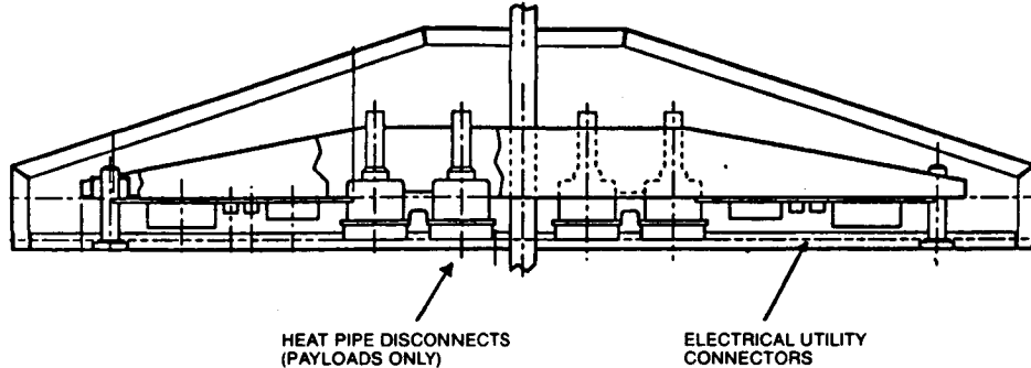
Figure 8. SIC Assembly with Heat Pipe Disconnects
