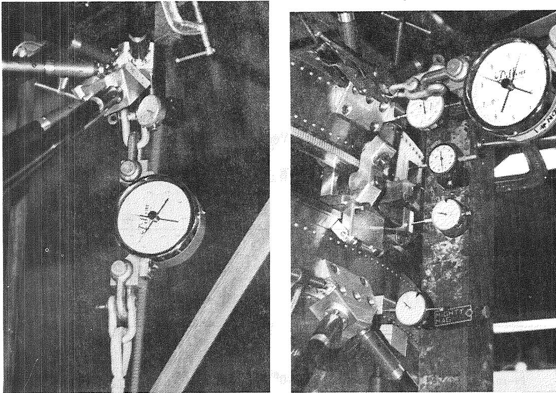
Figure 6: Bending, Shear Test Set-Ups
