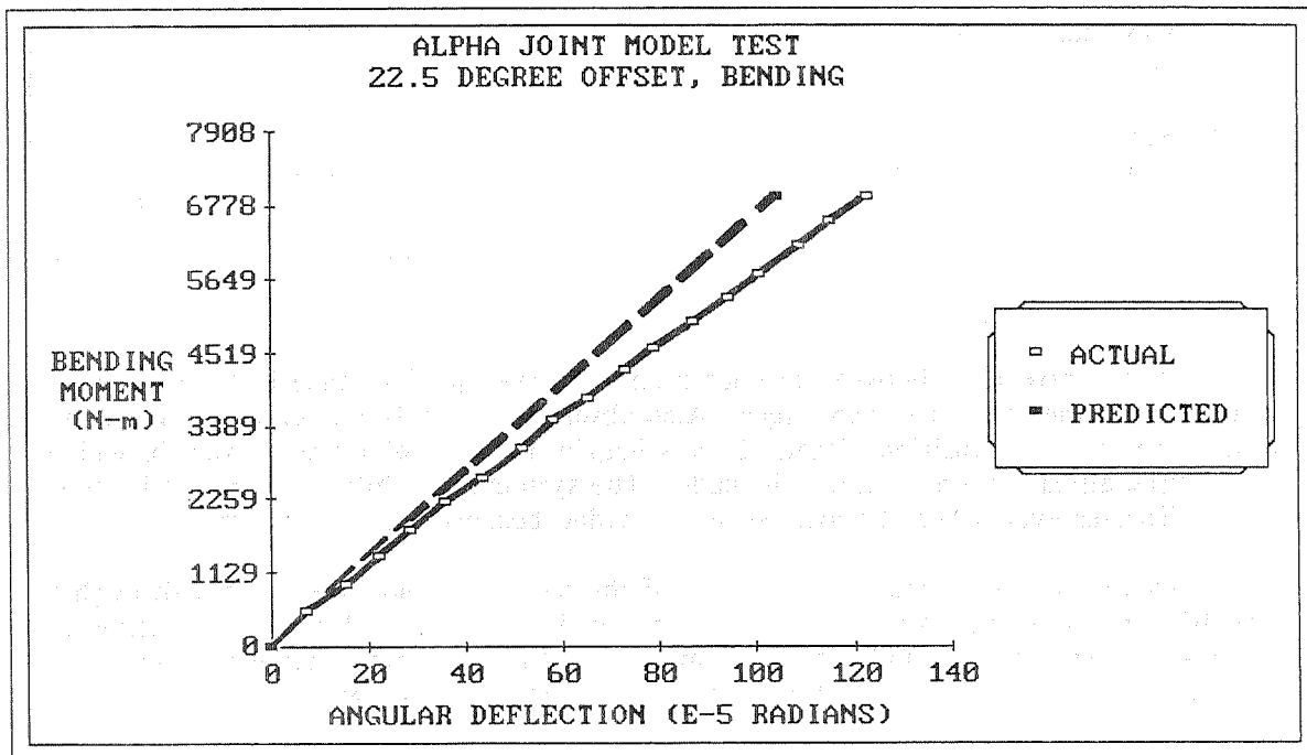
Figure 7: Bending Stiffness Test Results
