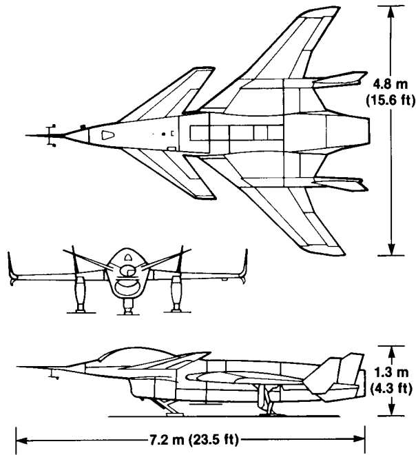
Figure 1. HiMAT remotely piloted research vehicle.
