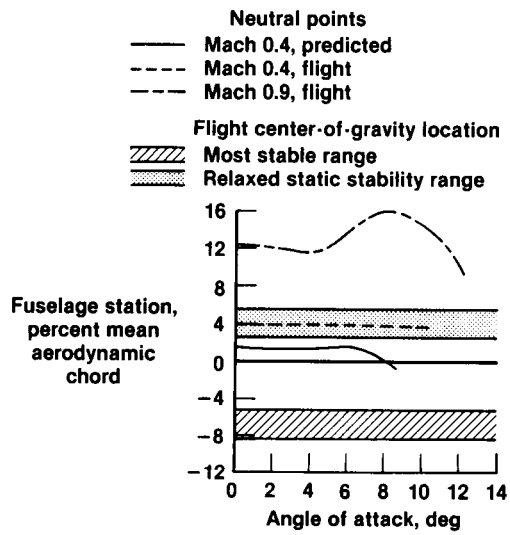
Figure 6. Neutral point and center-of-gravity ranges.
