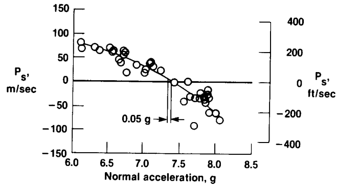
Figure 14. Flight-measured specific excess power.
