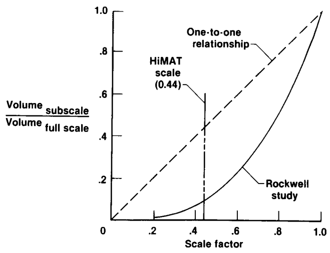
Figure 15. Vehicle volume ratio variation with scale factor.
