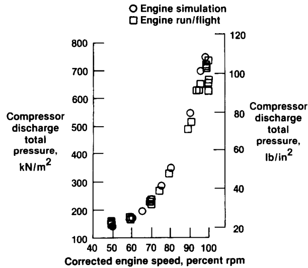
Figure 12. Digital propulsion control system performance for high-stability mode.
