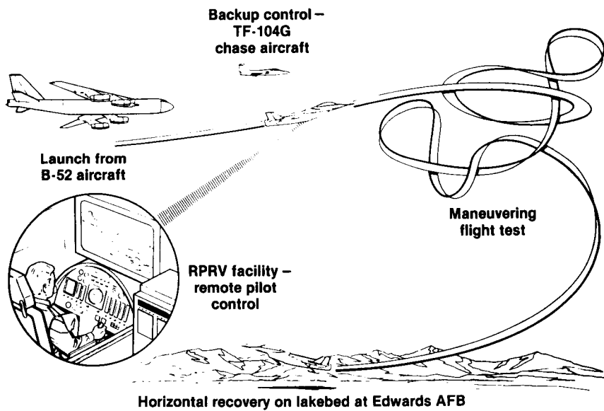
Figure 2. HiMAT operational concept.
