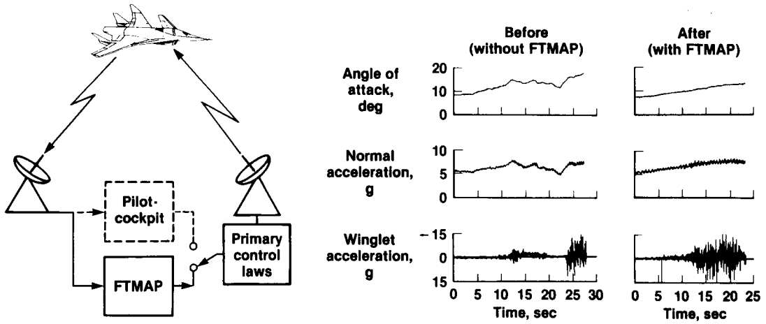
Figure 5. HiMAT flight test maneuver autopilot.
