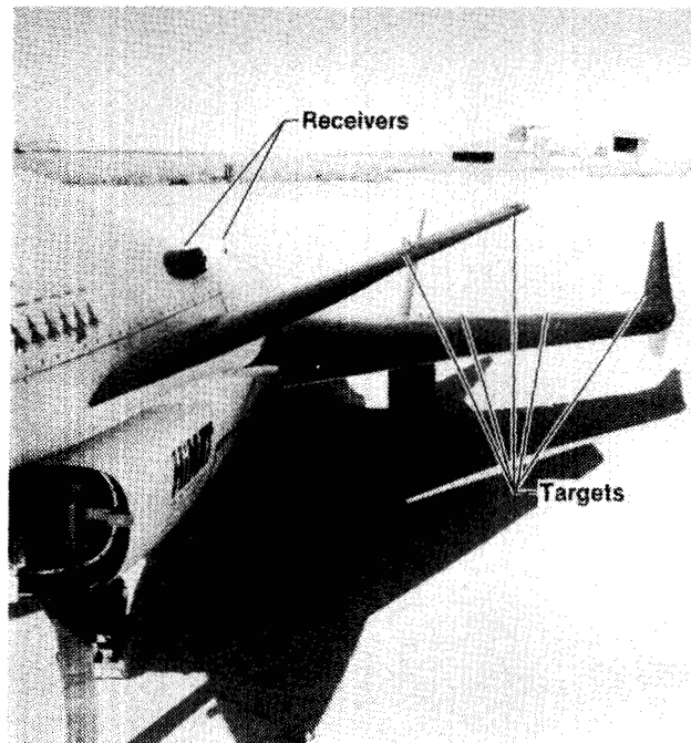
Figure 4. HiMAT flight deflection measurement system.
