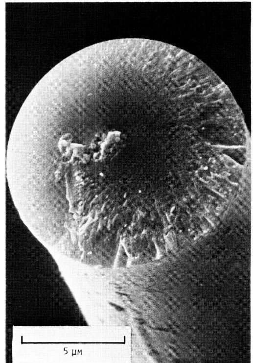
(C) FIBERS TREATED AT 10^{-8} ATM, WITH WT LOSS OF 0.8% AND TENSILE STRENGTH OF 154 KSI (1062 MPa).
