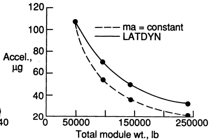
Variation of max module acceleration with module weight
