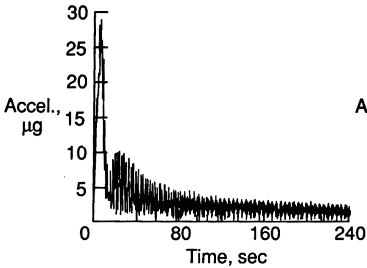
Typical module acceleration time history
