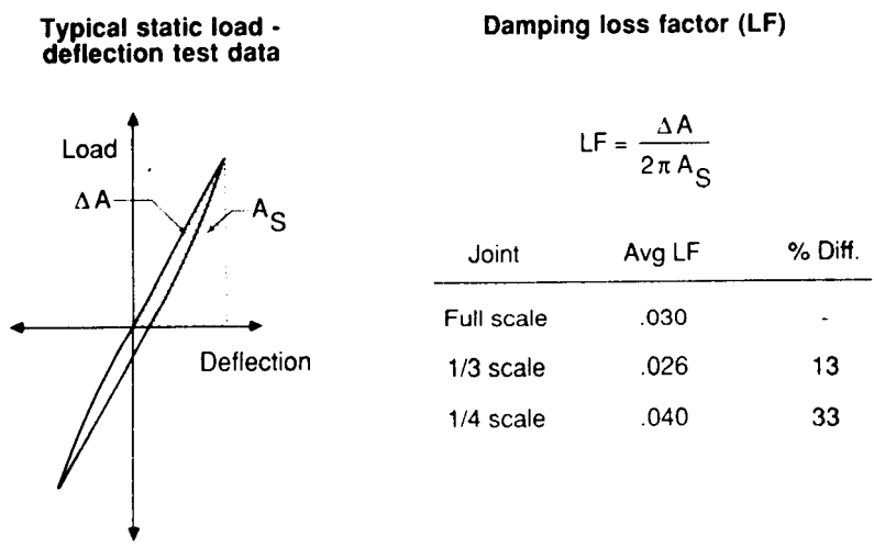
Fig. 16 Assessment of loss factors in scaled joints showing good correlation of scaled and full-scale test results.
