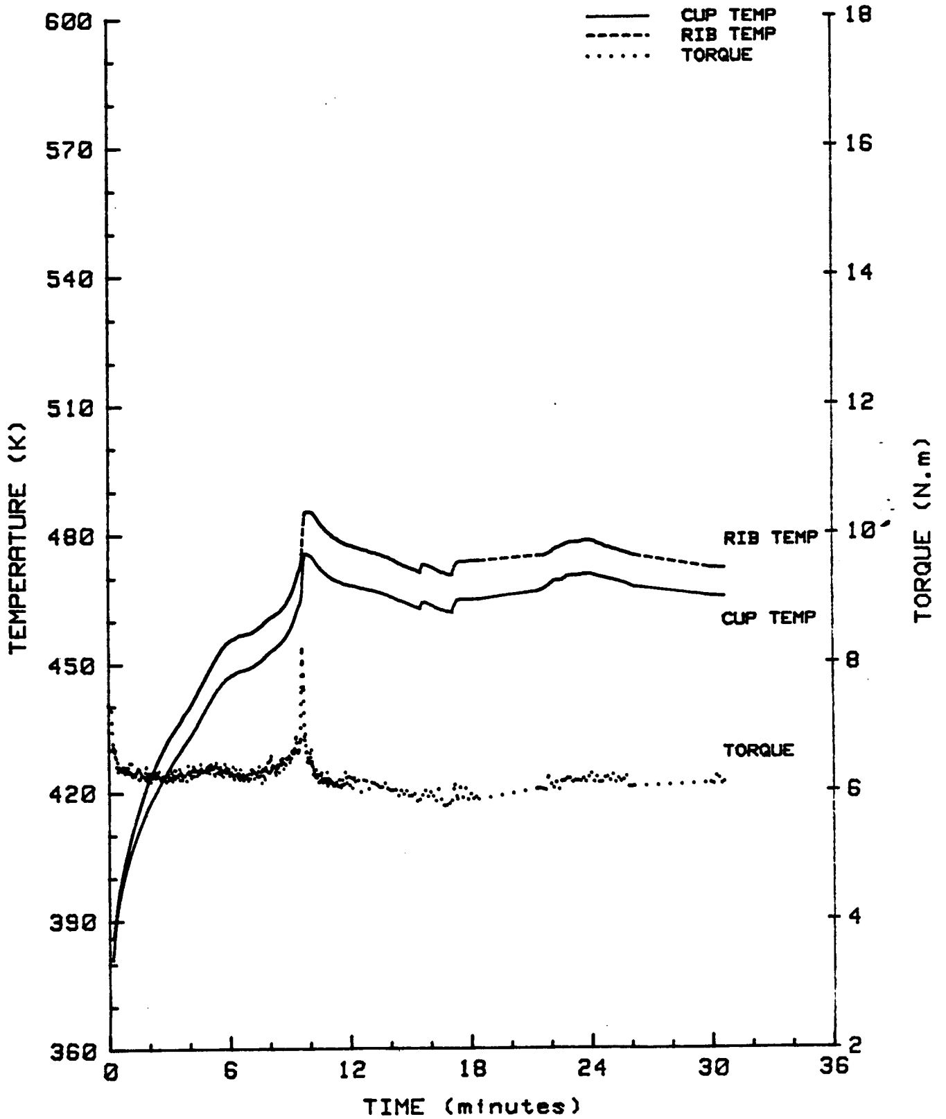
Figure 28. OIL-OFF TEMPERATURE and TORQUE vs TIME AT 11000 RPM. TSRC-S CBS1000M 65% DENSITY
