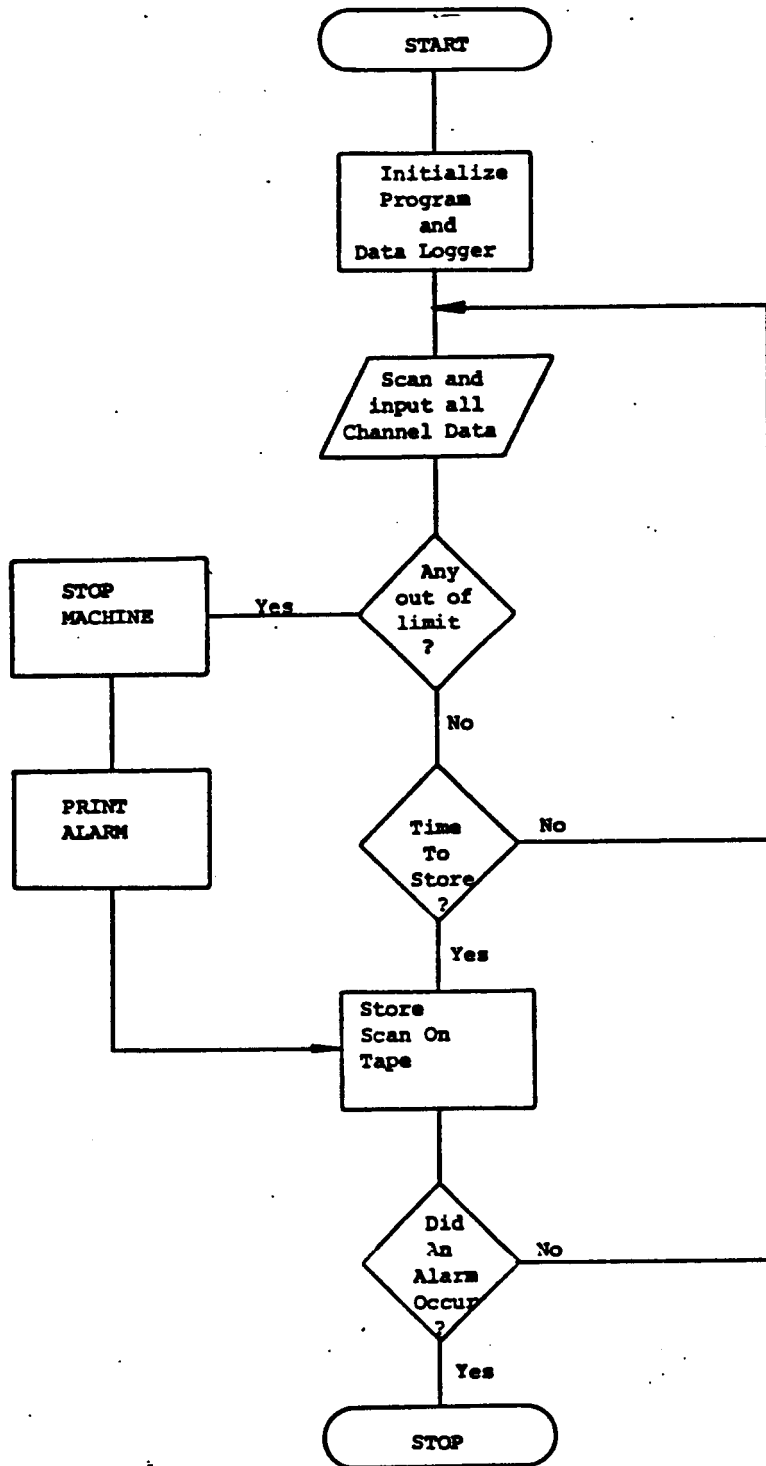
Figure 11 Data Acquisition Flow Chart
