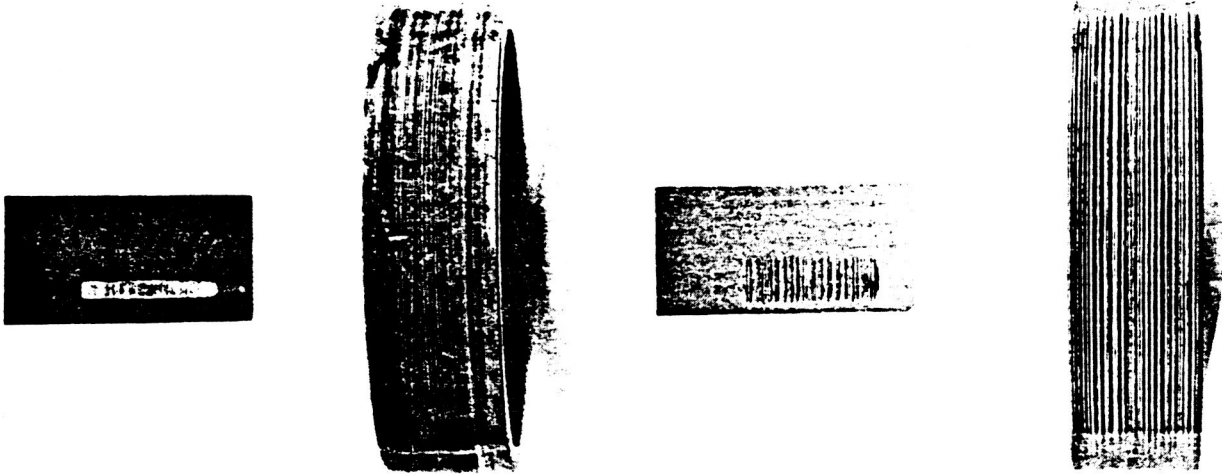
(b) Silicon Nitride Test Block and CBS 600 Ring
