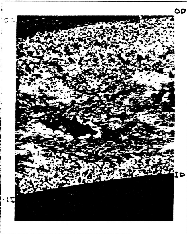
Rib No. 84-77 Damaged at 24000 rpm(1.6 million DN) (25X Magnification)
