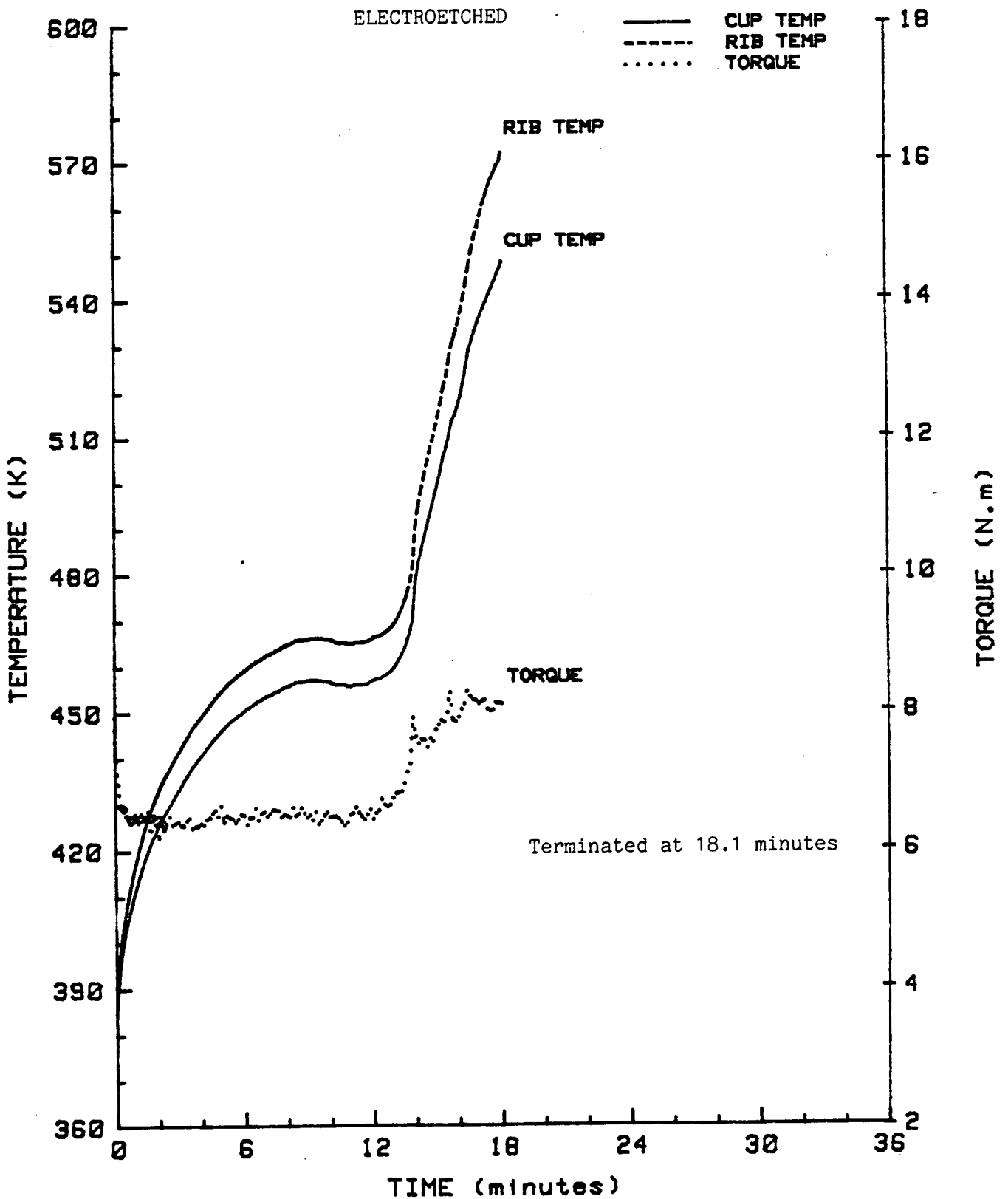
Figure 29. OIL-OFF TEMPERATURE and TORQUE vs TIME AT 12000 RPM. TSRC-S CBS1000M 65% DENSITY
