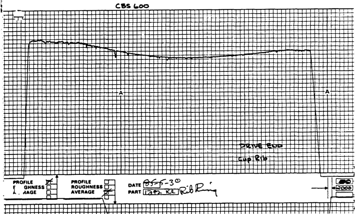
Figure 14 - JEX1292CE, TSRC, CBS600 Cup Rib Wear
