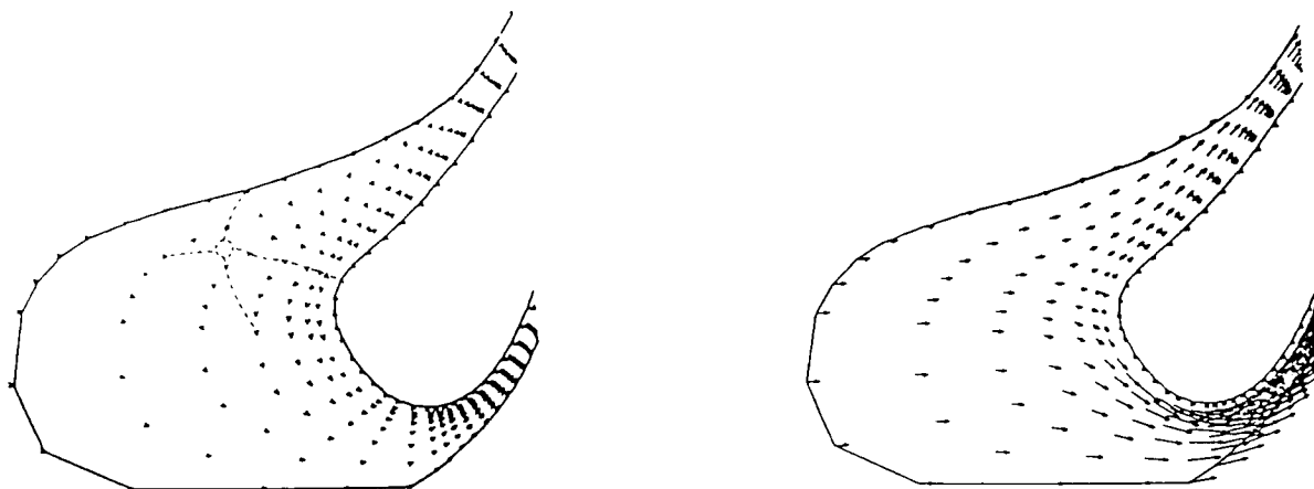
(b) VECTOR PLOT ON MIDSPAN PLANE
