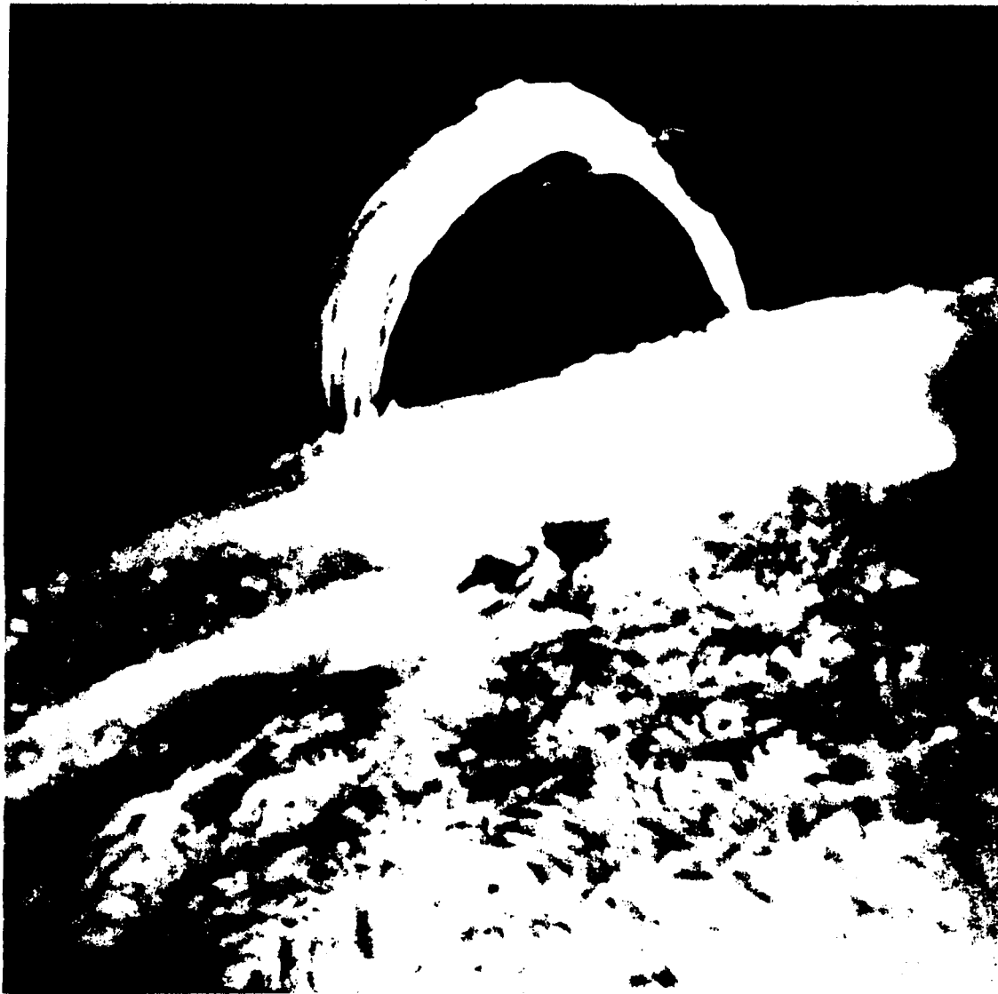
Fig. 11 Plots (a) of observed halfwidth against Balmer number for four different polarizer orientations, for the December 19, 1982, loop, shown in (b). The angle \theta = 45 corresponds roughly to E-field transverse to B-field at the loop apex.
