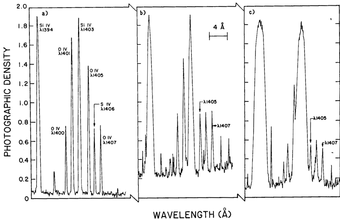
Fig. 5 - The O IV multiplet from Skylab S082-B spectra (Doschek 1984).
