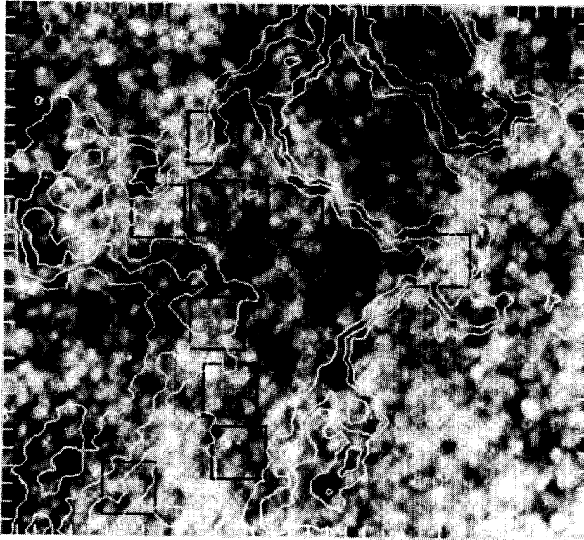
Fig. 5 Image of the pore region with magnetic contours overlaid. The contour levels are -75 and -270 gauss. The black boxes indicate regions used for constructing autocorrelation functions. Ticks are separated by one arc second.
