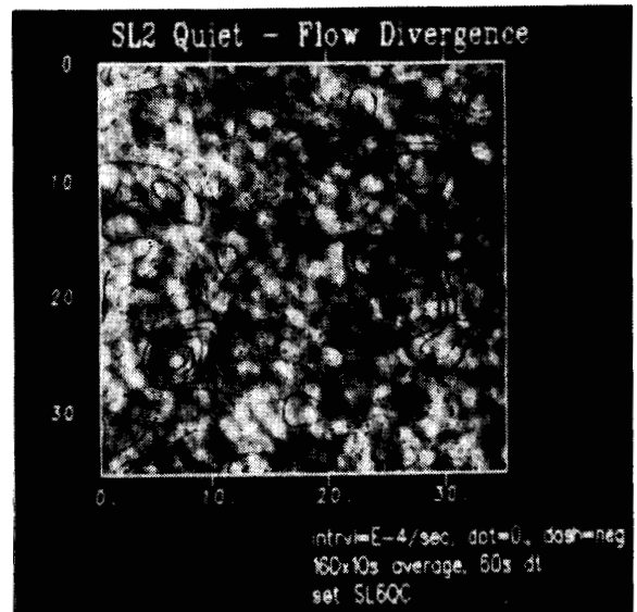
Figure 7. Divergence of quiet-region flows. The contours show the amplitude of the local divergence of the horizontal flows from Figure 1. The contour interval is 1 \cdot 10^{-4} \text{ s}^{-1} . Point source regions are those with positive divergence (solid contours), while the linear sink regions have negative divergence (dashed contours). The zero contour is dotted.
