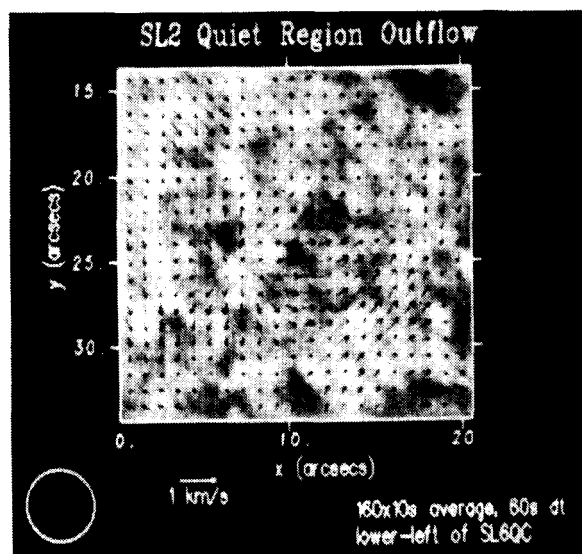
Figure 4. A magnified portion of the quiet proper-motion map from Figure 1 is magnified and more vectors are displayed. This demonstrates the cellular nature that is characteristic of the large-scale proper-motion flows.
