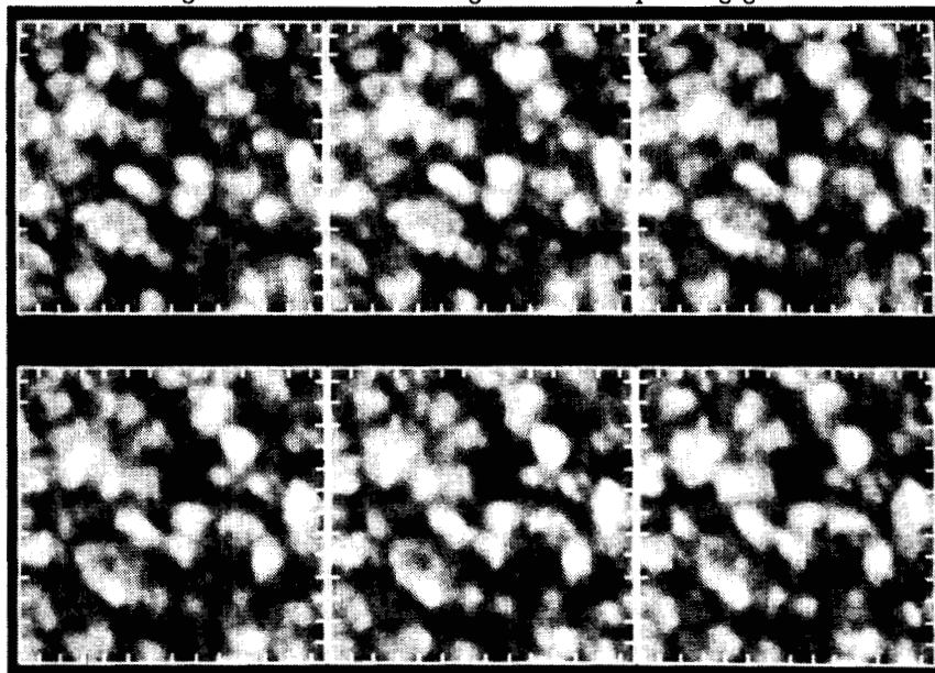
Fig. 20 Time sequence of images of region of elongated granules. Tick marks are at arc second intervals.
