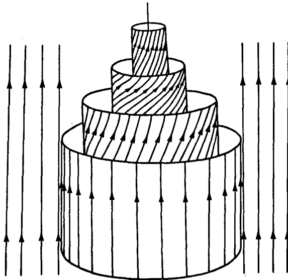
FIG. 2 A sketch of a twisted flux bundle extending uniformly from z=0 to z=L whose field fits smoothly and continuously onto the surrounding uniform field B_0 .
