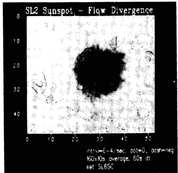
Figure 8. Divergence of sunspot-region flows shown in Figure 2.
