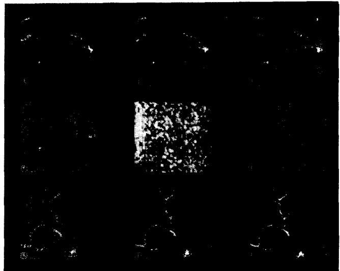
Figure 11. Propagation of long-lived tracers. "Corks" embedded in the flow field of Figure 1 trace out the flow pattern from their emergence in regions of positive divergence until they congregate in sinks and network regions where the divergence is negative. The nine frames proceed from -8 to +8 hours with the actual observation time (hour 0) shown as a superposed uniform grid of corks and granulation intensity in the center frame.
