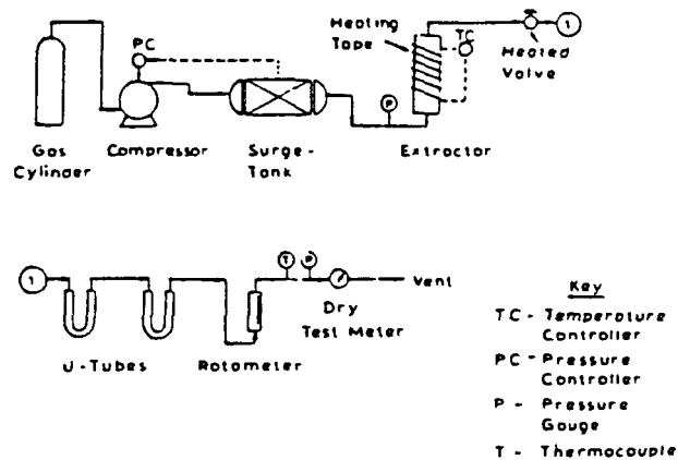
Fig. 2) Schematic diagram of experimental fluid extraction for supercritical fluid extraction (from /16/).
