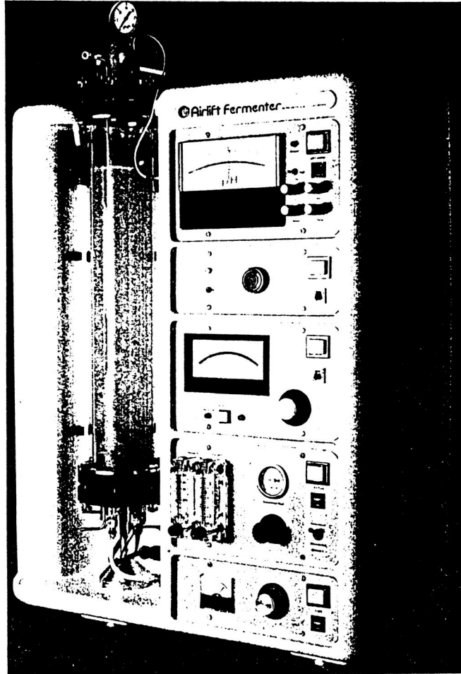
Fig.2 A 21 Bethesda Research Laboratory Air-Lift fermentor.
