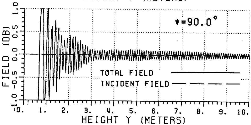
Figure 136: Normalized magnitude of total fields from finite symmetrical slabs with different wedge angles (3 GHz).
