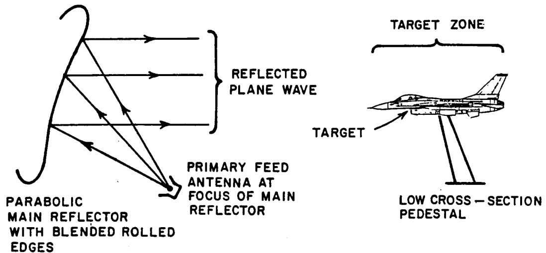
Figure 1: Typical focus-fed compact range configuration.
