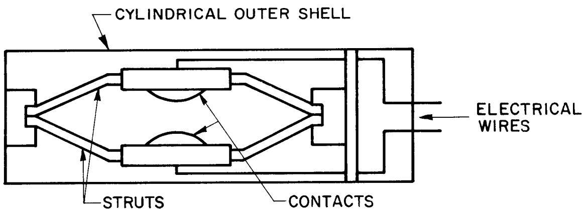
Figure 7. - Rate-compensation detector.
