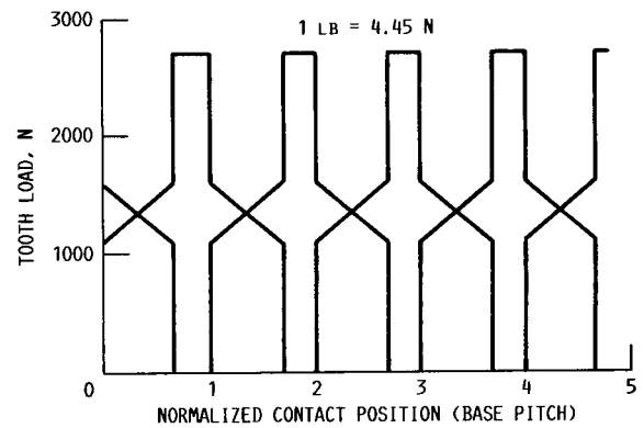
FIGURE 8. - TYPICAL STIFFNESS AND LOAD SHARING OF LOW CONTACT RATIO GEARS OF FIGURE 4(A).
