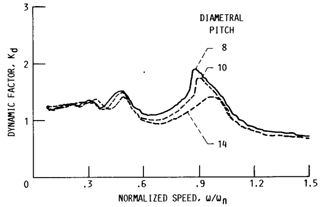
FIGURE 11. - EFFECT OF DIAMETRAL PITCH ON DYNAMIC RESPONSE.
