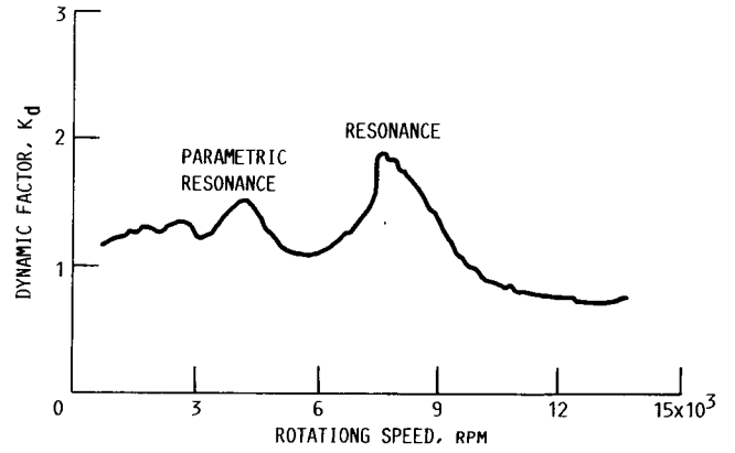
FIGURE 4. - DYNAMIC FACTOR AS A FUNCTION OF ROTATING SPEED.
