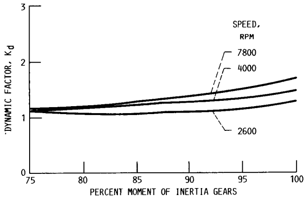
FIGURE 10. - EFFECT OF GEAR INERTIA ON DYNAMIC ON DYNAMIC RESPONSE. (GEAR INERTIA: 100% VALUE = 3.33 \times 10^{-3} KG-M 2 ).
