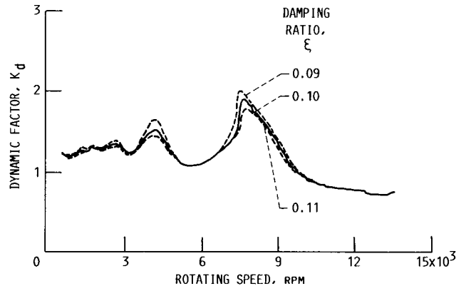
FIGURE 8. - EFFECT OF DAMPING ON DYNAMIC RESPONSE.
