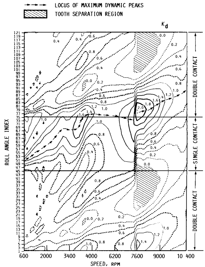
FIGURE 6. - CONTOUR PLOT OF SYSTEM DYNAMIC RESPONSE.
