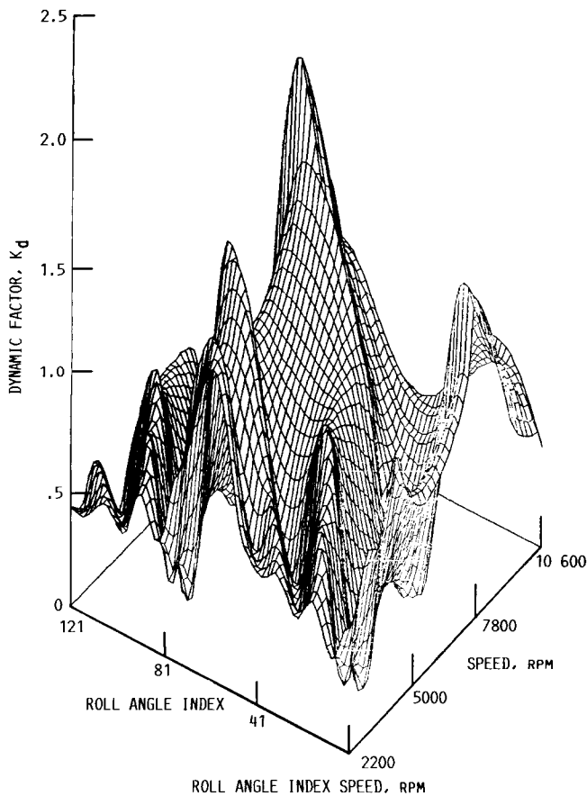
FIGURE 5. - SYSTEM DYNAMIC RESPONSE.
