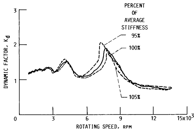
FIGURE 9. - EFFECT OF AVERAGE TOOTH STIFFNESS ON DYNAMIC RESPONSE. AVERAGE TOOTH STIFFNESS: 100% VALUE = 3.991 \times 10^5 N-M/RAD.
