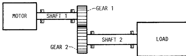
FIGURE 1. - A SIMPLE SPUR GEAR SYSTEM.
