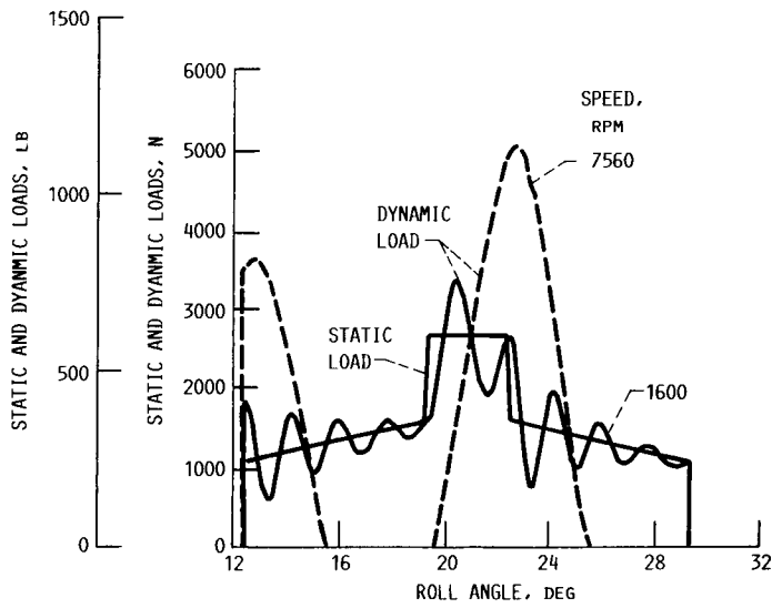
FIGURE 3. - DYNAMIC LOADS AT DIFFERENT SPEEDS FOR IDENTICAL YEARS. MODULE = 3.18 MM; PRESSURE ANGLE = 20°; PITCH RADIUS = 57.1 MM; APPLIED LOAD = 2760 N (600 LB).
