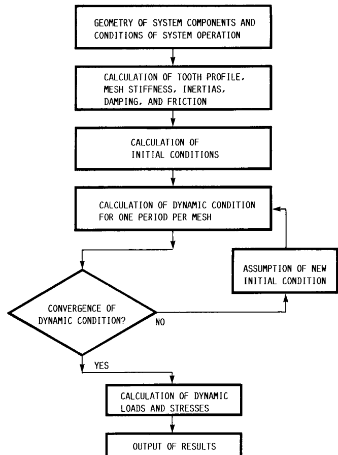
FIGURE 2. - FLOW CHART OF COMPUTATIONAL PROCEDURE.
