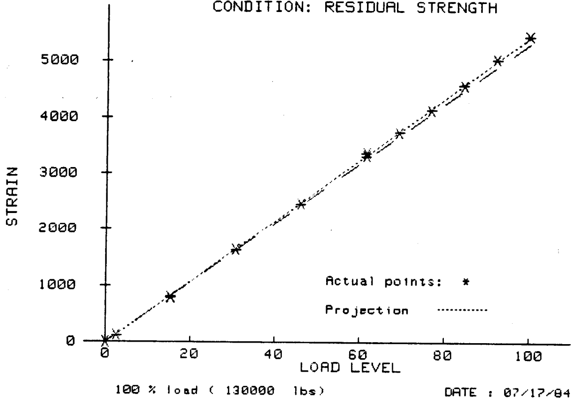
Figure H-18. CV2-2 Residual Strength Tension Test - Strain Gauge Readings - Plot Gage 18
