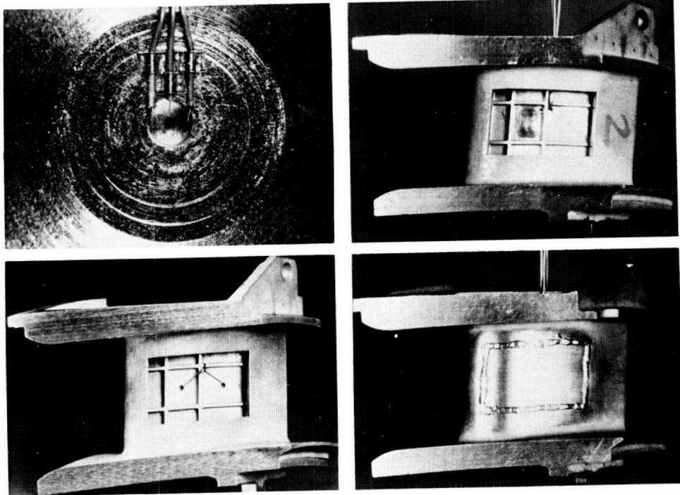
FIGURE 3. - HEAT FLUX SENSORS INSTALLED IN TURBINE VANE.
