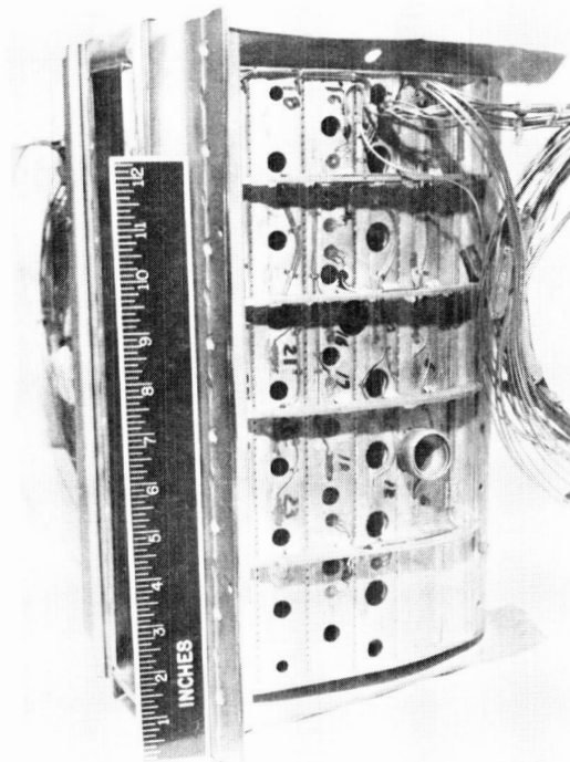
FIGURE 4. - COMBUSTOR SEGMENT INSTRUMENTED WITH HEAT FLUX SENSORS.
