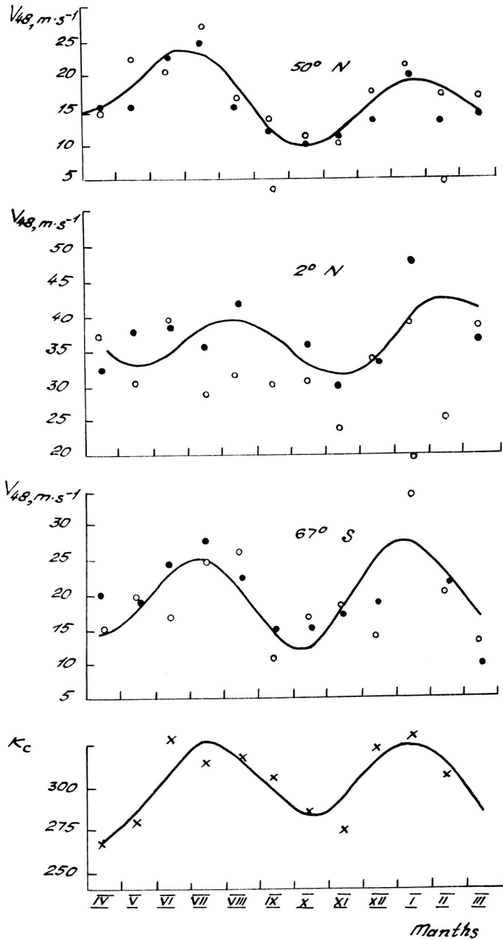
Fig. 3 Average maximum monthly amplitude of the two day wave from data measured at 95 km from Obninsk ( 50^{\circ}N , 1970-76), Mogadishu ( 2^{\circ}N , 1968-70) and Molodezhnaya ( 67^{\circ}S , 1972-74), meridional \bullet , zonal \circ ; note the obvious correlation with K_c .
