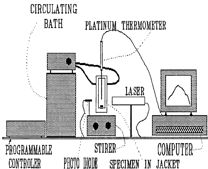
Figure 6. Apparatus for determination of phase diagrams of the transparent model monotectic alloy.
