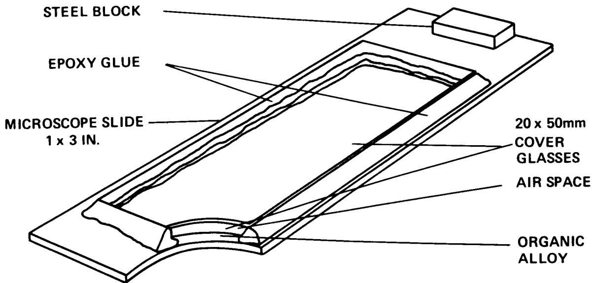
Figure 3. Sample cell for transparent alloy study.
