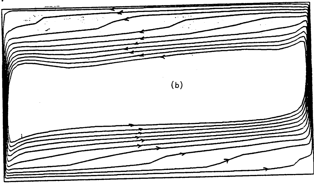
Figure 7. Steady-state velocity vectors (a), stream lines (b) and iso-concentrations for Case 2
