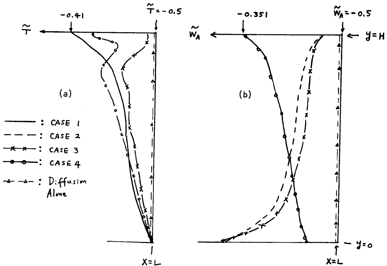
Figure 16. Temperature and mass concentration profiles along the vertical coordinate at the control volumes next to the right vertical surface
